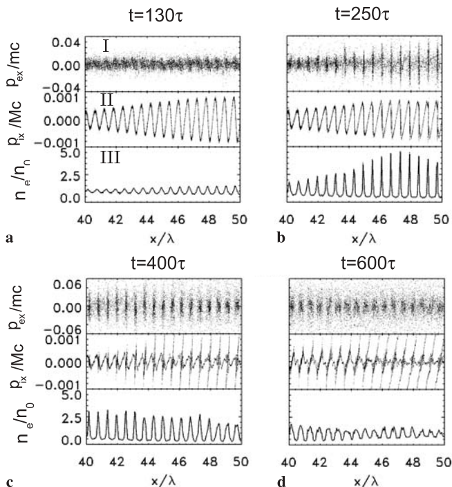
FIGURE 3 Snapshots of the longitudinal components of electron (frame I) and ion (frame II) momenta as well as the electron (in solid lines) and ion (in dotted lines) densities (frame III) at different times. The parameters for the plasma and laser pulses are the same as in Fig. 2. Note that one cannot distinguish the distribution of the ion density from that of the electron density plotted in this scale, indicating that a quasi-charge-neutrality state is achieved at these times
