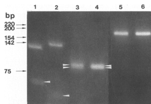
Fig. 2. Restriction analysis of the 170-bp Y-chromosome-specific fragment. Lane 1 DdeI digestion, lane 2 HinfI digestion, lane 3 HpaII digestion, lane 4 NciI digestion, lane 5 EcoRI digestion, lane 6 undigested 170-bp fragment. Positions of size markers shown on the left
