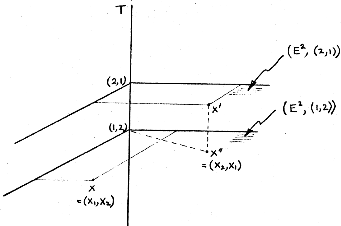
Fig. 6.1: Example of Y \times T where Y = E^2 , T = \{(1,2), (2,1)\}
