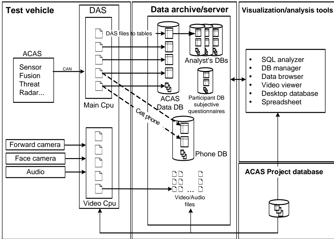
Figure 4.1. Overview of the ACAS data handling paths
