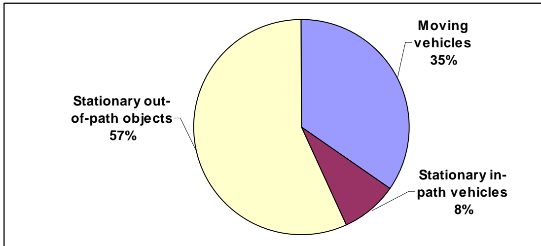
Figure 6.82. Breakdown of ACC alerts by target type
