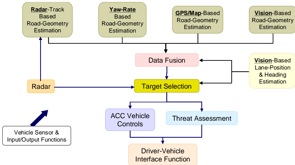
Figure 3.2. ACAS functional schematic
