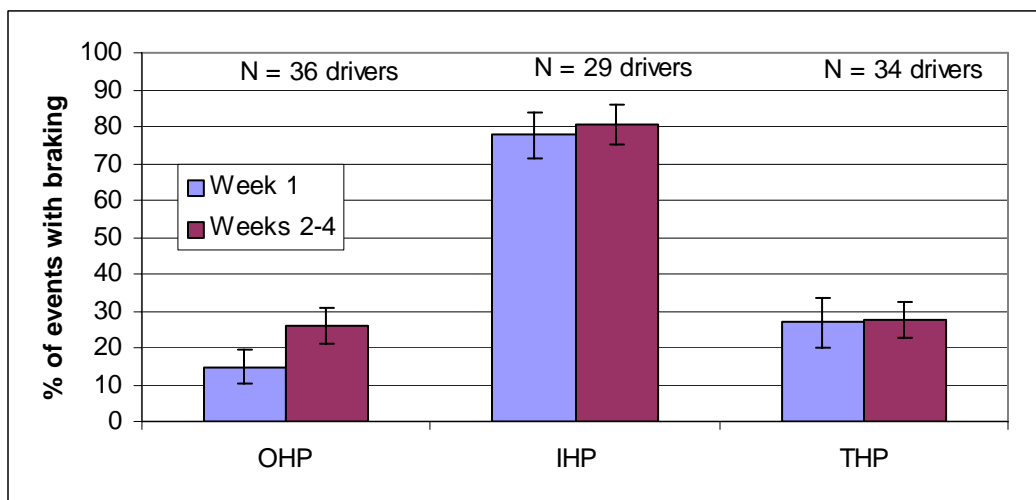
Figure 7.21. Mean fraction of FCW alert events with driver braking. Error bars represent standard error of the means.
