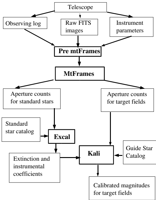
Fig. 3 A flowchart of MTPipe.
