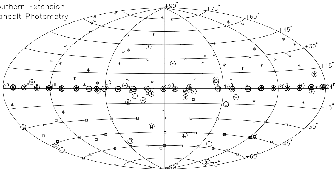
Fig. 1 Locations of the 158 Smith et al. (2002) primary standards (asterisks) and the 64 fields of the southern extension to the primary standard star network (unfilled squares; see Sect. 5). Circled symbols indicate u'g'r'i'z' standard stars or fields for which there is currently Landolt UBVR_cI_c photometry (Landolt 1973, 1983, 1992) or for which Landolt is currently obtaining UBVR_cI_c photometry (Landolt, in prep.).
