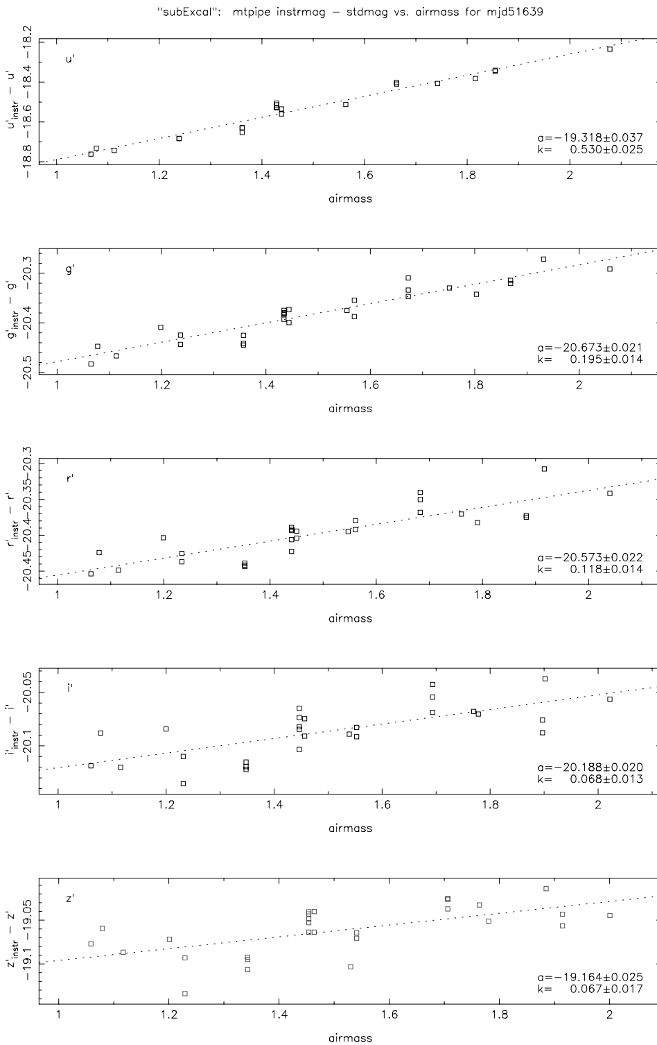
Fig. 15 "subExcal" results for photometric zeropoints ( a terms) and first-order extinctions ( k terms) for the PT data from the night of MJD 51639. The dotted line in each panel shows the best fit line to the data. The values for the slope ( k ) and zeropoint ( a ) of the best fit line is shown in each panel's legend.
