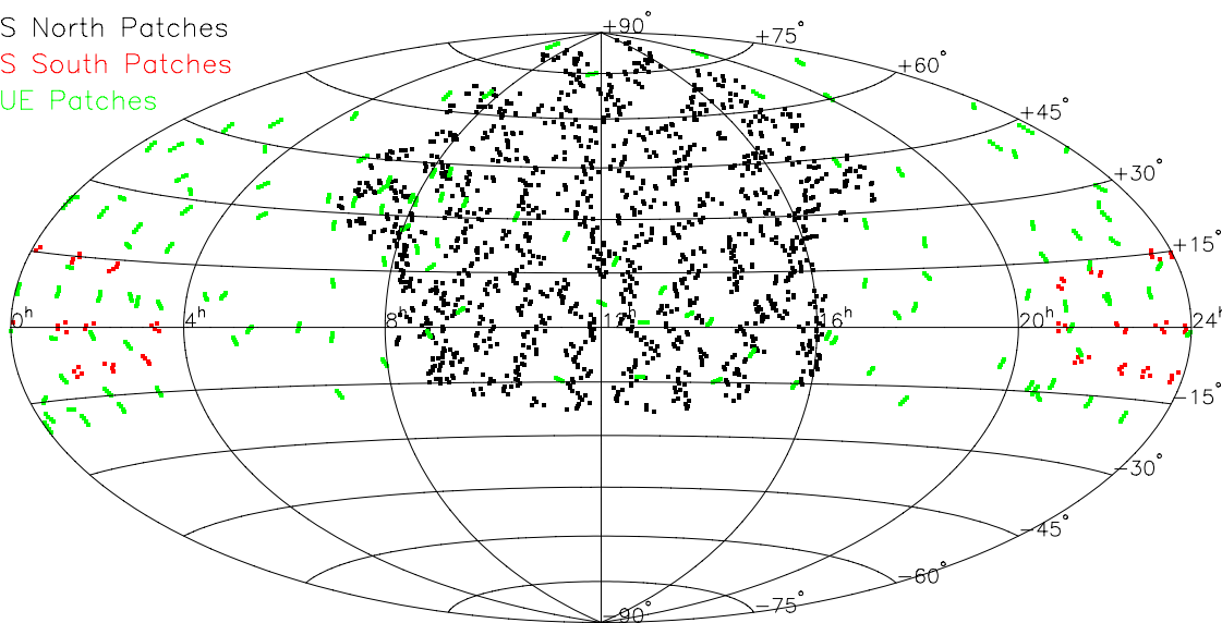
Fig. 2 Locations of the SDSS secondary patches in equatorial coordinates (Aitoff projection): (black) Northern SDSS patches, (red) Southern SDSS patches, and (green) SEGUE patches. (SEGUE is part of the Sloan extension, or SDSS-II, and is discussed in Sect. 5.)
