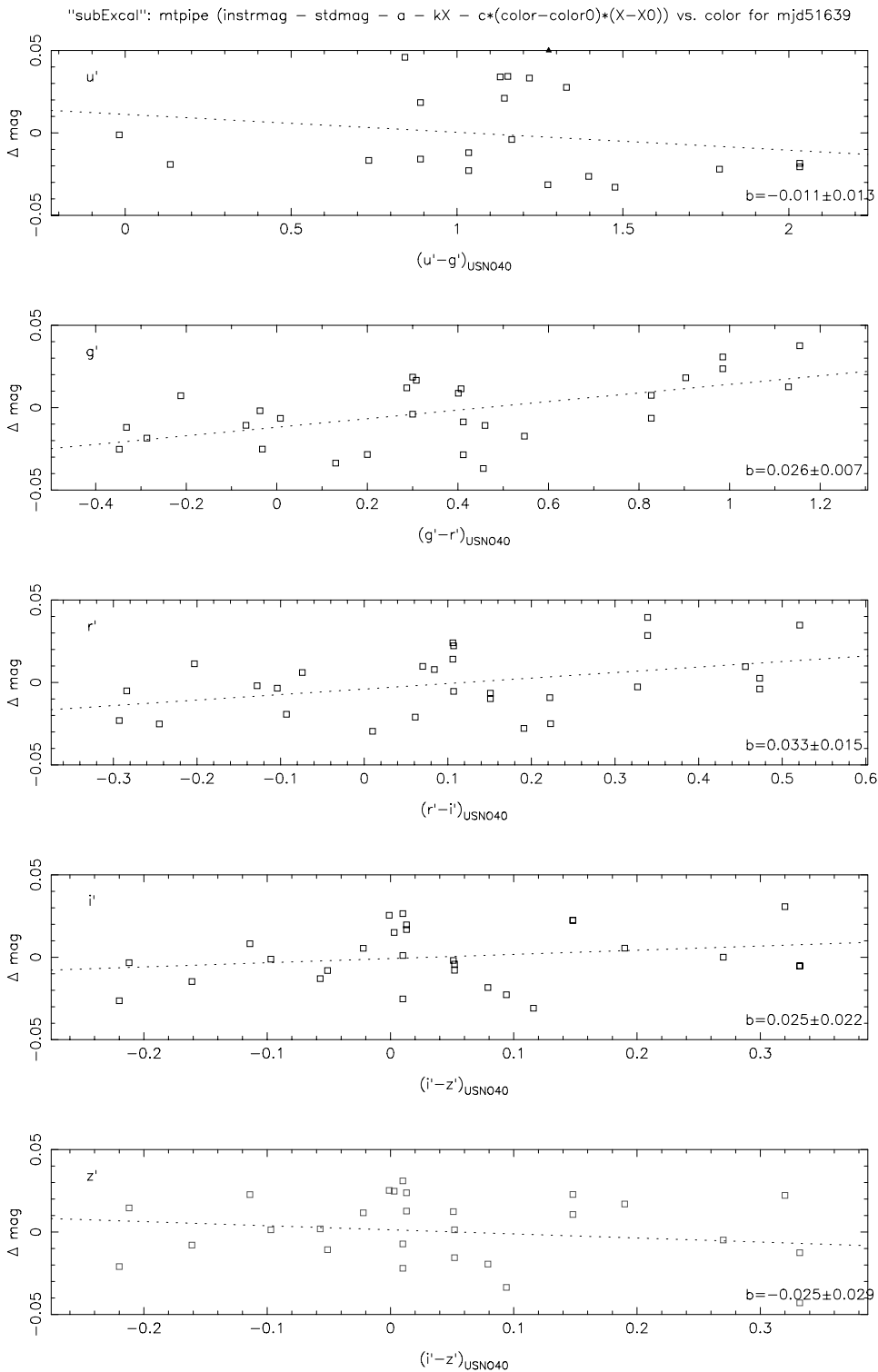
Fig. 16 “subExcal” results for instrumental color ( b ) term coefficients for the PT data from the night of MJD 51639. The dotted line in each panel shows the best fit line to the data. The value for the slope ( b ) of the best fit line is shown in each panel’s legend.
