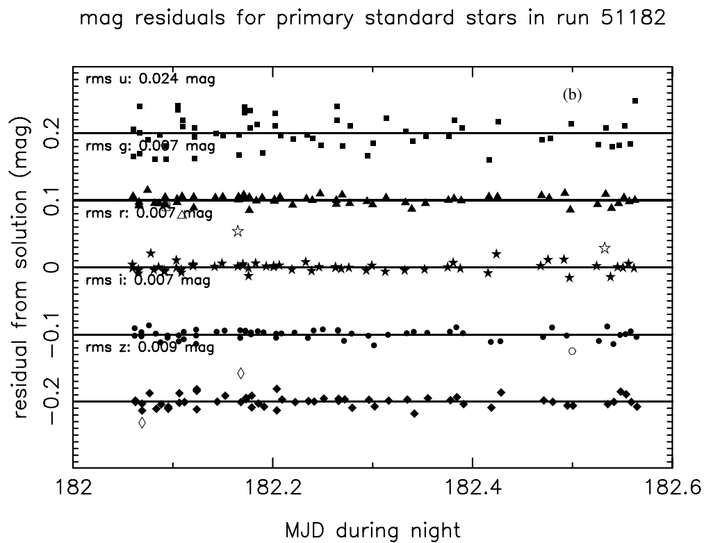
Fig. 9 The same excal quality assurance plots as in Fig. 8, but for the USNO-1.0m data taken on the night of MJD 51182, in which the k terms were solved for in 3-hour time blocks.
