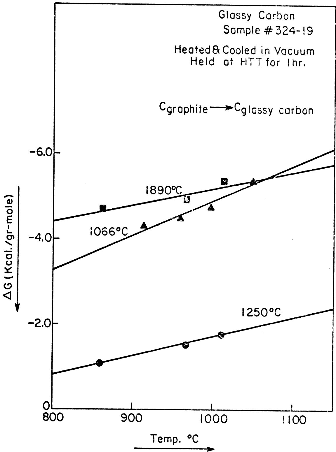
Figure 1. Free Energy-Temperature Relationship for 324-19 Series Glassy Carbons
