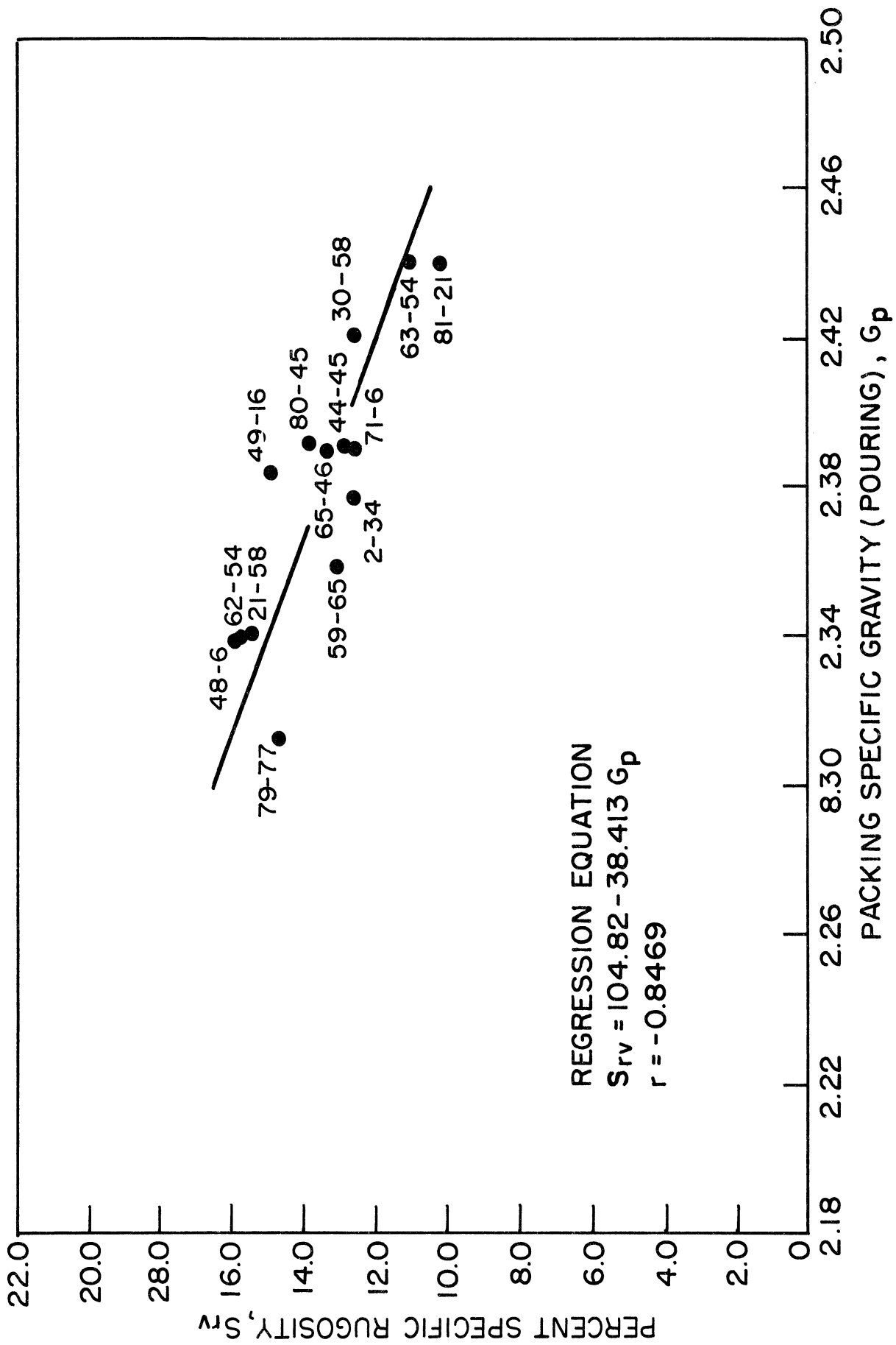
Figure 20. Specific rugosity vs. packing specific gravity (pouring) for 1/2 in.-5/8 in. fractions.
