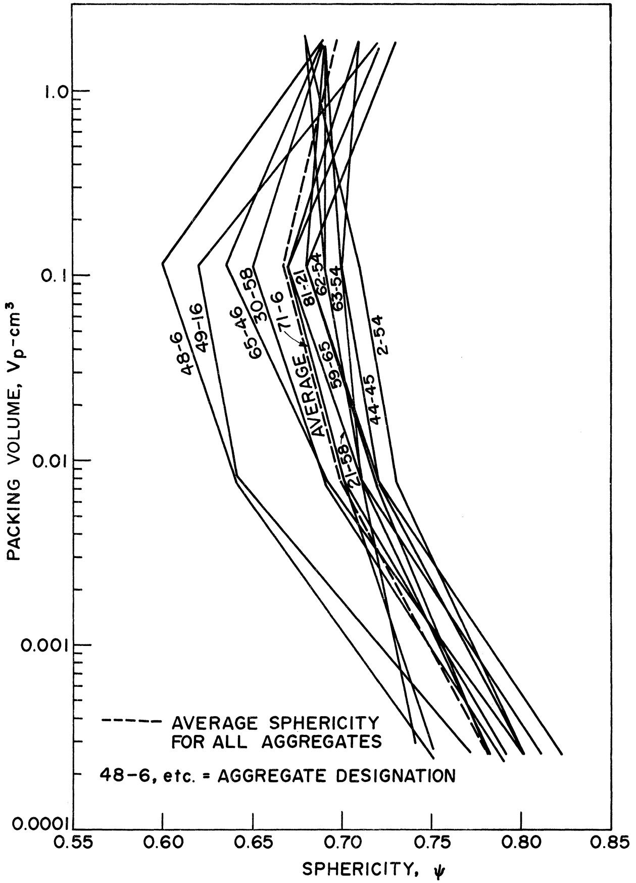
Figure 11. Relationship between packing volume and sphericity for different types of aggregates.
