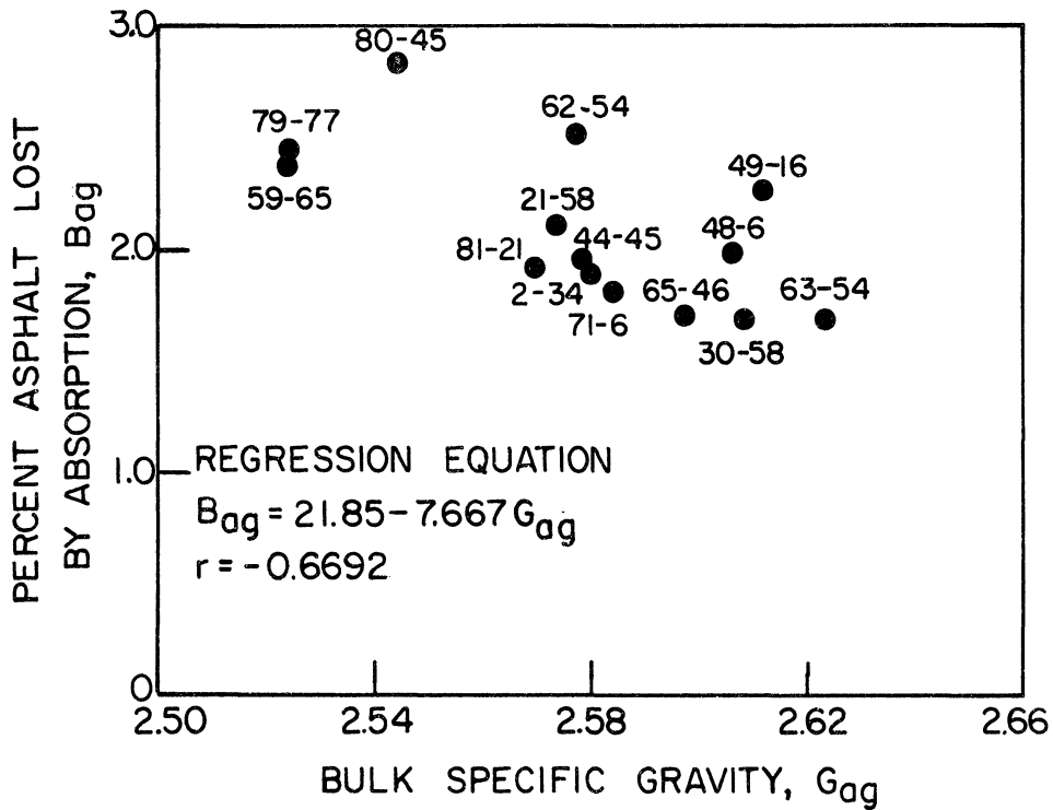
Figure 25. Asphalt lost by absorption vs. bulk specific gravity for #3-#4 fractions.
