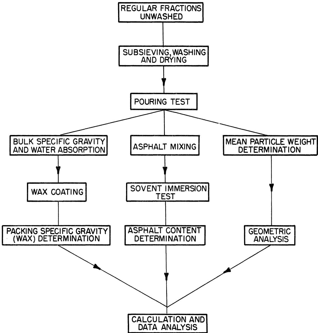
Figure 8. Method and order of testing program for each size of fractions. Flow chart.
