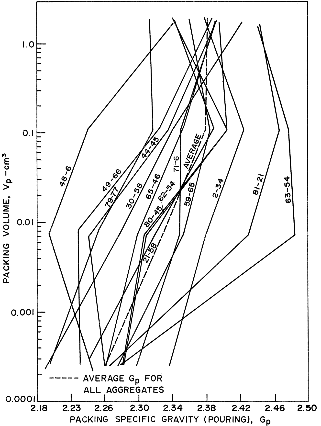
Figure 14. Relationship between packing volume and packing specific gravity (pouring) for different types of aggregates.
