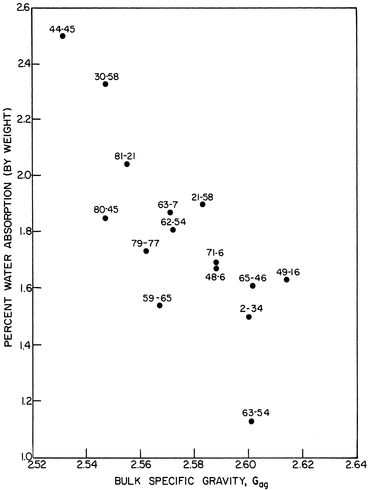
Figure 5. Relationship between water absorption and bulk specific gravity for graded aggregate blends (fines: -#4).
