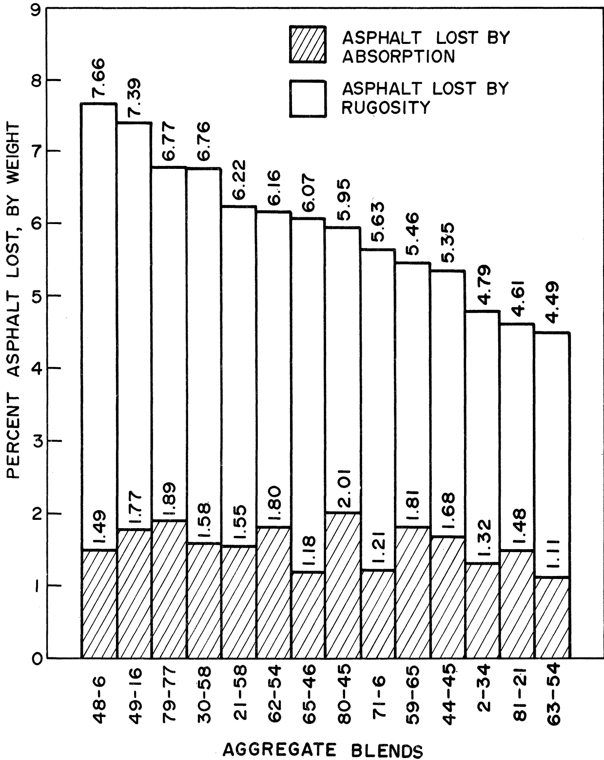
Figure 15. Average asphalt lost by rugosity and asphalt lost by absorption for different types of aggregates.
