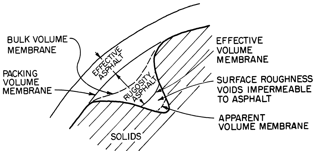
Figure 2. Rugosity asphalt in a surface pore.
