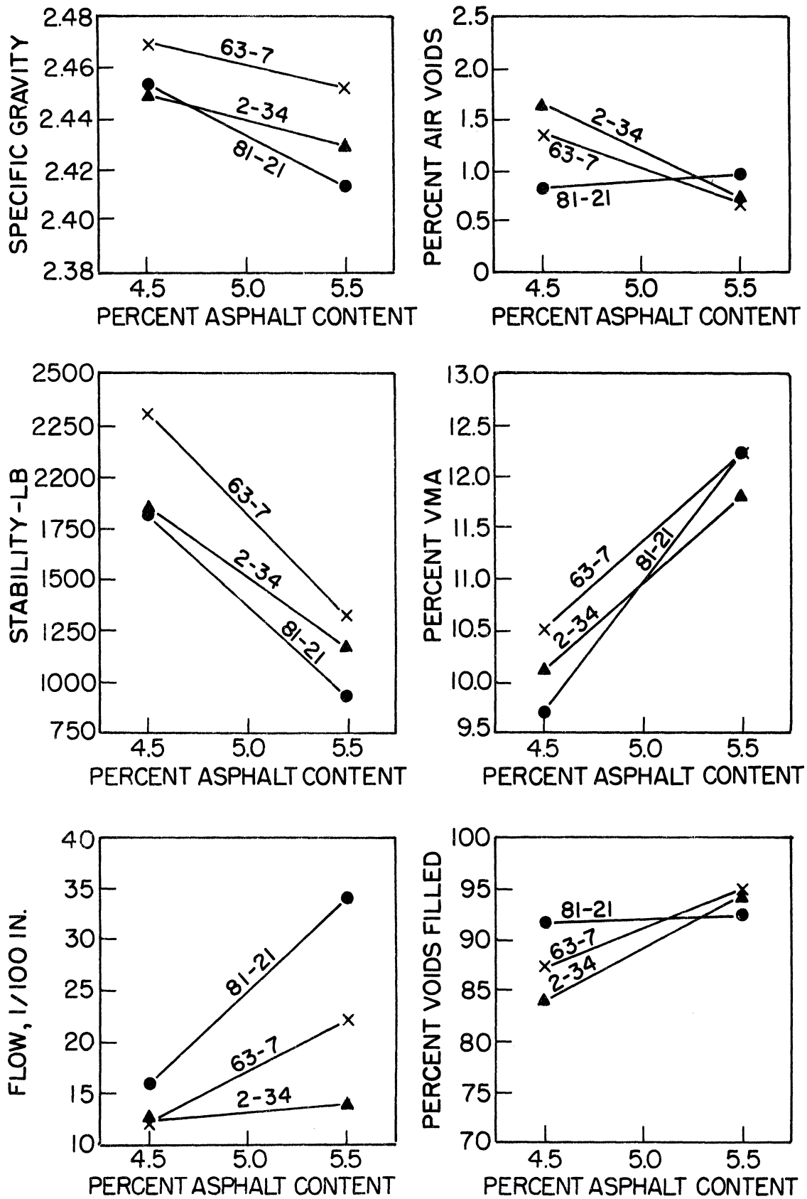
Figure 7. Marshall data for mixtures 81-21, 63-7, and 2-34 (unwashed).
