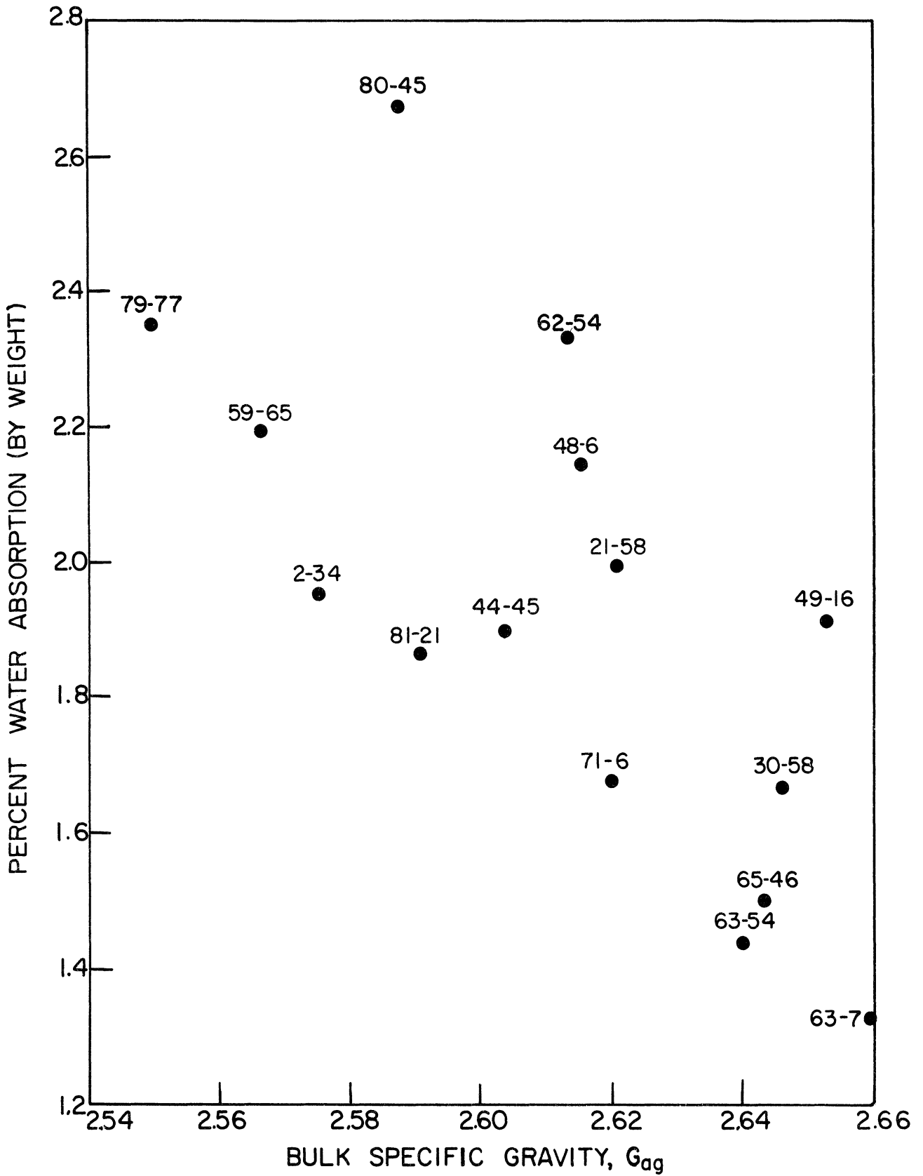
Figure 6. Relationship between water absorption and bulk specific gravity for graded aggregate blends (coarse: #4-3/4 in.).
