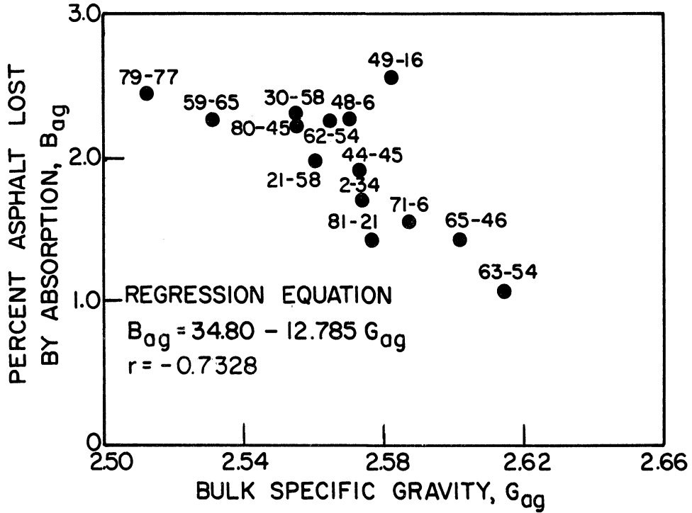
Figure 26. Asphalt lost by absorption vs. bulk specific gravity for #8-#10 fractions.
