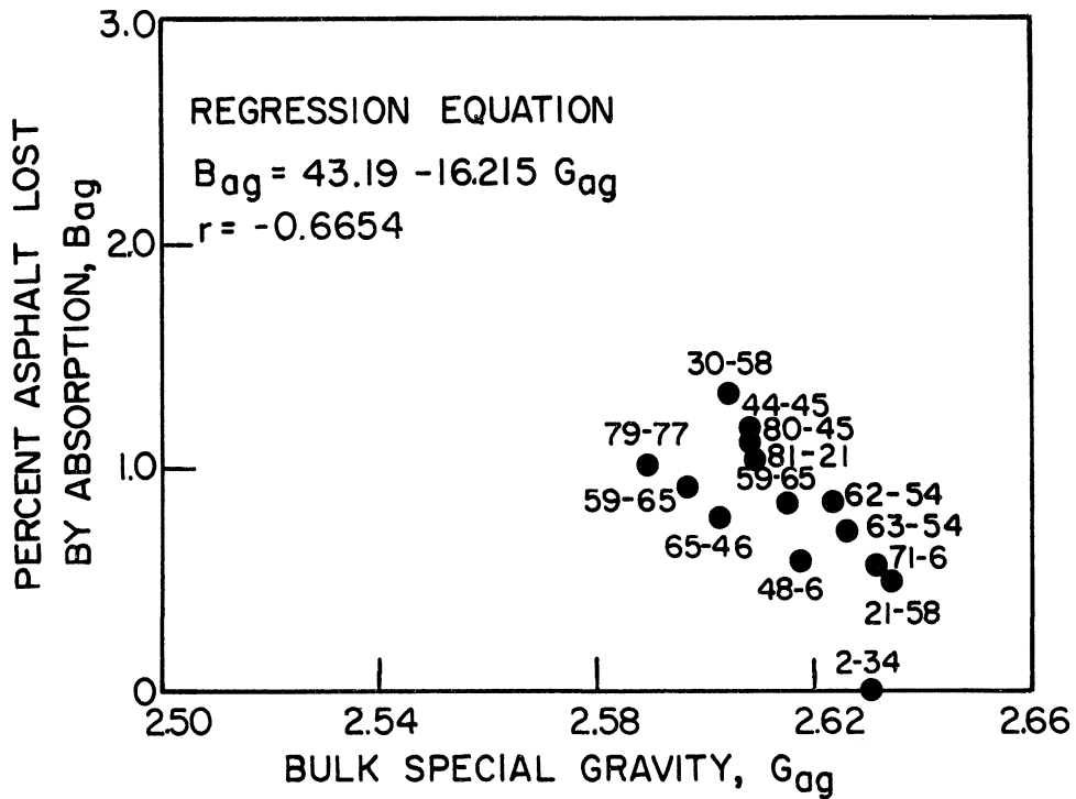
Figure 27. Asphalt lost by absorption vs. bulk specific gravity for #20-#30 fractions.
