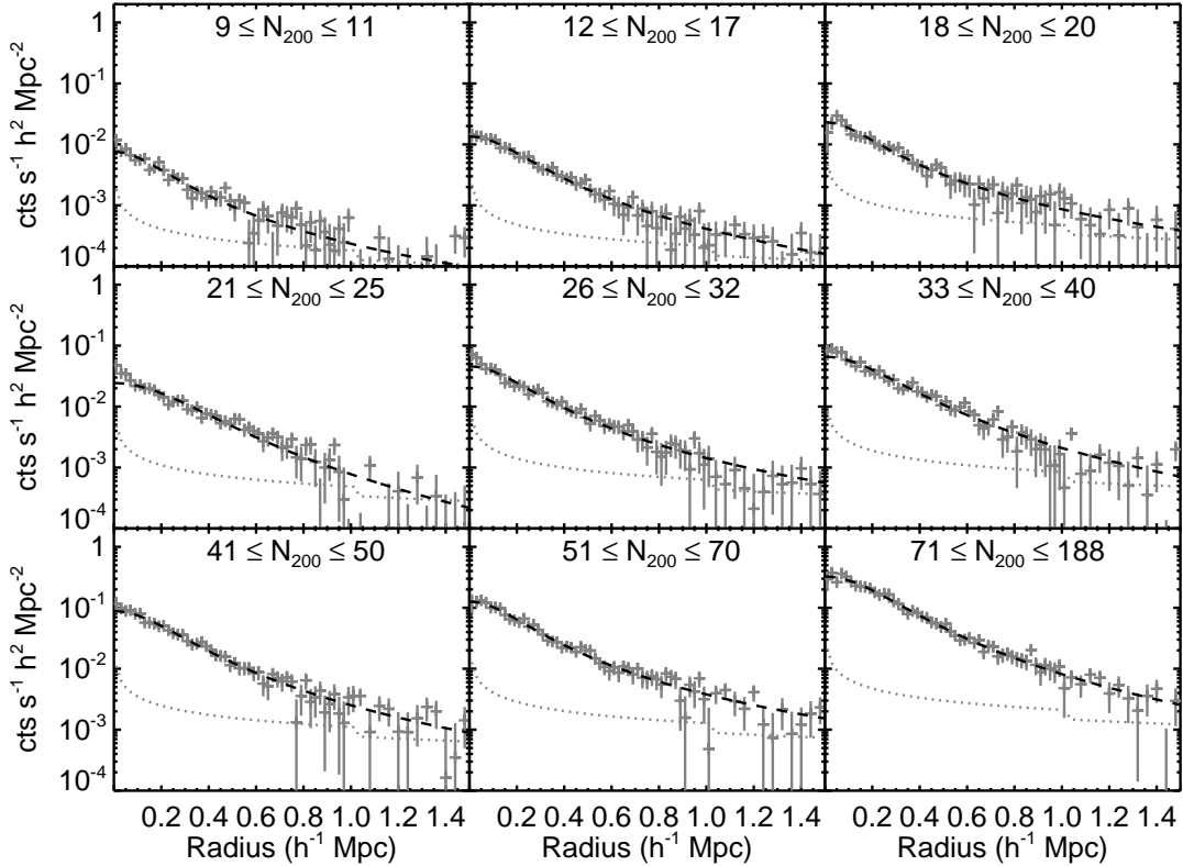
FIG. 2.— The background-subtracted surface-brightness profiles for the stacked images in each richness bin. The radial profiles have been summed in 50 h^{-1} \text{ kpc} ( 100 h^{-1} \text{ kpc} ) bins inside (outside) 1 h^{-1} \text{ Mpc} . For reference, the dotted lines represent the 1\sigma background limit. Significant cluster emission is seen in each richness bin. For the richest bins, this extends out beyond 1 h^{-1} \text{ Mpc} . The dashed lines show the \beta model fits from Table 2.
