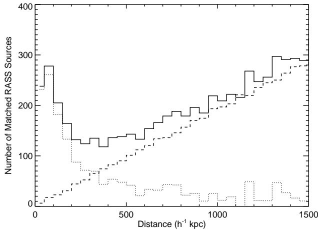
FIG. 4.— Histogram of offset distribution between maxBCG clusters and X-ray sources detected in the BSC and FSC catalogs. Each cluster is allowed to match to multiple X-ray sources, ensuring we find all associated X-ray sources in addition to all random matches. The solid (dashed) line shows the histogram of maxBCG (random) offsets in 50 h^{-1} kpc bins. The dotted line shows the result of subtracting the random matches from the cluster matches. There is a tight core in which the BCG is within \sim 150 h^{-1} kpc of an X-ray source, as well as a long tail.
