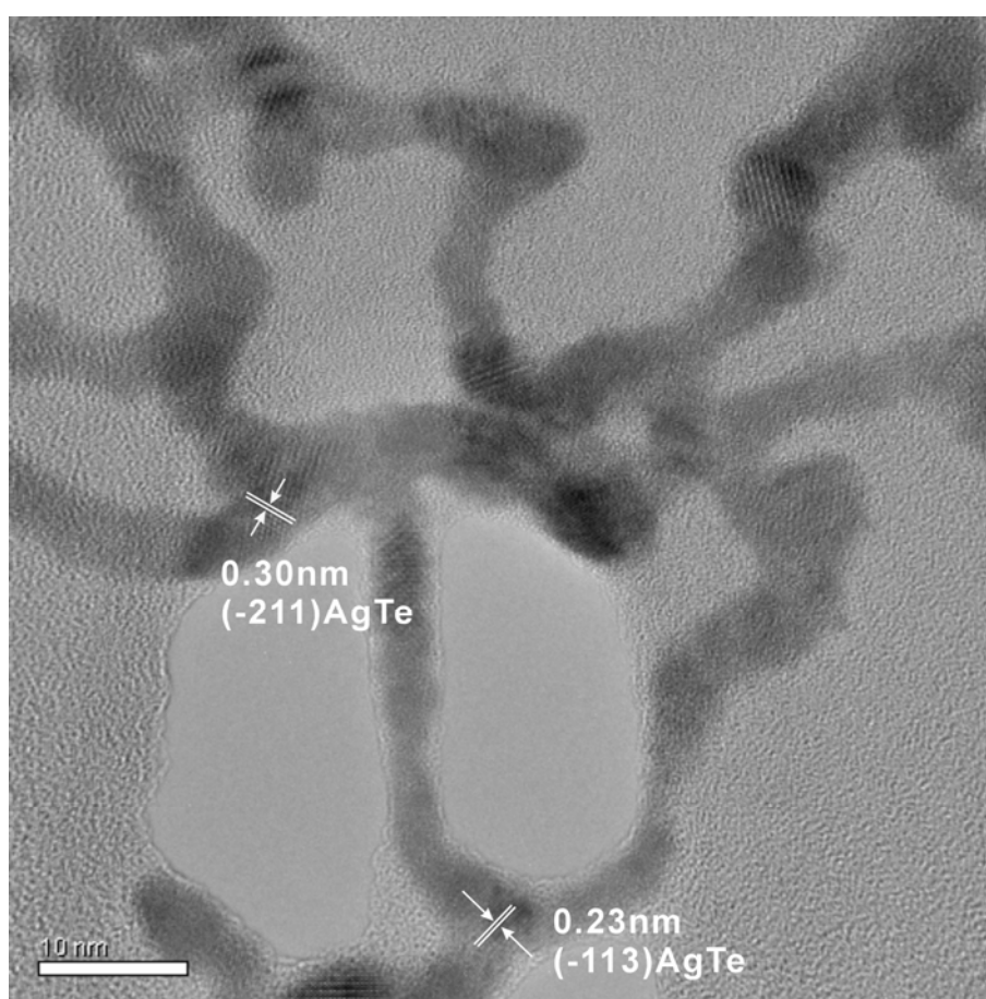
Figure S1. HRTEM image of \text{Ag}_2\text{Te} nanowire network.
