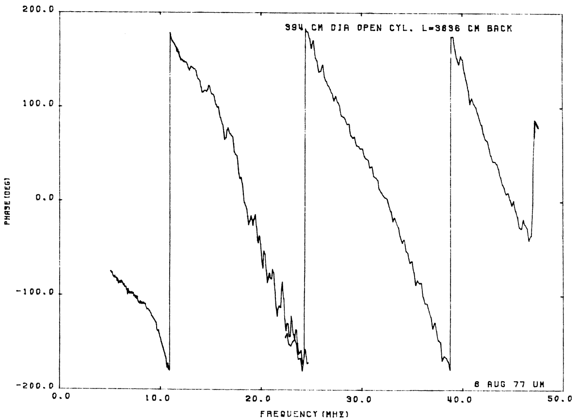
Figure B.10: Current at back center of cylinder No. 2b.
