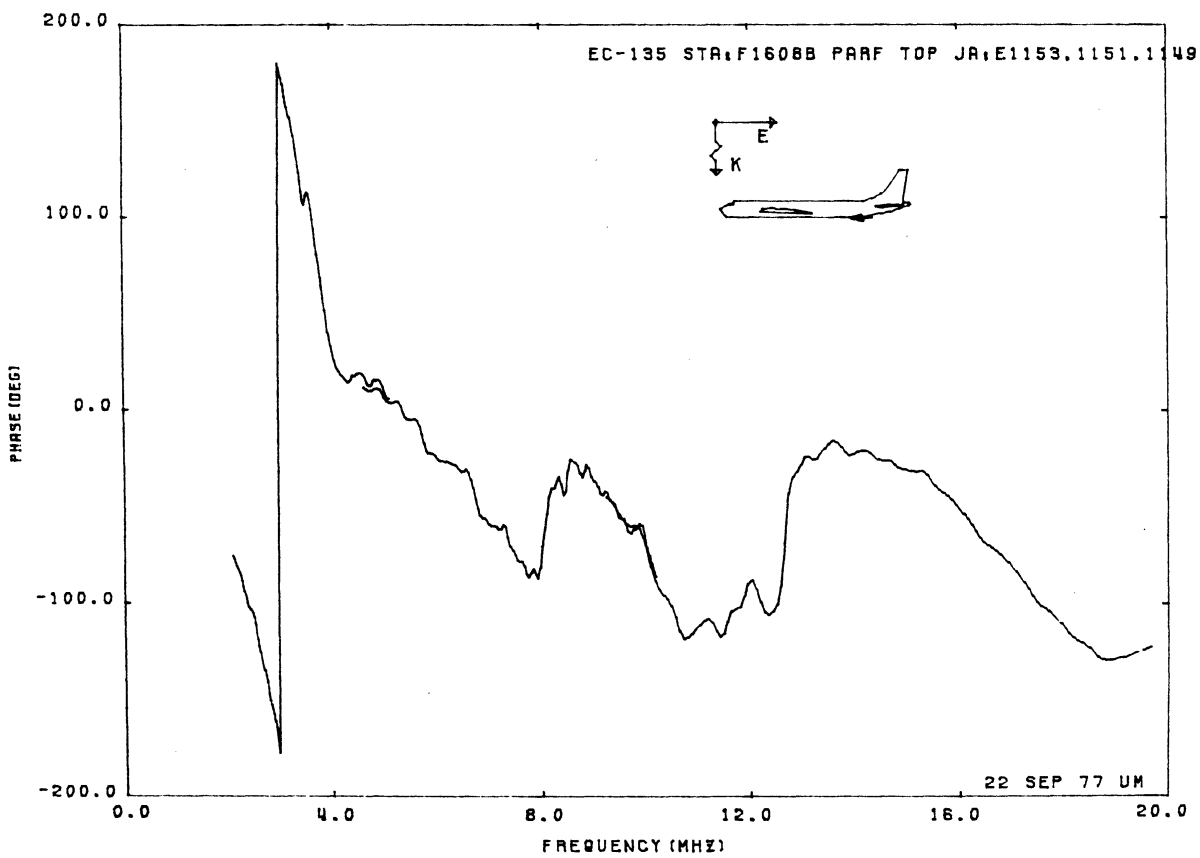
Figure 2: Data of Figure 1 filtered with f_c = 20 and n = 2 .
