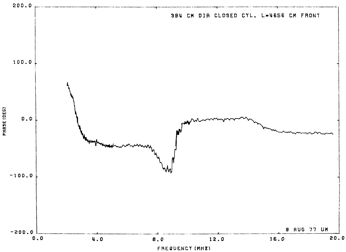
Figure B.1: Current at front center of cylinder No. 1.
