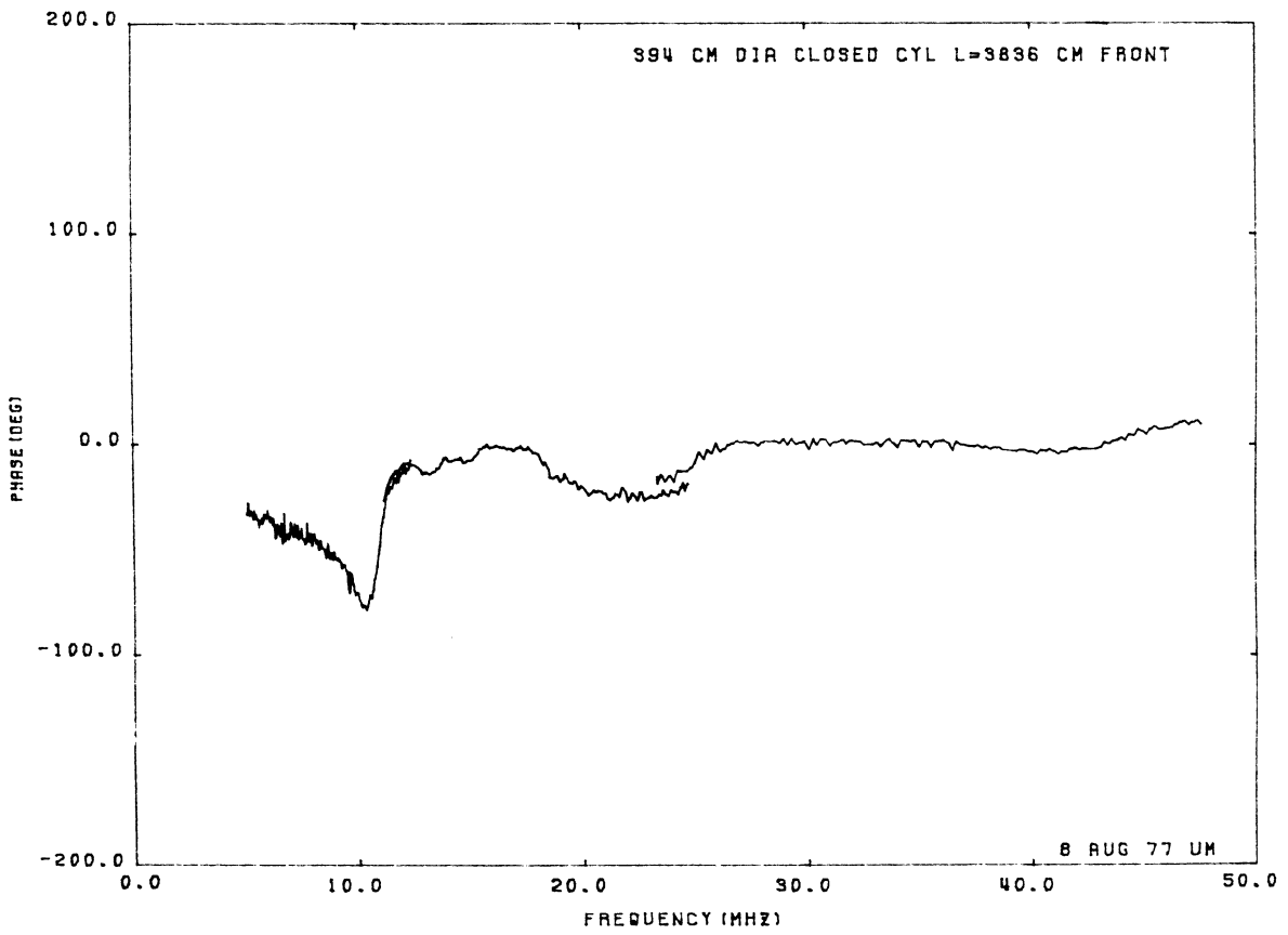
Figure B.5: Current at front center of cylinder No. 2a.
