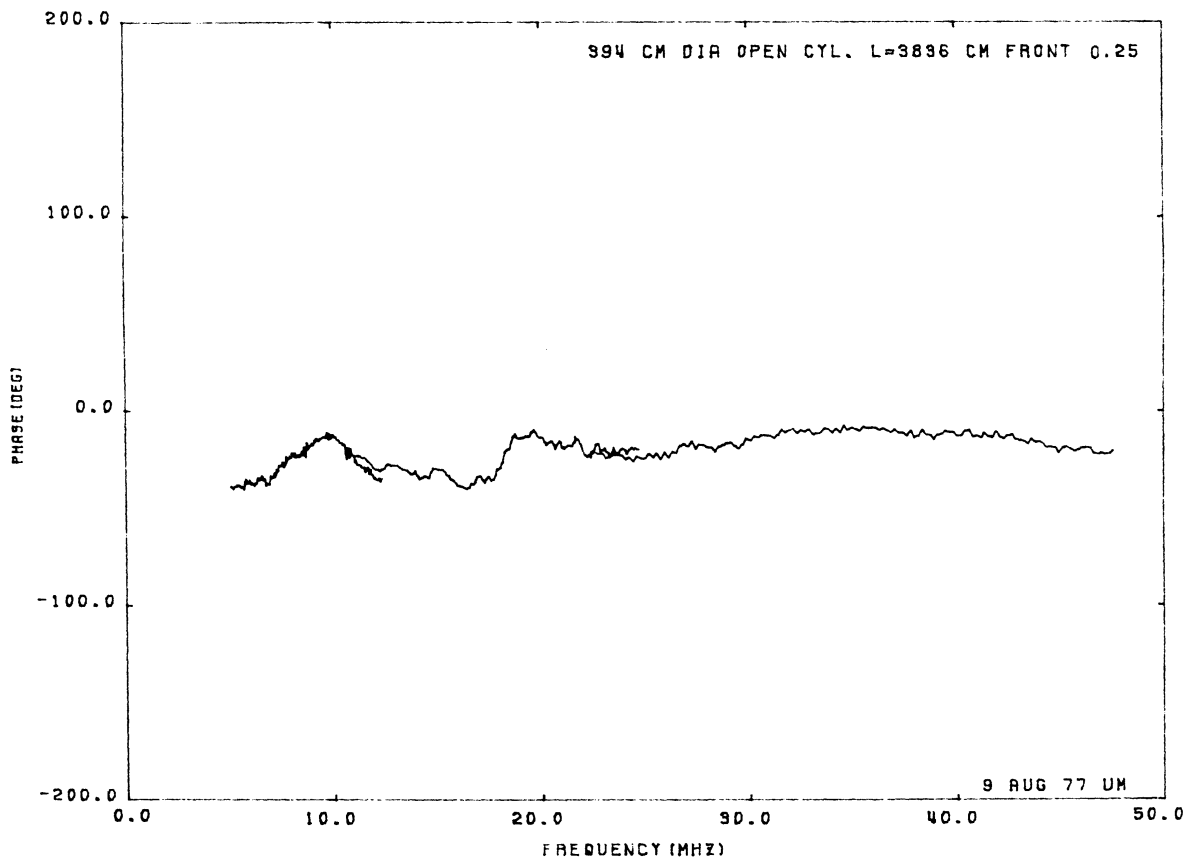
Figure B.11: Current at front 1/4 of cylinder No. 2b.
