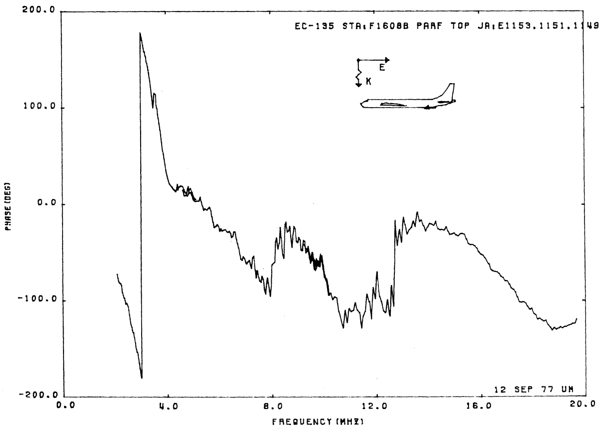
Figure 1: Raw data measured on EC-135 at STA:F1608B.
