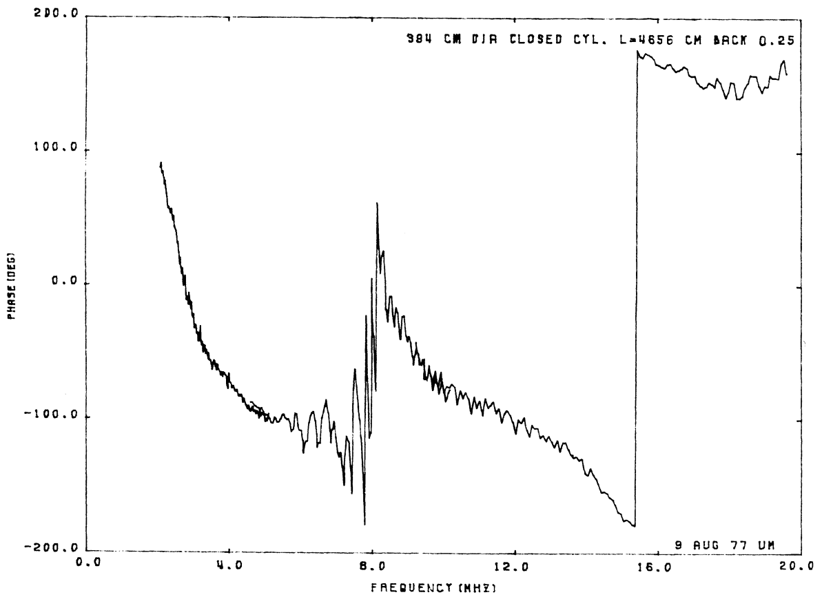
Figure B.4: Current at back 1/4 of cylinder No. 1.
