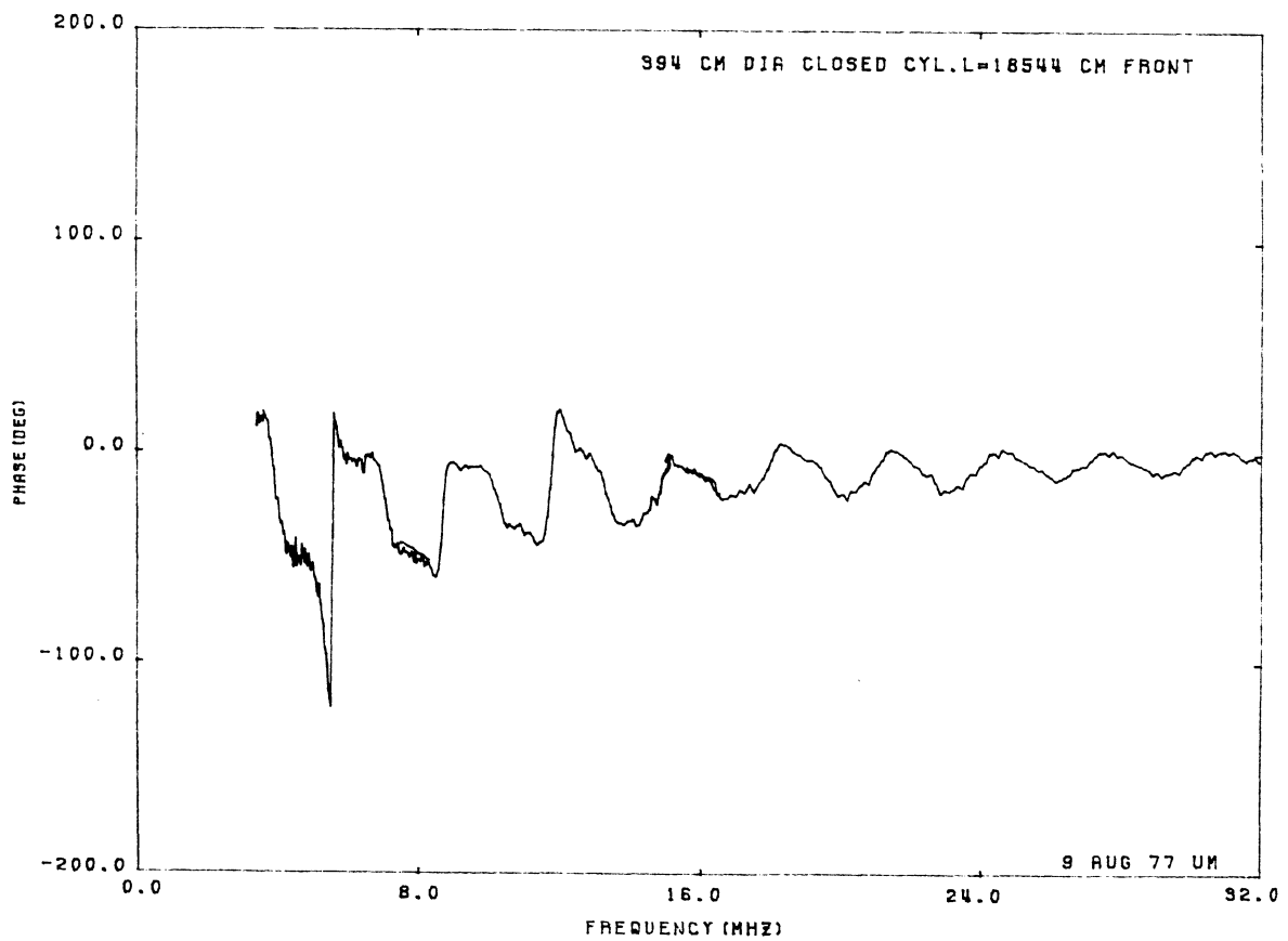
Figure B.13: Current at front center of cylinder No. 3.
