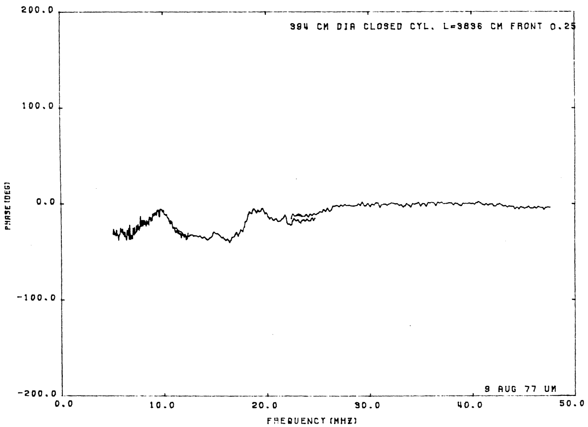
Figure B.7: Current at front 1/4 of cylinder No. 2a.
