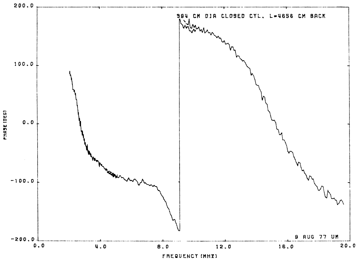
Figure B.2: Current at back center of cylinder No. 1.
