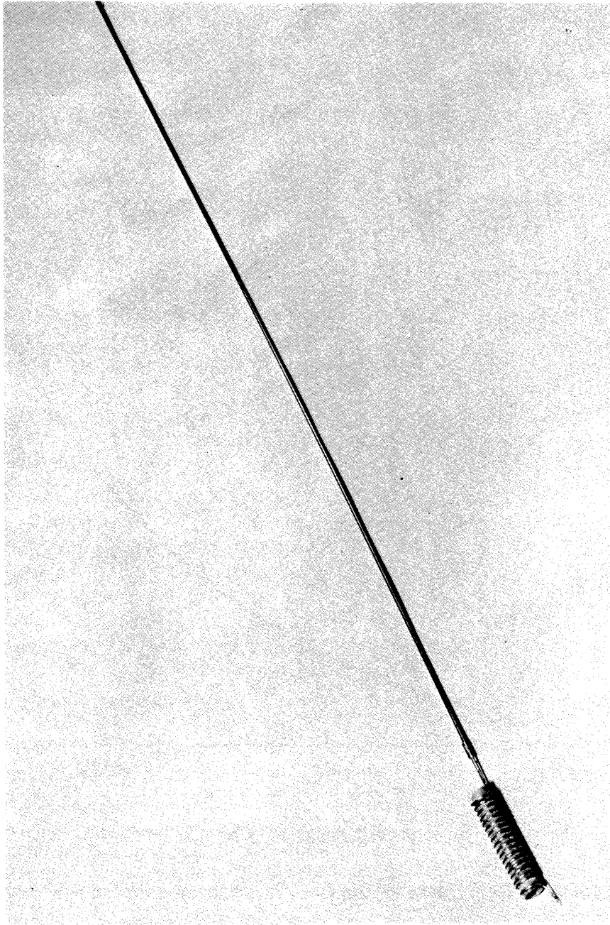
FIG. 3-12: The 75 cm Monopole With the Inductor L_1 Connected in Series.
