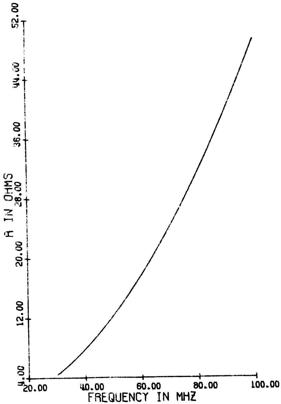
FIG. 2-1: Calculated Resistance of a Short Monopole: length = 75 cm, diameter = 0.1 cm.
