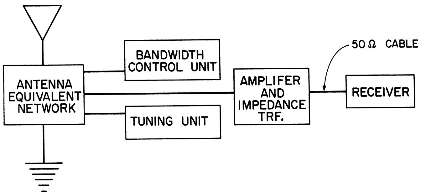
FIG. 1-4: Block Diagram for Voltage Tunable Antenna.
