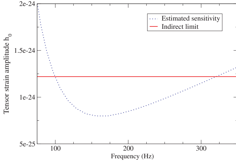
Figure 1. Estimated sensitivity of an S5 search compared to the indirect limit on GW emission for Cas A. Search parameters are the fiducial ones described in the text.
