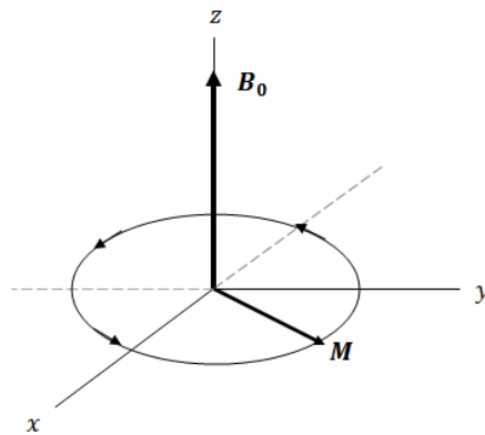
Figure 1.10: Using an RF-pulse to introduce a magnetic field orthogonal to \mathbf{B}_0 results in the precession of \mathbf{M} around the z -axis at frequency \omega_0 = \gamma|\mathbf{B}_0| .
