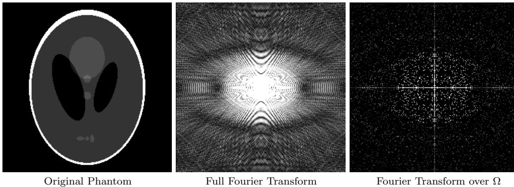
Figure 3.12: Original Shepp-Logan Phantom along with its full and partial Fourier Transforms.
