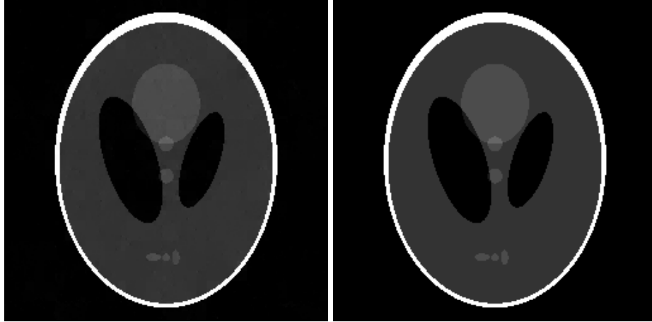
Figure 3.5: Shepp Logan phantom with streakiness corrected by the Haar Wavelet method vs. the original phantom.
