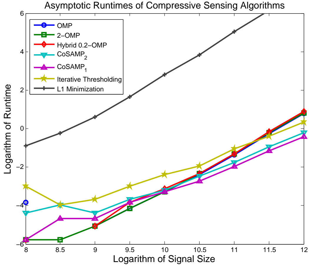
Figure 2.11: Log-log plot of the average runtimes of compressive sensing algorithms as a function of the signal length.
