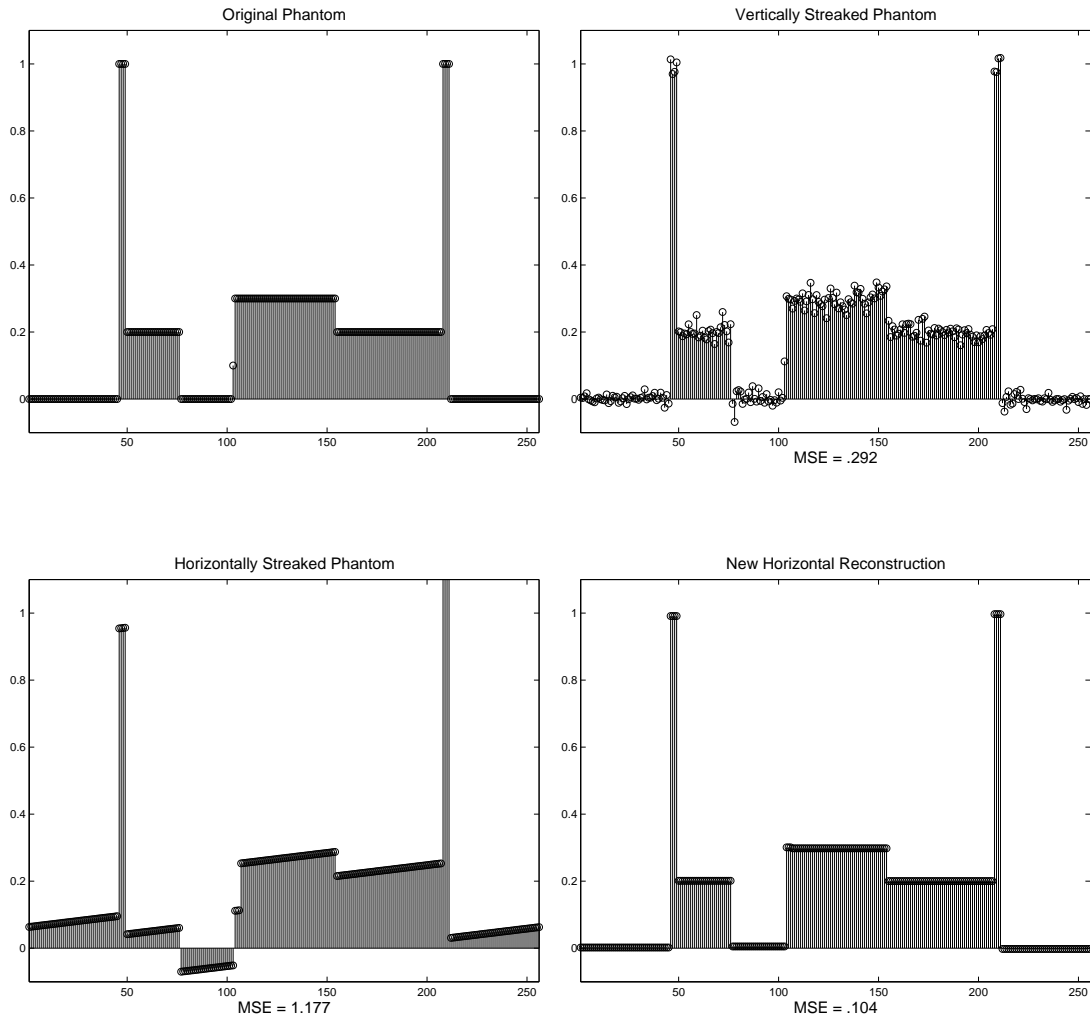
Figure 3.6: Cross-sections of original phantom, vertically streaked phantom, horizontally streaked phantom, and finally the reconstruction of the horizontally streaked image based on the cross-section method.
