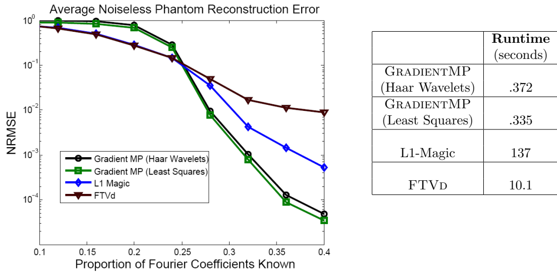
Figure 3.15: Reconstruction NRMSEs and Runtimes of GRADIENTMP and TV-Minimization with respect to recovering a 64 \times 64 Shepp-Logan phantom.
