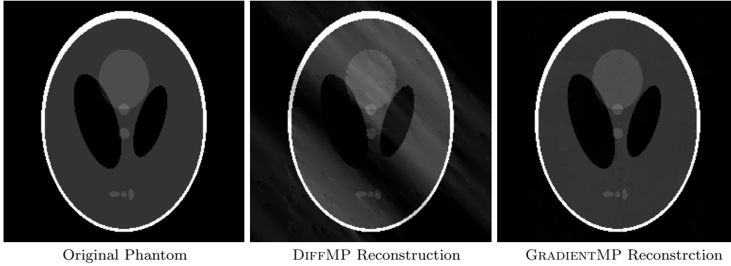
Figure 3.2: Comparison of DIFFMP and GRADIENTMP reconstructions of a Shepp-Logan phantom from 6.6% of its Fourier coefficients.
