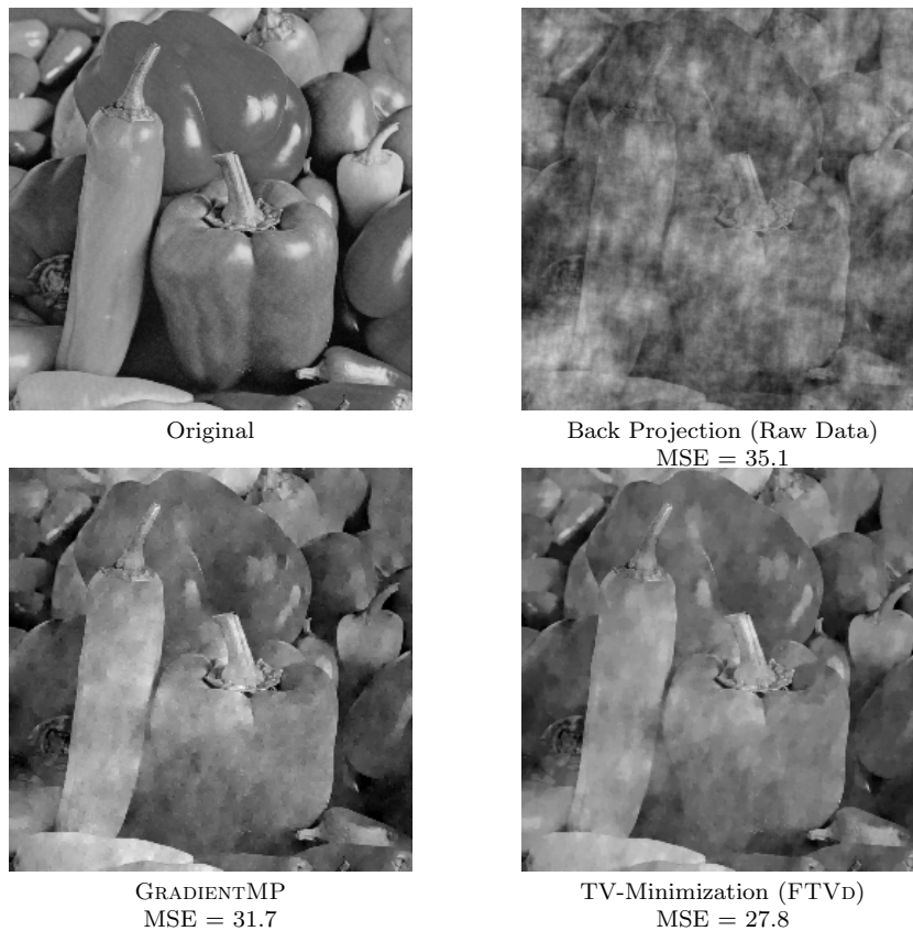
Figure 3.17: Original peppers image and reconstructions using Fourier Back Projection, GRADIENTMP, and FTV D .
