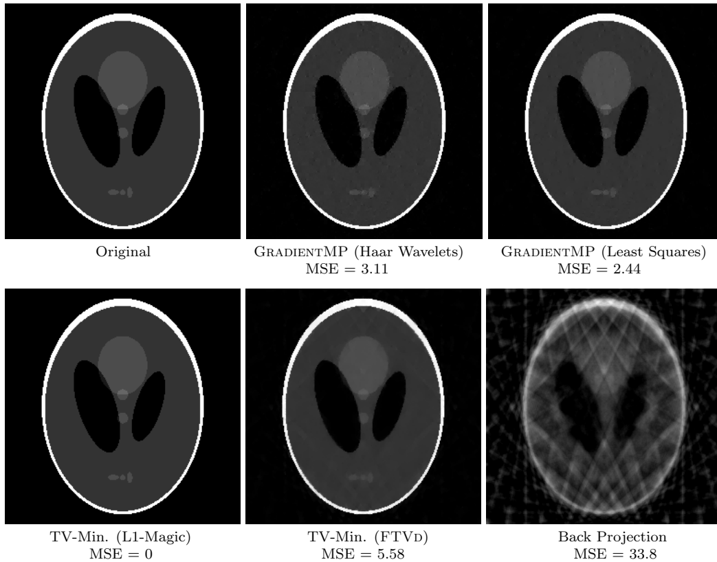
Figure 3.14: Various reconstruction of the Shepp-Logan phantom from Fourier Coefficients along radial lines.
