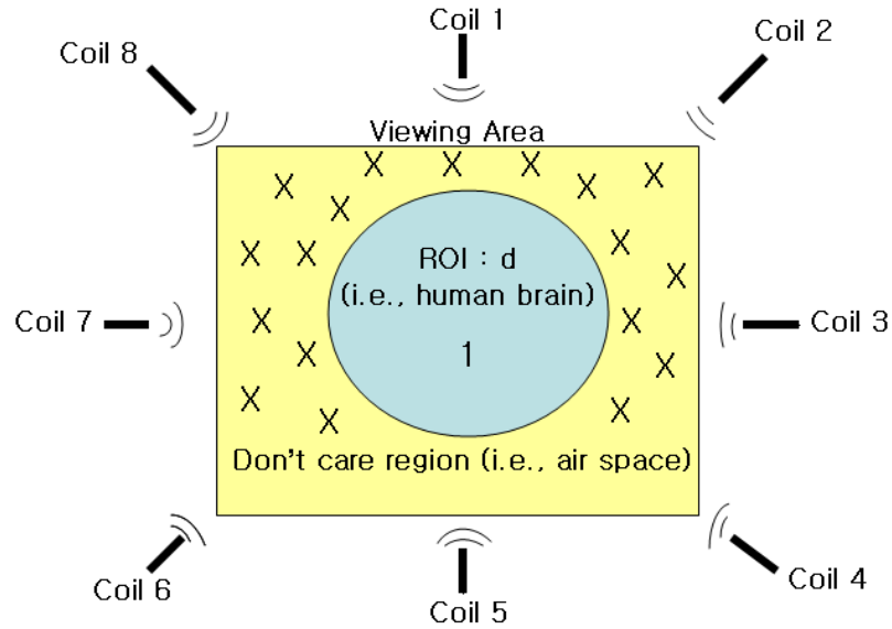
Figure 4.3: An idealized in-plane excitation profile that is identically one over the region of interest.
