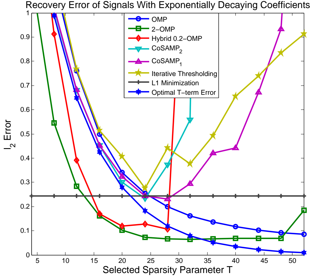
Figure 2.9: Average reconstruction errors in recovering signals with exponentially decaying coefficient generated by the various compressive sensing algorithms as a function of the sparsity parameter T .
