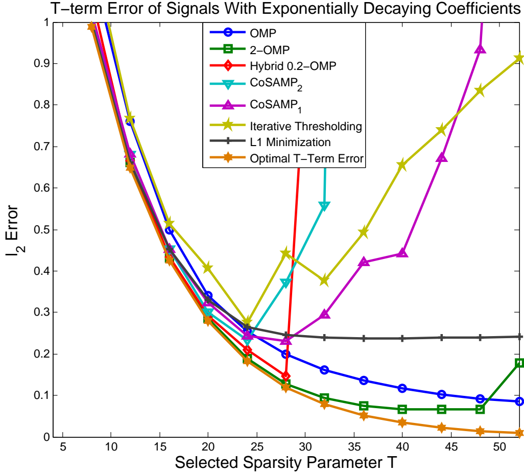
Figure 2.10: Average T -term reconstruction errors in recovering signals with exponentially decaying coefficient generated by the various compressive sensing algorithms as a function of the sparsity parameter T .
