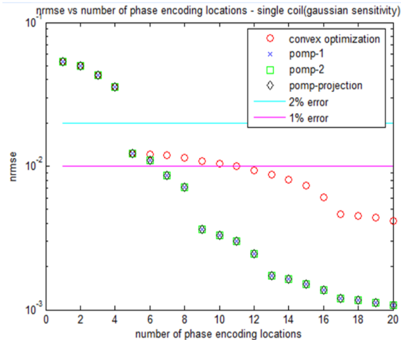
Figure 4.8: The NRMSEs of the excitation patterns induced by convex optimization and the three variations of POMP in the case of a single coil MRI setup
