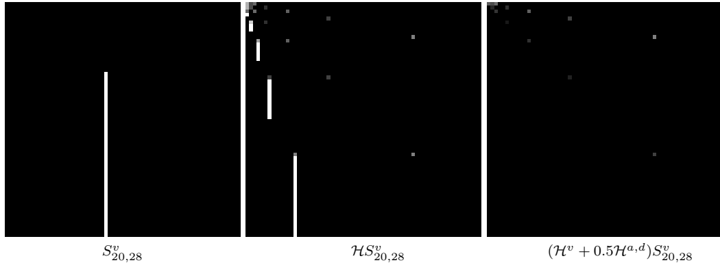
Figure 3.10: Single streak image along with its full Haar Wavelet Transform as well as its Haar Wavelet Transform restricted to vertical and diagonal differences only.
