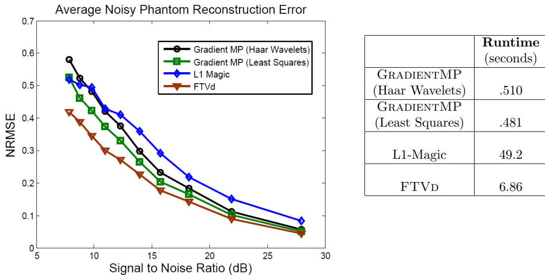
Figure 3.16: Reconstruction NRMSEs and Runtimes of GRADIENTMP and TV-Minimization with respect to recovering 64 \times 64 Shepp-Logan phantoms corrupted with a significant amount of white Gaussian noise.
