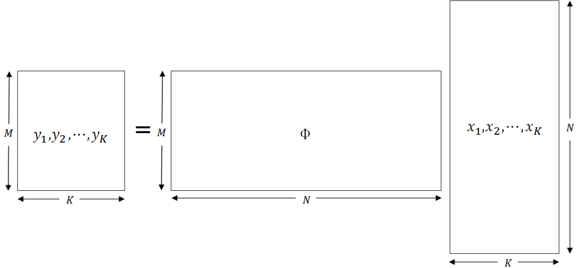
Figure 1.6: A schematic of the basic simultaneous compressive sensing problem
