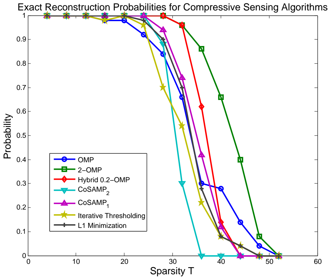
Figure 2.7: Probability of exact reconstruction of T -sparse signals using various compressive sensing algorithms.
