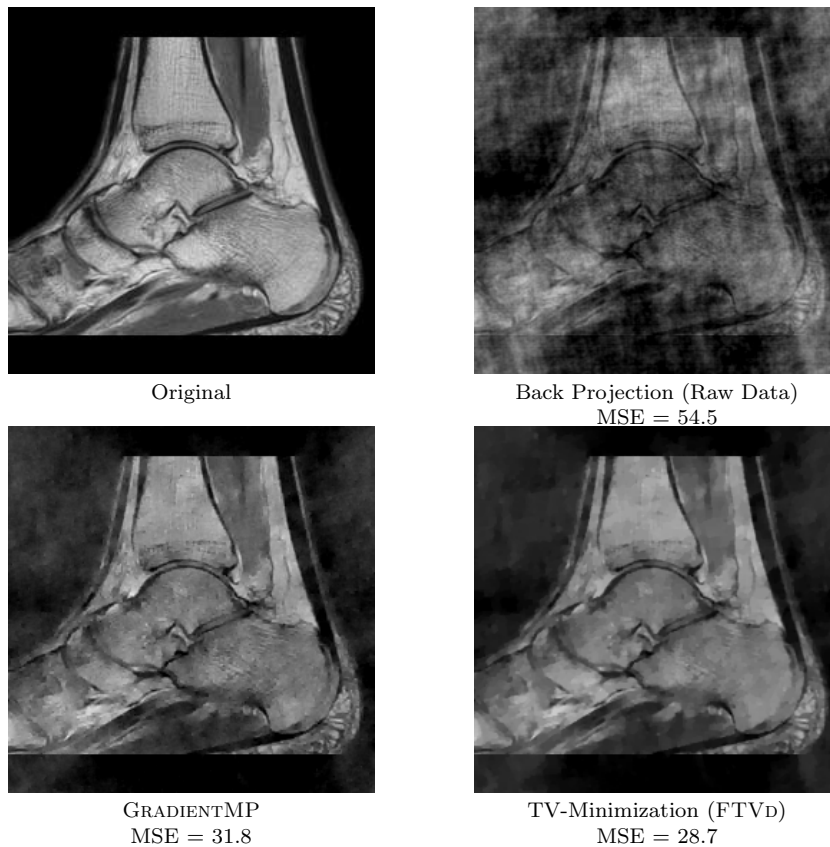
Figure 3.18: Original medical image and reconstructions using Fourier Back Projection, GRADIENTMP, and FTVd.
