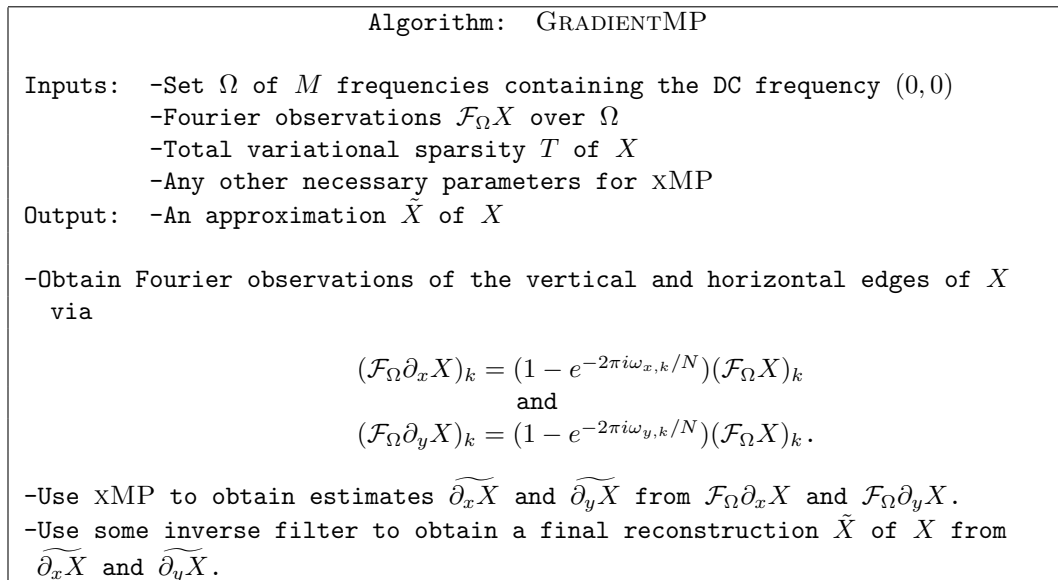
Figure 3.1: Outline of the GRADIENTMP algorithm.
