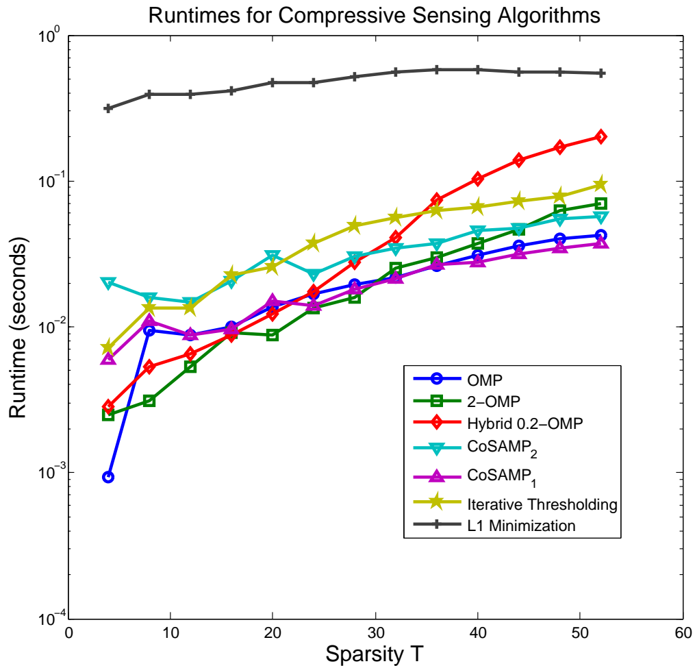
Figure 2.8: Runtimes of various compressive sensing algorithms when recovering T -sparse signals.
