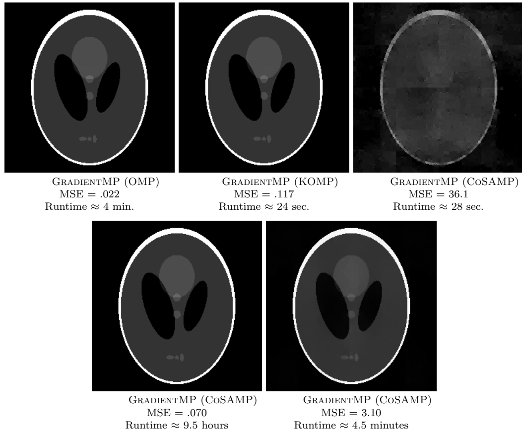
Figure 3.13: Various reconstruction of the Shepp-Logan phantom from 10% of its Fourier Coefficients.
