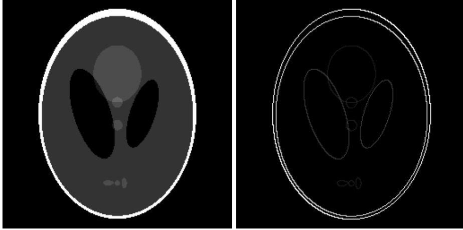
Figure 1.1: The famous Shepp-Logan Phantom image: a classical example of a sparse gradient image.
