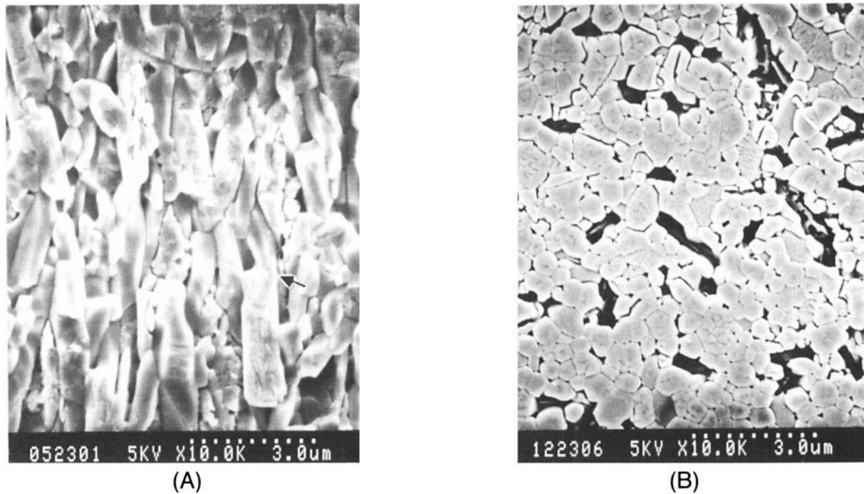
Fig. 6. SEM micrographs of a specimen after tensile deformation at 1550°C, \dot{\epsilon}_0 = 10^{-4} \text{ s}^{-1} , to \delta = 246\% , sectioned (A) parallel (L) and (B) perpendicular (W) to the tensile direction.
