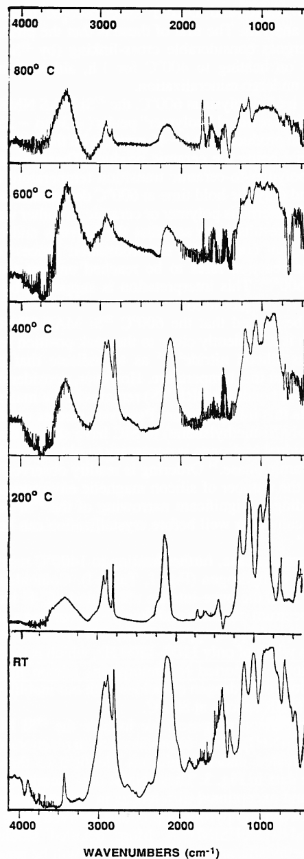
Fig. 5. Diffuse reflectance infrared fourier transform spectra (DRIFTS) of [\text{H}_2\text{SiNMe}]_x - samples pyrolyzed to selected temperatures. Data points for 1-g samples heated at 5^{\circ}\text{C}/\text{min}/\text{N}_2 to temperature and held for 1 h.
