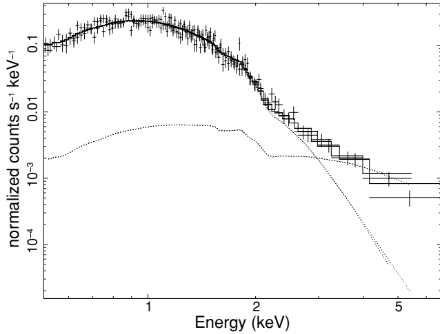
Figure 1. Spectra of both Chandra observations, along with the model fit (solid line) for D = 7.4 kpc, \Gamma = 1 and M = 1.4M_{\odot} . The dotted lines indicate the nsatmos and power-law components.
