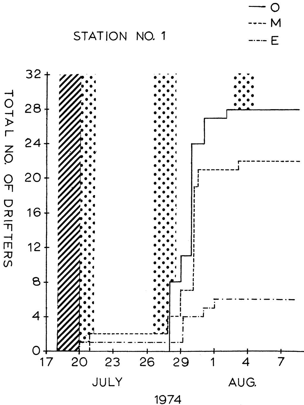
Figure E6: Cumulative drifter return numbers for each of three drifter types released at point No. 1 plotted separately versus time adrift. O-ring drifters. M-Mobius drifters. E-vertical envelopes. Hatching indicates dates of release for July cruise. Dot filled columns delineate weekends.
