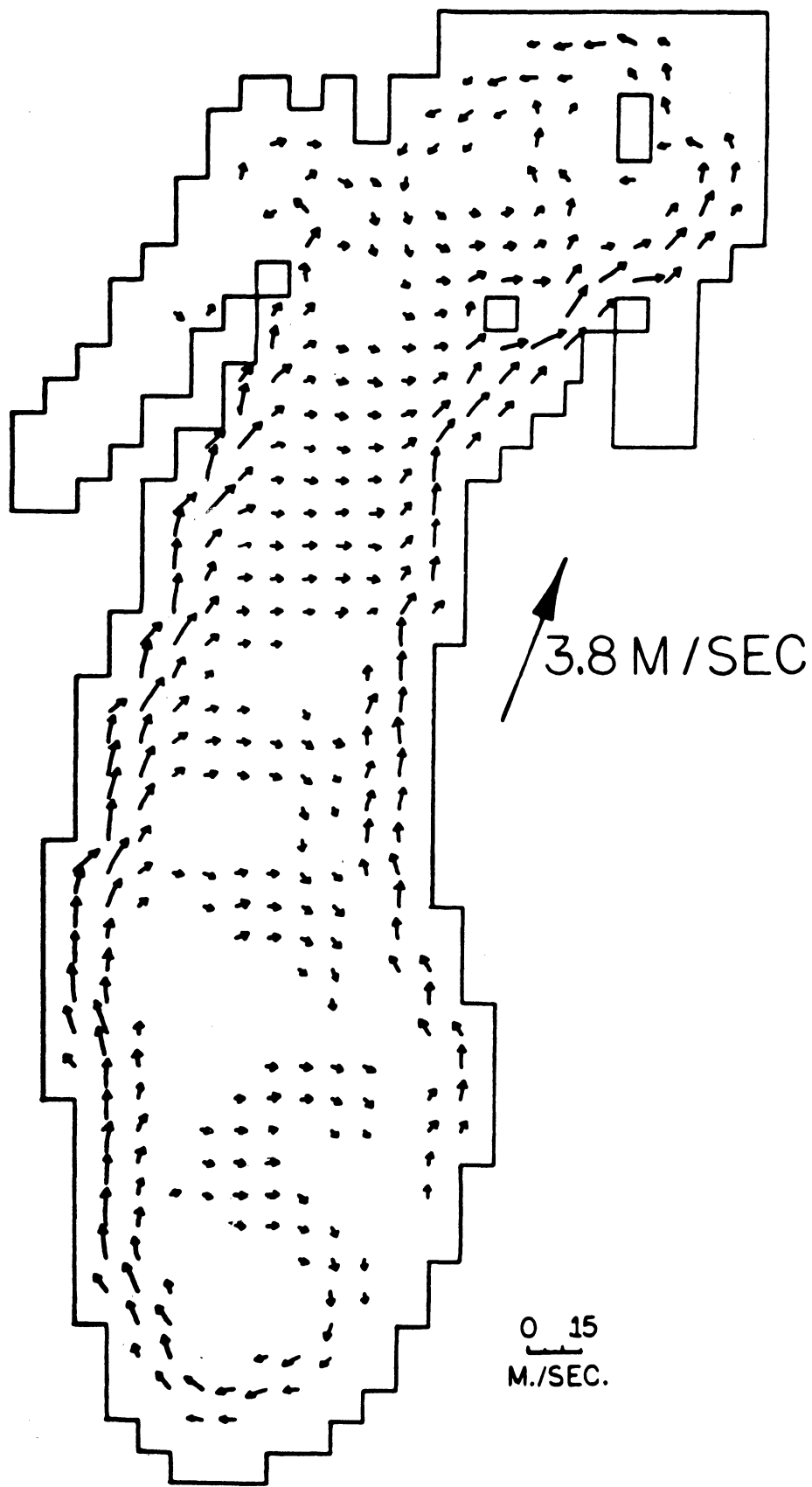
Figure 40 Current predictions from a computer model by Kizlauskas and Katz (1973).
