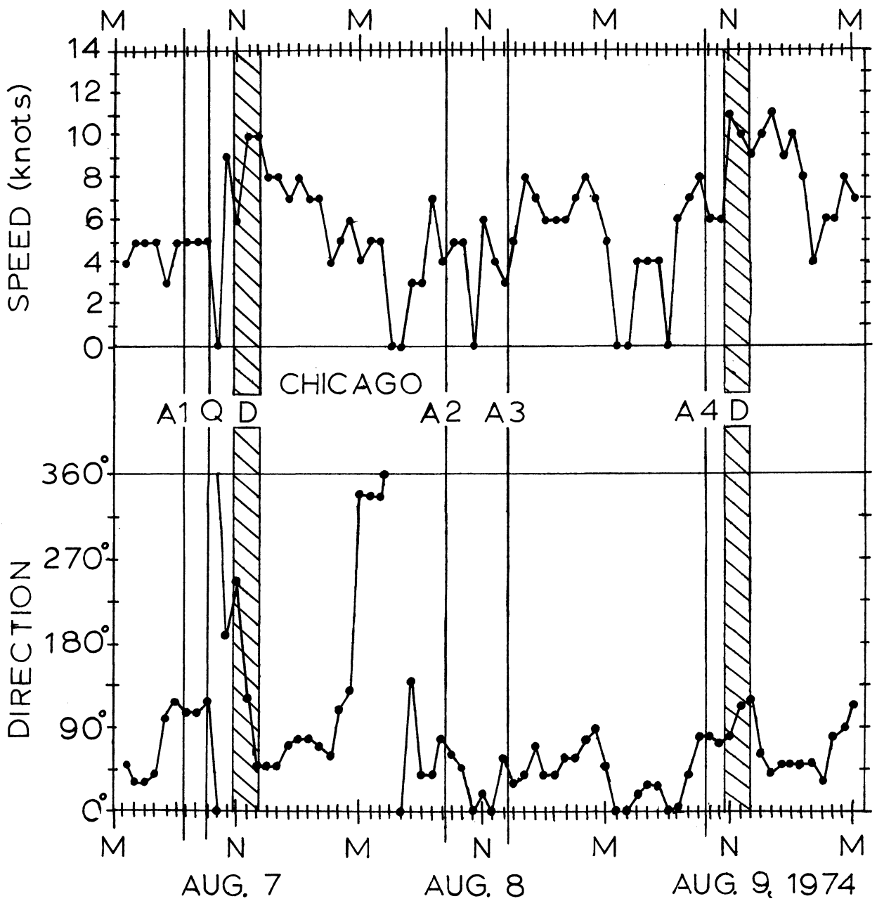
Figure 12: Chicago wind history (speed and direction versus time) for interval 7-9 August 1974. In accord with meteorological convention, wind direction is that from which wind is blowing. Vertical lines indicate time at which various stations were occupied. Hatched columns indicate intervals when drogues were adrift.
