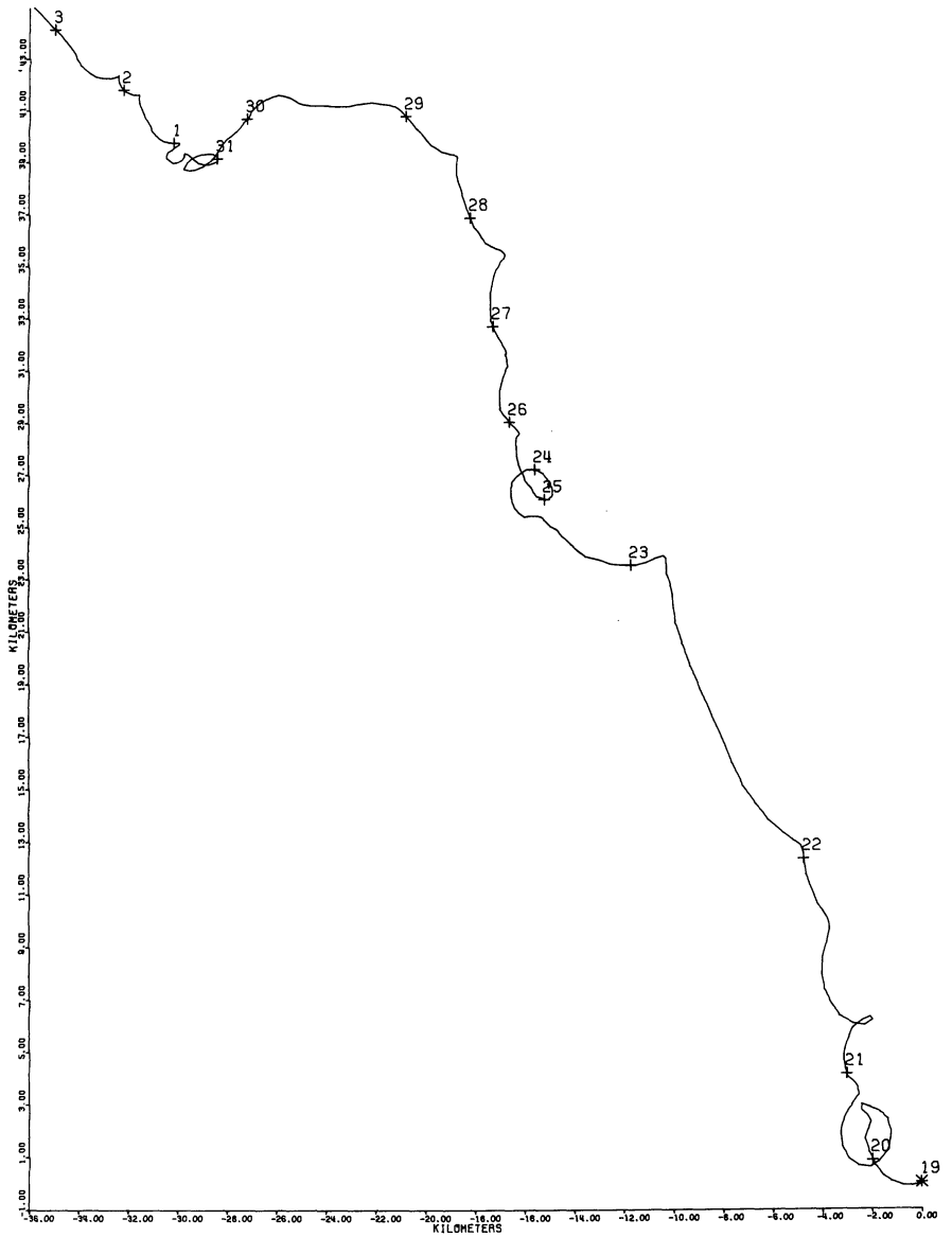
Figure 24: Mooring "Q" progressive vector diagram.
