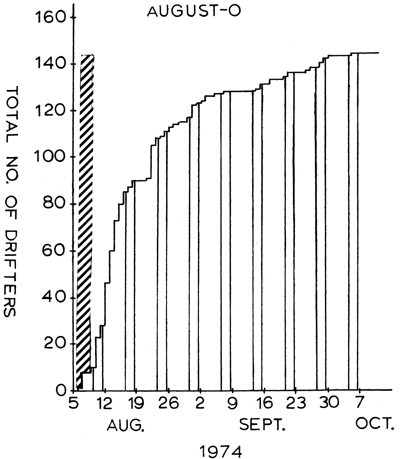
Figure E4: Cummulative drifter return number for Ring Drifters released during 5-10 August Cruise versus time adrift. Hatching indicates dates of release. Narrow vertical columns delineate weekends.
