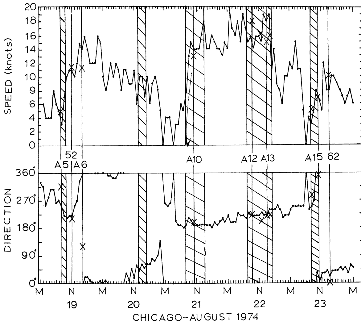
Figure 18: Chicago wind history (speed and direction versus time) for interval 19-23 October 1974 (NOTE: LEGEND INDICATING AUGUST IS INCORRECT). Vertical lines indicate time at which various anchor stations were occupied. Hatched columns indicate intervals when drogues were adrift. X's represent wind data measured aboard the R/V LAURENTIAN.
