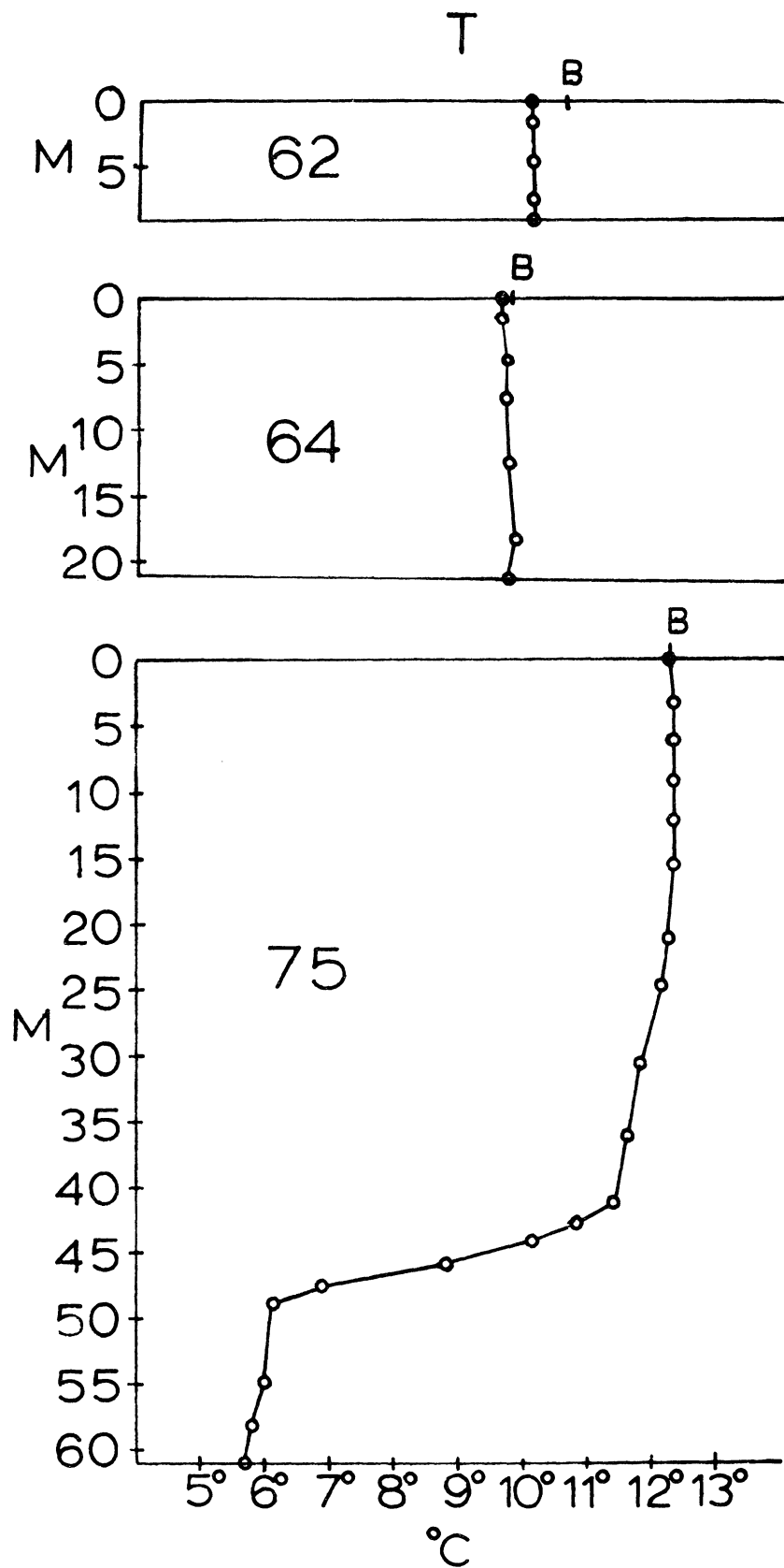
Figure 17: Additional temperature profiles. Vertical bars marked B; surface bucket temperatures. Depth in meters.
