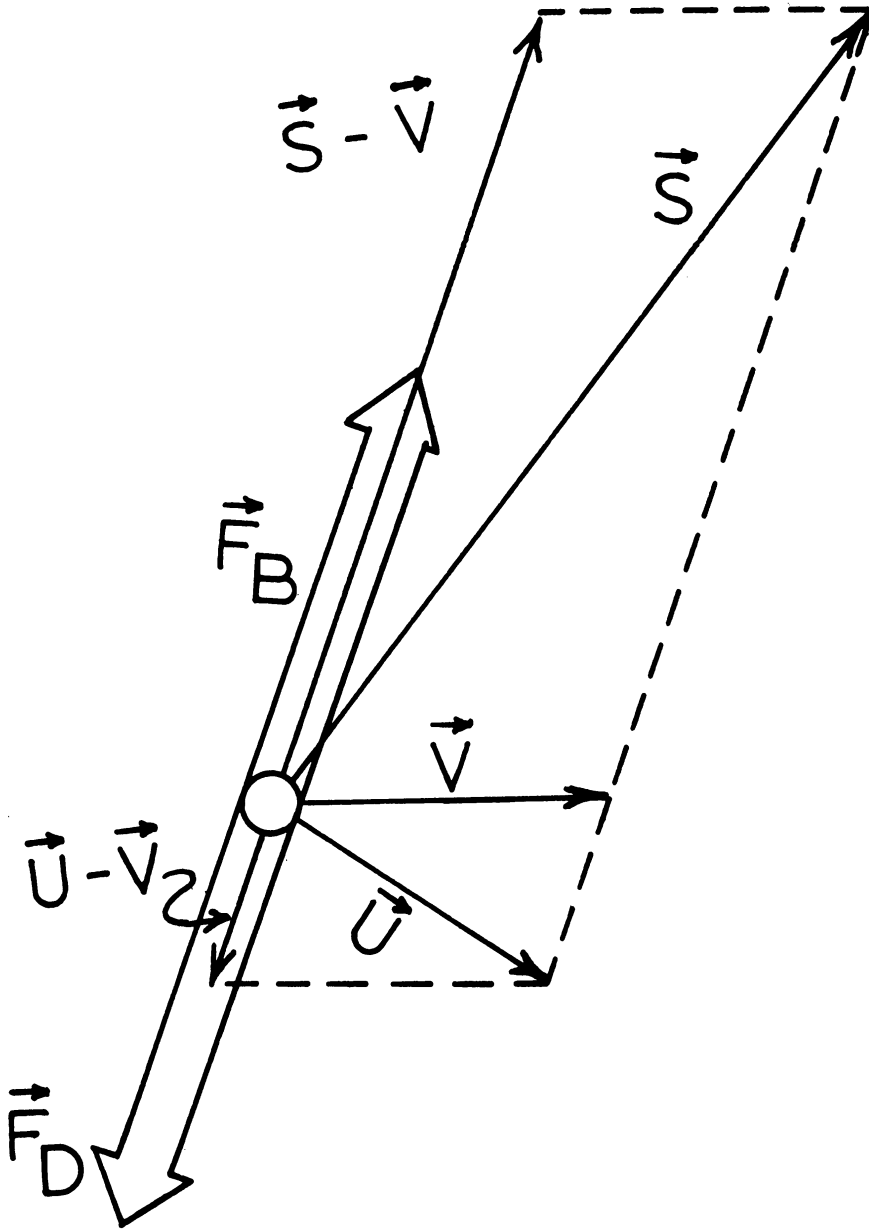
Figure D3: Drogue Mechanics in Planar View. Thin arrows are current vectors. Thick arrows are force vectors. Symbols defined in Table DI.
