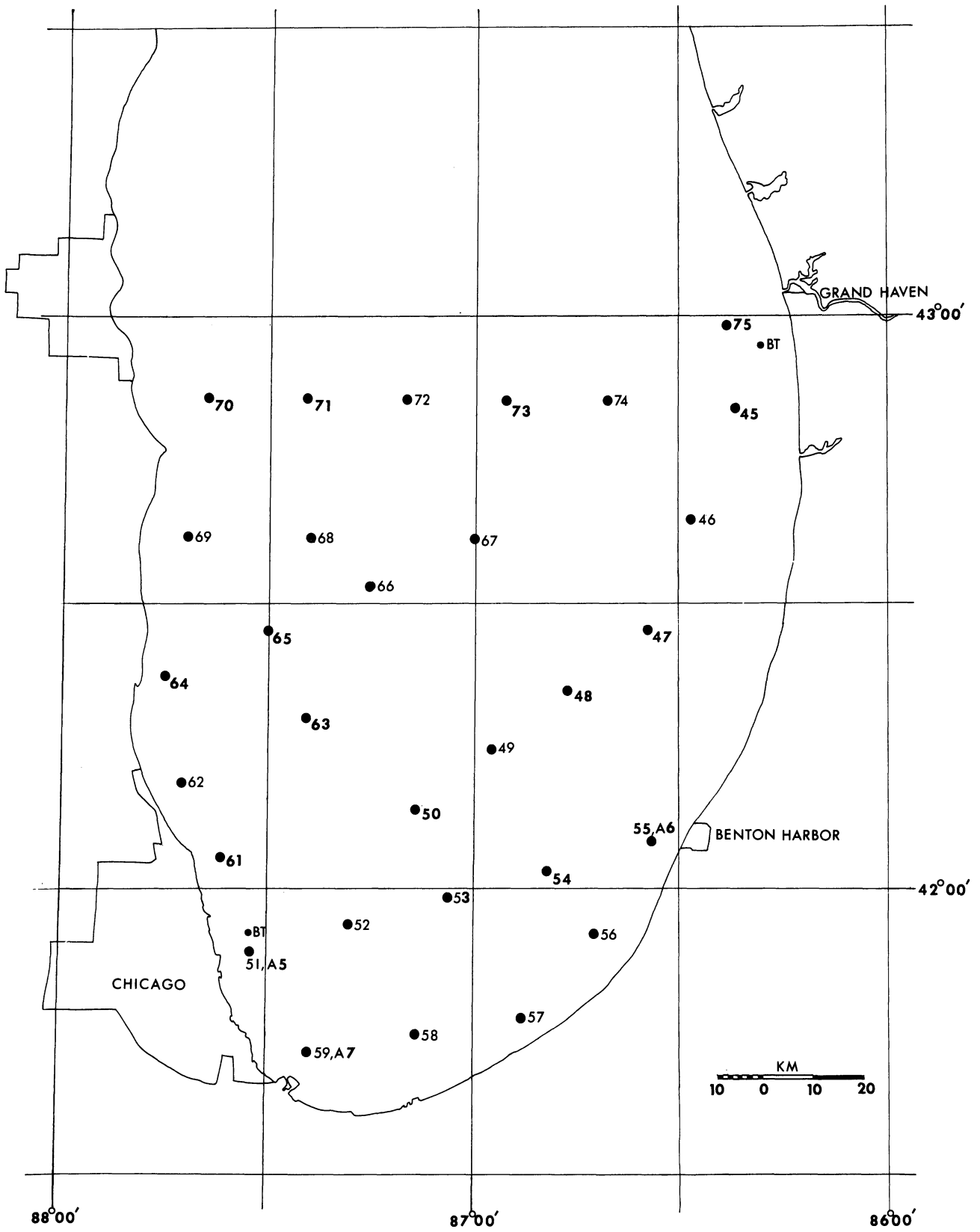
Figure 5: Small scale cruise chart: 15-24 October 1974.
