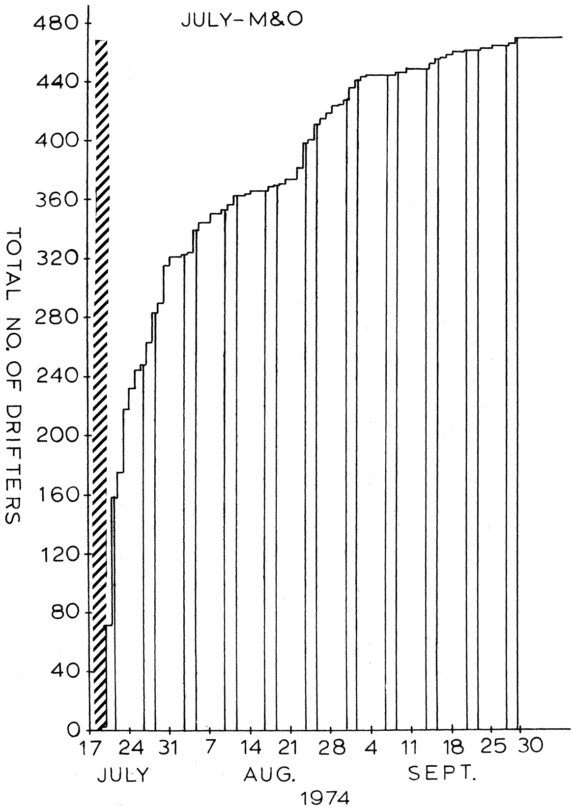
Figure E1: Cumulative drifter return number for all Mobius and Ring Drifters released during 18-20 July 1974 cruise versus time adrift. Hatching indicates dates of release. Narrow vertical columns delineate weekends.
