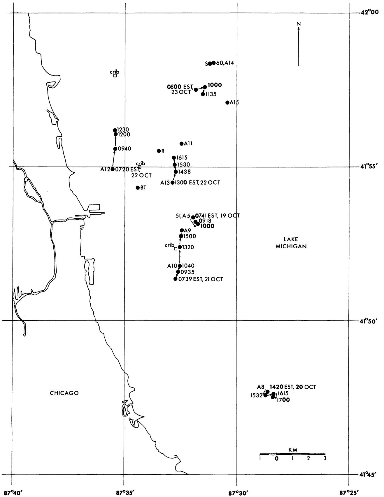
Figure 6: Detailed cruise and drogue chart: 15-24 October 1974.
