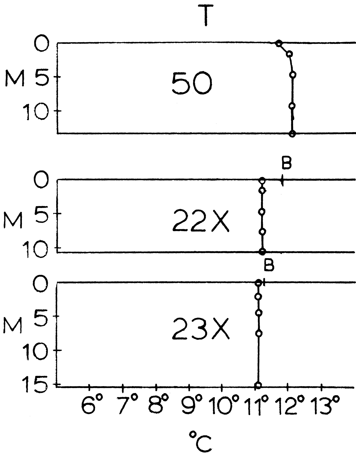
Figure 16: Additional temperature profiles. Vertical bars marked B; surface bucket temperature. Depth in meters.
