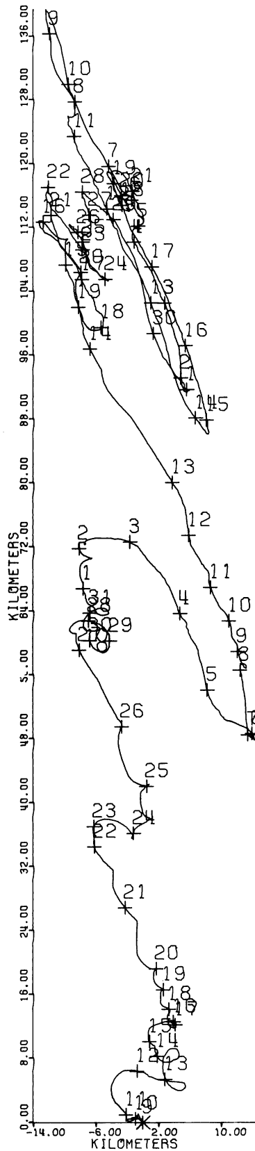
Figure 29: Mooring "R" progressive vector diagram.
