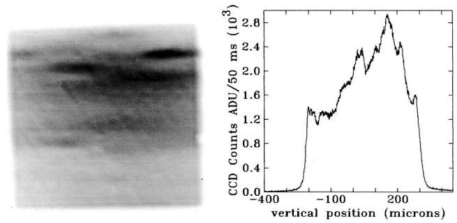
FIG. 1. (Left-hand side image) Inverted gray scale image (black is the highest intensity) of the square beam, 0.51 ( V ) by 0.53 ( H ) mm x-ray beam at 10.87 keV, unfocused. (Right-hand side image) A typical vertical slice of the image, near the undulator beam center.
