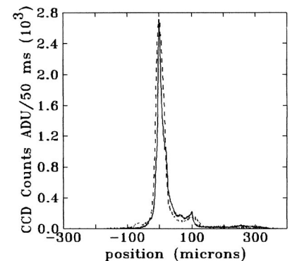
FIG. 2. (Left-hand side image) An inverted gray scale image of the focused x-ray beam in the image plane of the lens with the same CCD exposure as Fig. 1. Several Al foils reduce the intensity by a factor 24. (Right-hand side image) Cross sections through the focus, along x (dashed) and y (solid). The pixel size is 0.93 \mu\text{m} . The image horizontal and vertical FWHM is 33 and 17 \mu\text{m} , respectively.
