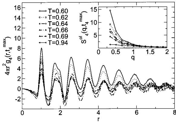
FIG. 11. Temperature dependence of g_4(r, t_4^{\max}) at six values of T , indicated in the legend. Inset shows the structure factor S_4^{\text{ol}}(q, t_4^{\max}) for the same values of T .
