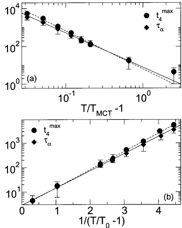
FIG. 7. T dependence of the peak time t_4^{\max} , compared with \tau_\alpha . (a) Fits using MCT in the form of Eq. (2). (b) Fits using VFT in the form of Eq. (3). Error bars are shown only for \tau_\alpha for clarity. Error bars on \chi_4(t) are comparable in size, and are shown in later figures.
