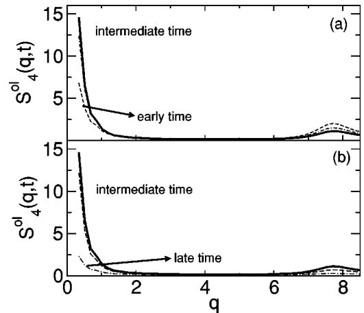
FIG. 10. Time dependence of S_4^{\text{ol}}(q, t) at T=0.60 . S_4^{\text{ol}}(q, t) is shown at times identical to those shown for g_4(r, t) in Fig. 9. Note that the height of the first diffraction peak in S_4^{\text{ol}}(q, t) decreases monotonically as a function of time. This is because it depends on the number of overlapping particles, which decreases monotonically in time (see Fig. 3).
