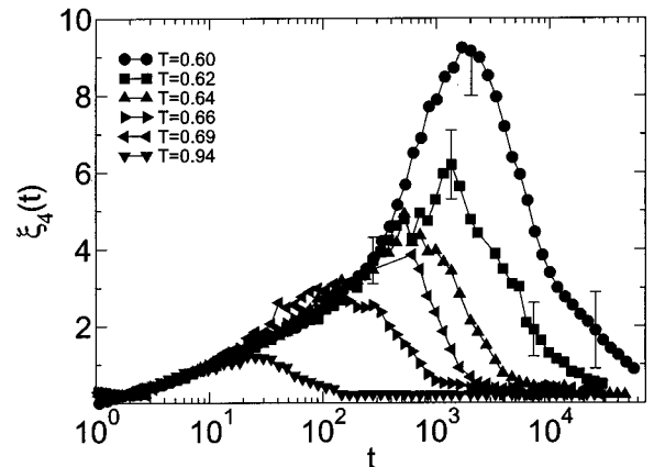
FIG. 13. Time and temperature dependence of \xi_4(t) obtained from the fits to Eq. (30). The data shown are smoothed over successive groups of three points.
