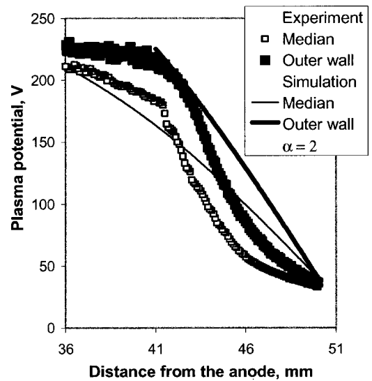
FIG. 9. Measured and calculated potential profiles along the channel median and outer wall for the segmented electrode case. The channel exit is at 46 mm.
