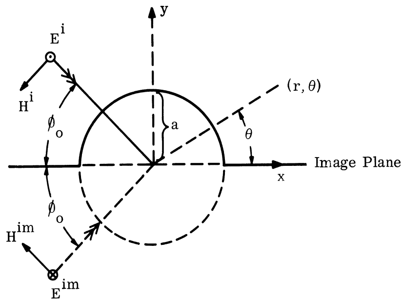
FIG. 5-1: Incident and Image Wave for Horizontal Polarization
