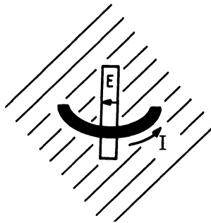
FIG. 6-5: ORIENTATION FOR A SLOT AND A HALF-LOOP ON A CONDUCTING PLANE FOR SIMILAR RADIATION.
