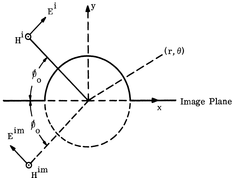
FIG. 5-2: Incident and Image Wave for Vertical Polarization
