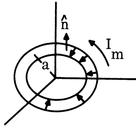
FIG. 6-3: CIRCULAR SLOT OF RADIUS a.
