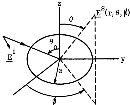
FIG. 3-1: A WIRE LOOP IN THE xy PLANE.
