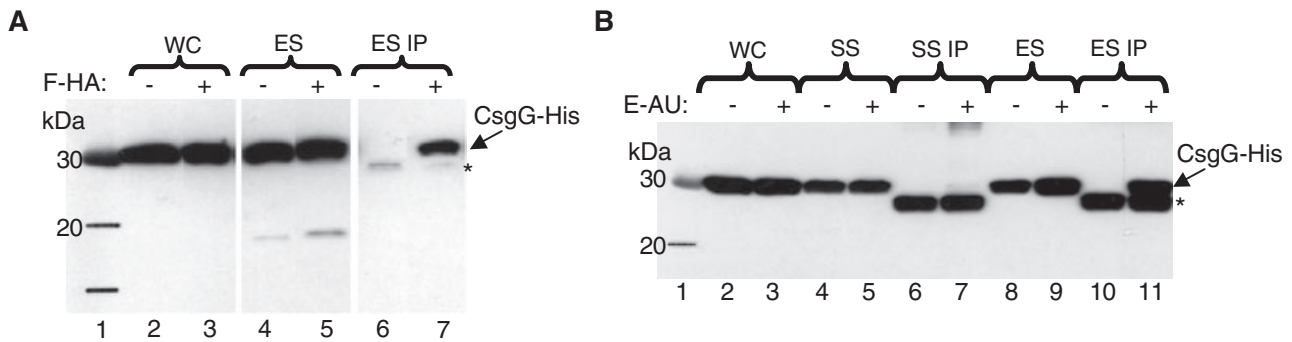
Fig. 5. CsgG interacts with CsgE and CsgF at the outer membrane.
