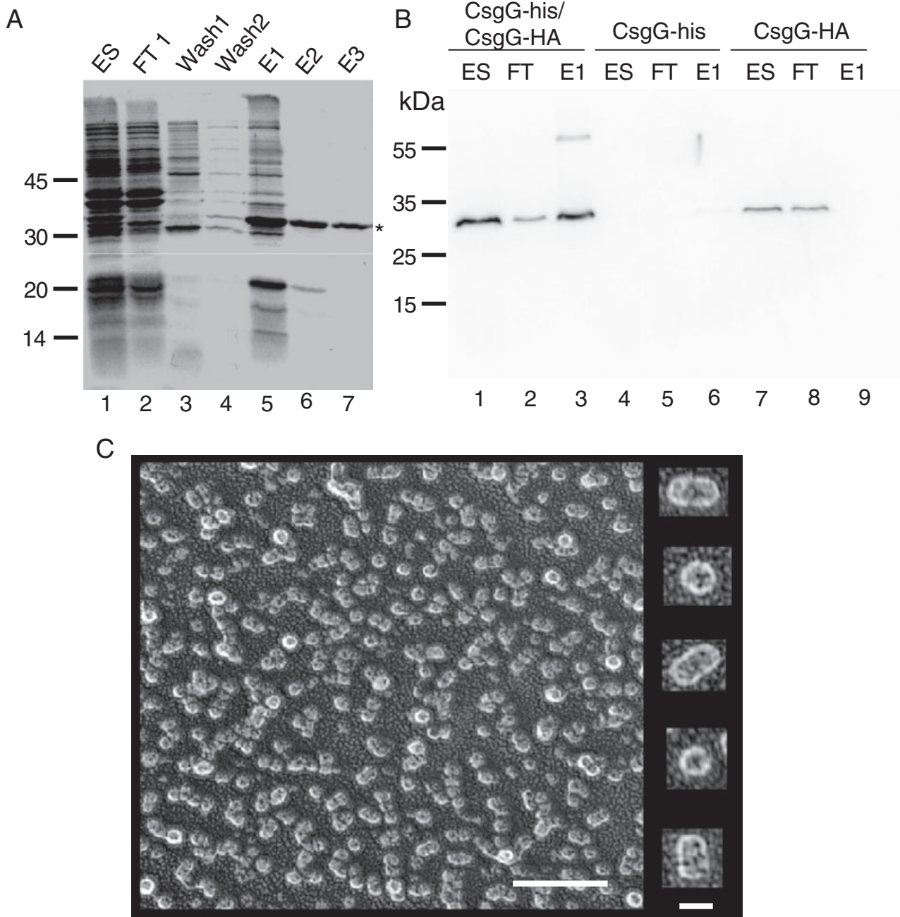
Fig. 2. Purification and structural analysis of CsgG.
