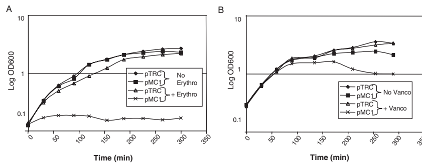
Fig. 3. Antibiotic sensitivity studies.
