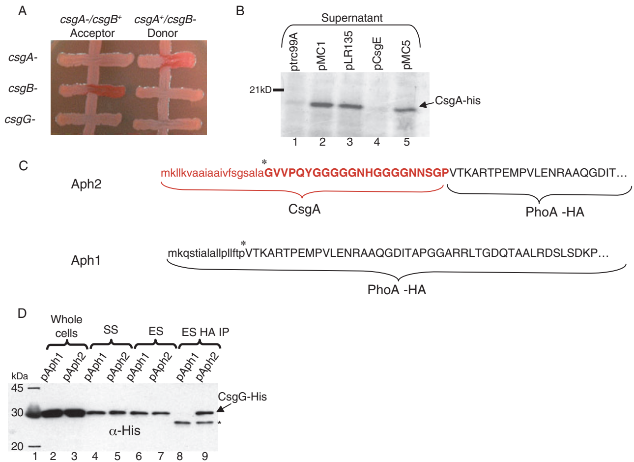
Fig. 1. CsgG is required for interbacterial complementation and CsgA secretion.
