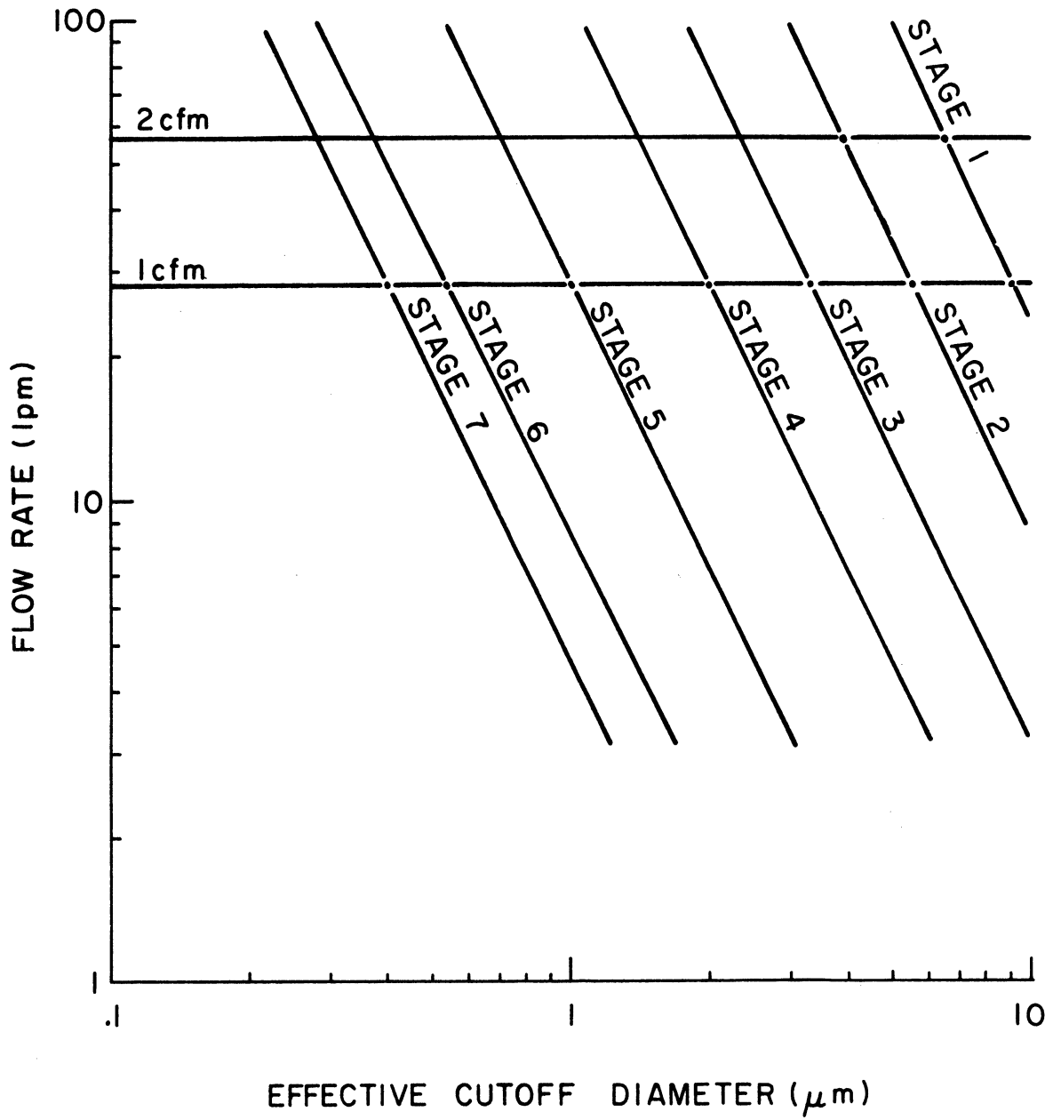
Figure I-1 Flow Rate Dependence for the Effective Cutoff Diameters of the
