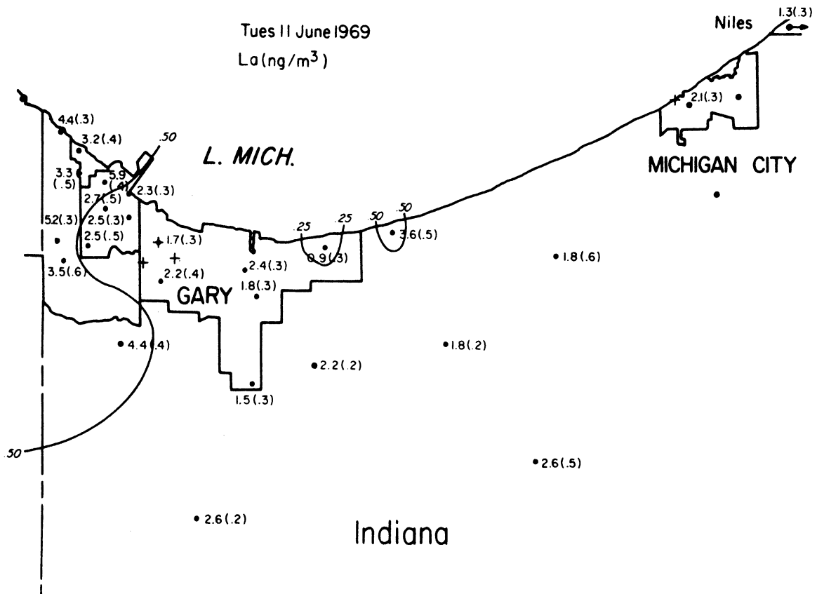
Figure VI-13 Concentration Distribution of Lanthanum
