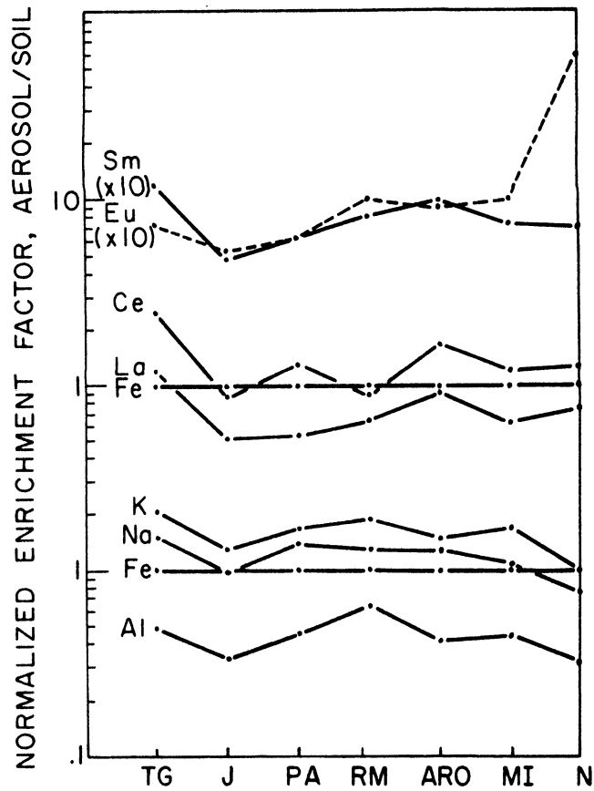
Figure III-16 Normalized Enrichment Factors, Canadian Summer Experiment
