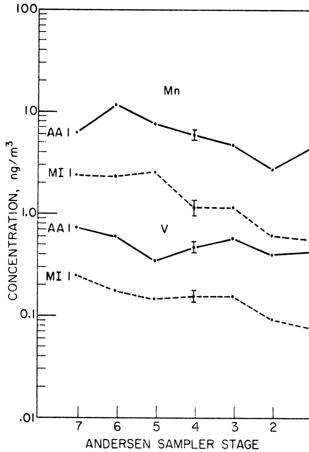
Figure IV-20 AAI - MII Comparison - Mn, V
