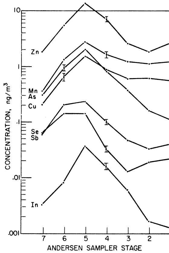
Figure V-1 Andersen Sample AR01 - M-Type Elements
