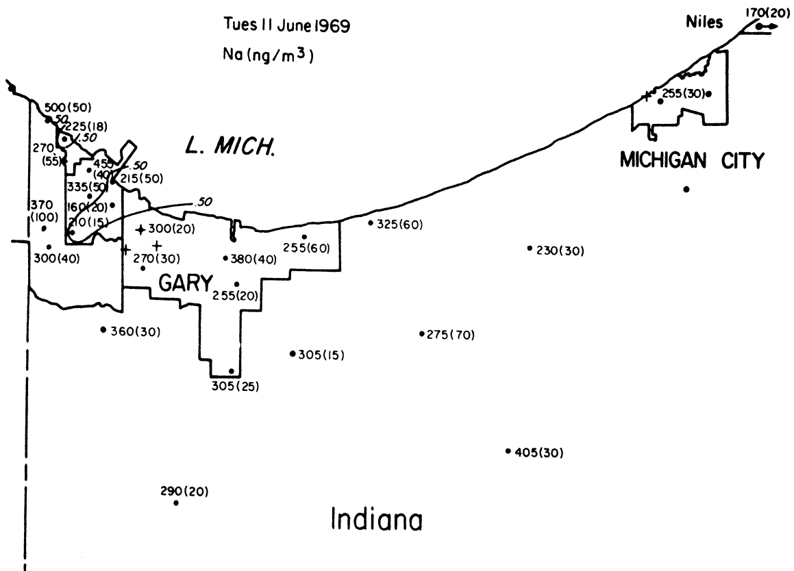
Figure VI-26 Concentration Distribution of Sodium
