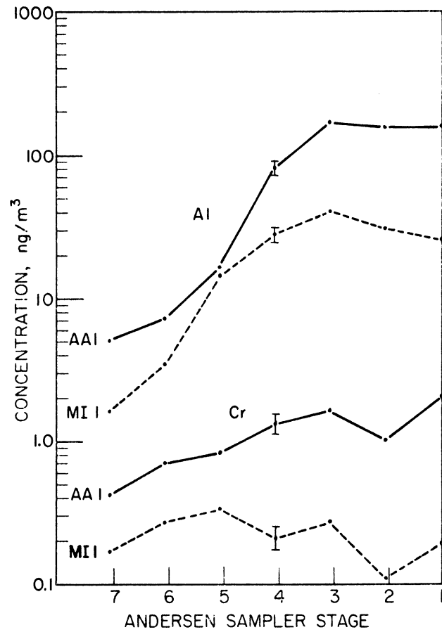
Figure IV-18 AAI - MI I Comparison - Al, Cr
