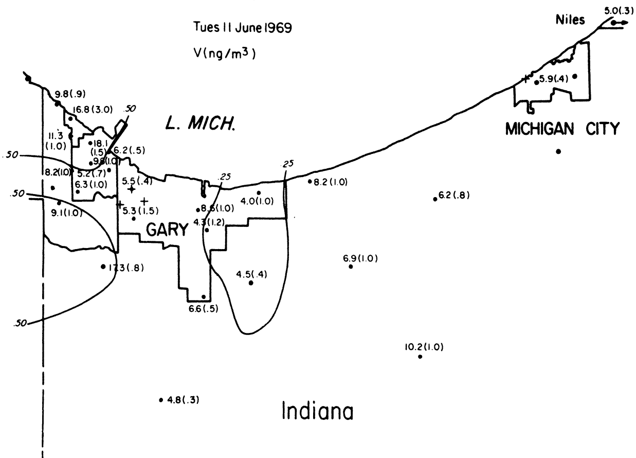
Figure VI-23 Concentration Distribution of Vanadium
