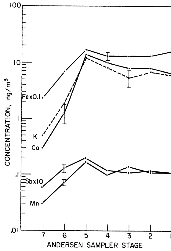
Figure IV-29 Andersen Sample TG2 - L-Type Elements
