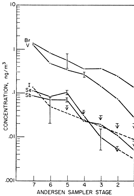
Figure V-6 Andersen Sample AR02 - S- and M-Type Elements
