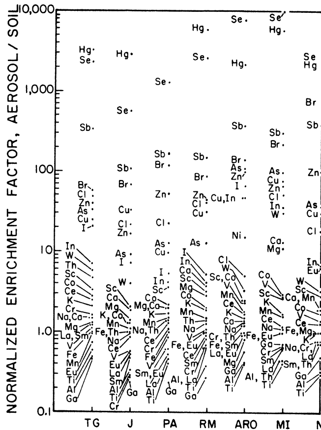
Figure III-14 Normalized Enrichment Factors, Canadian Summer Experiment
