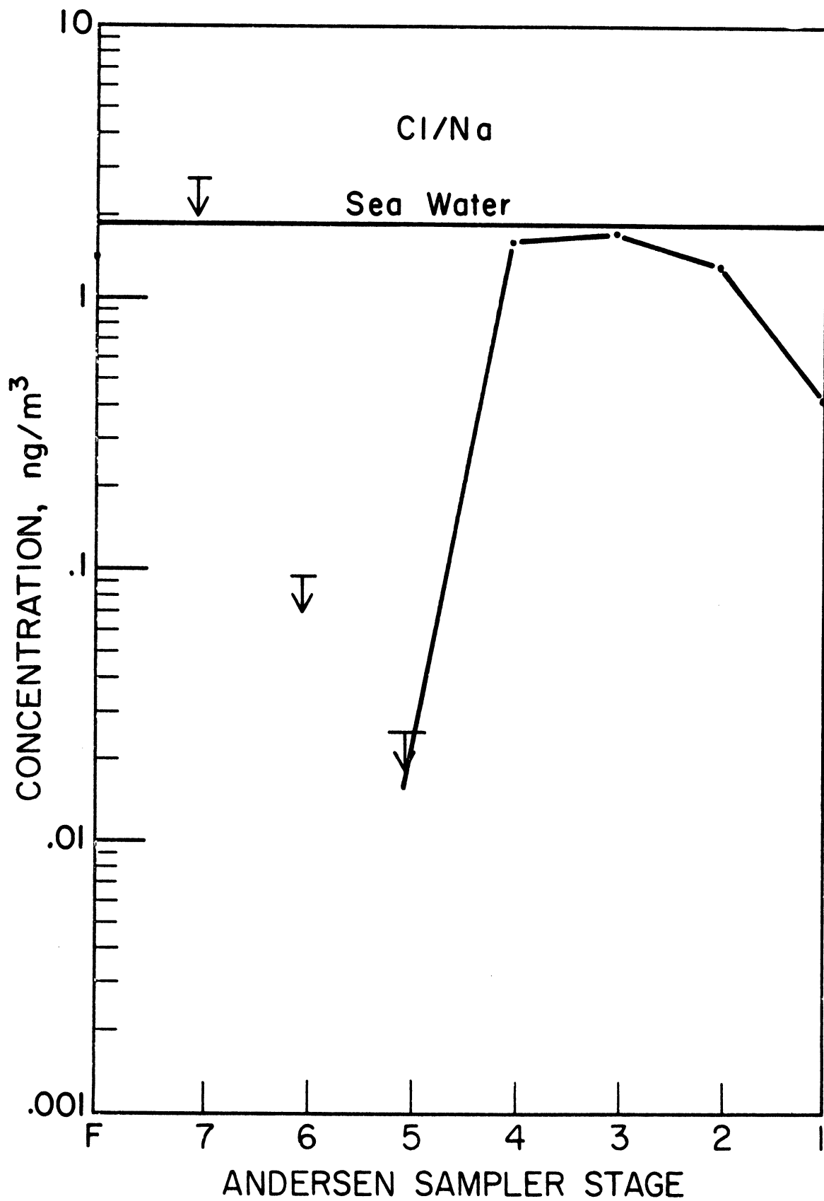
Figure IV-39 Cl/Na Ratios - TG3
