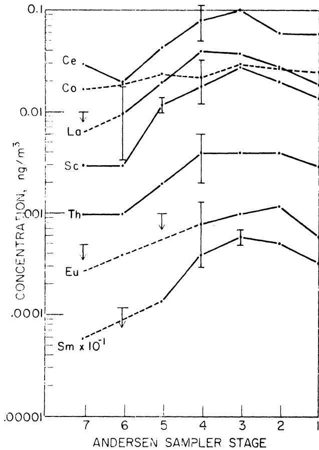
Figure IV-6 Andersen Sample M11 - L-Type Elements
