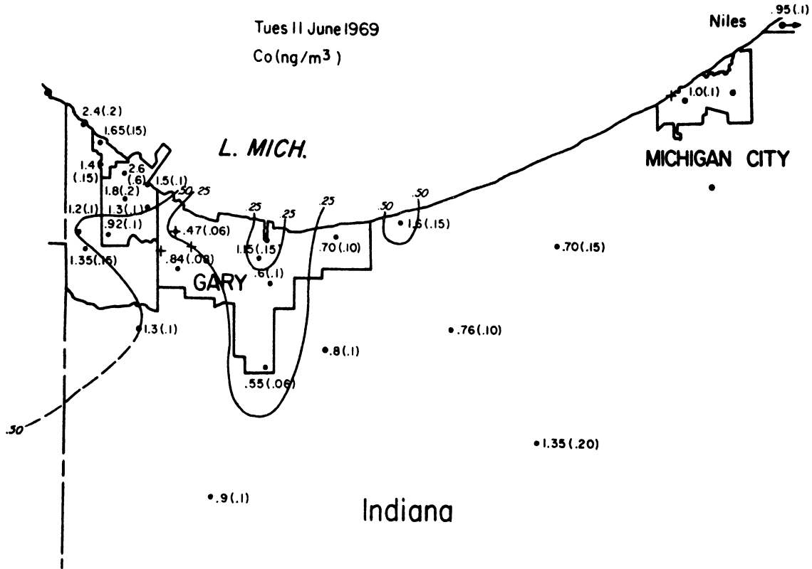
Figure VI-19 Concentration Distribution of Cobalt
