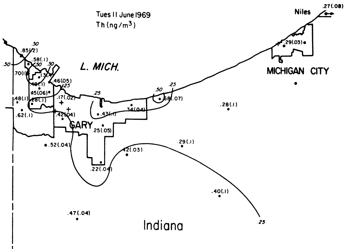
Figure VI-14 Concentration Distribution of Thorium
