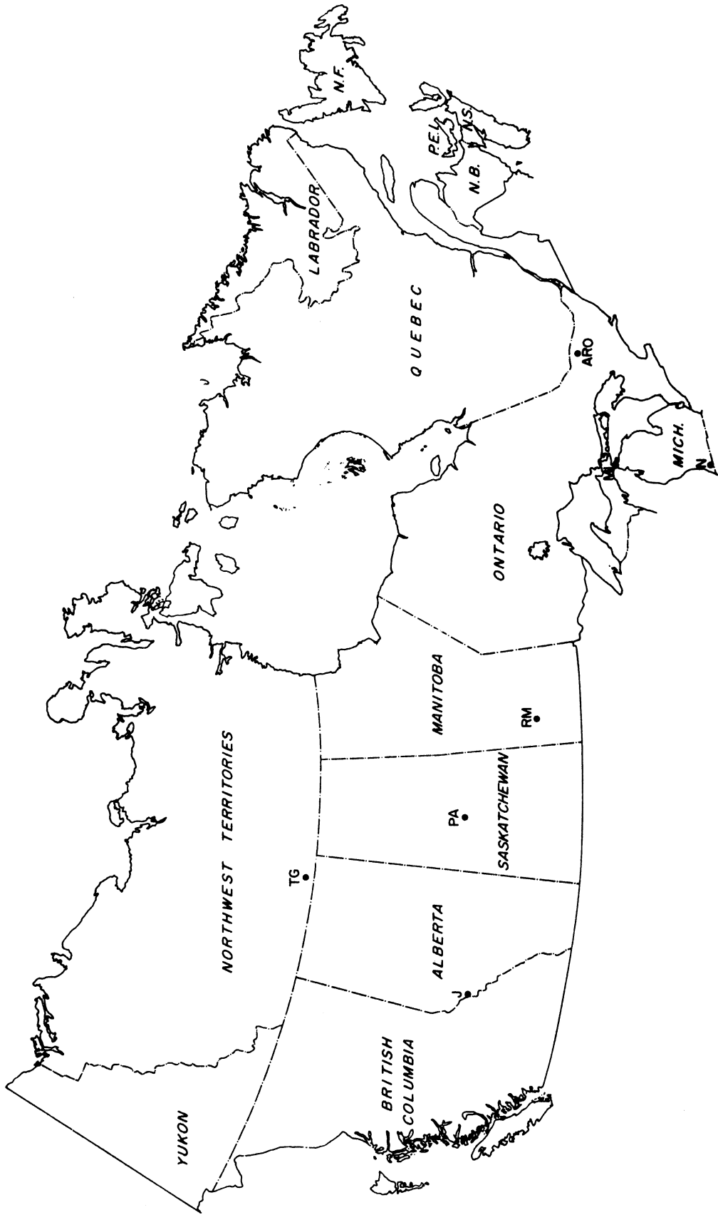
Figure II-2 Sampling Locations - Canadian Experiments
