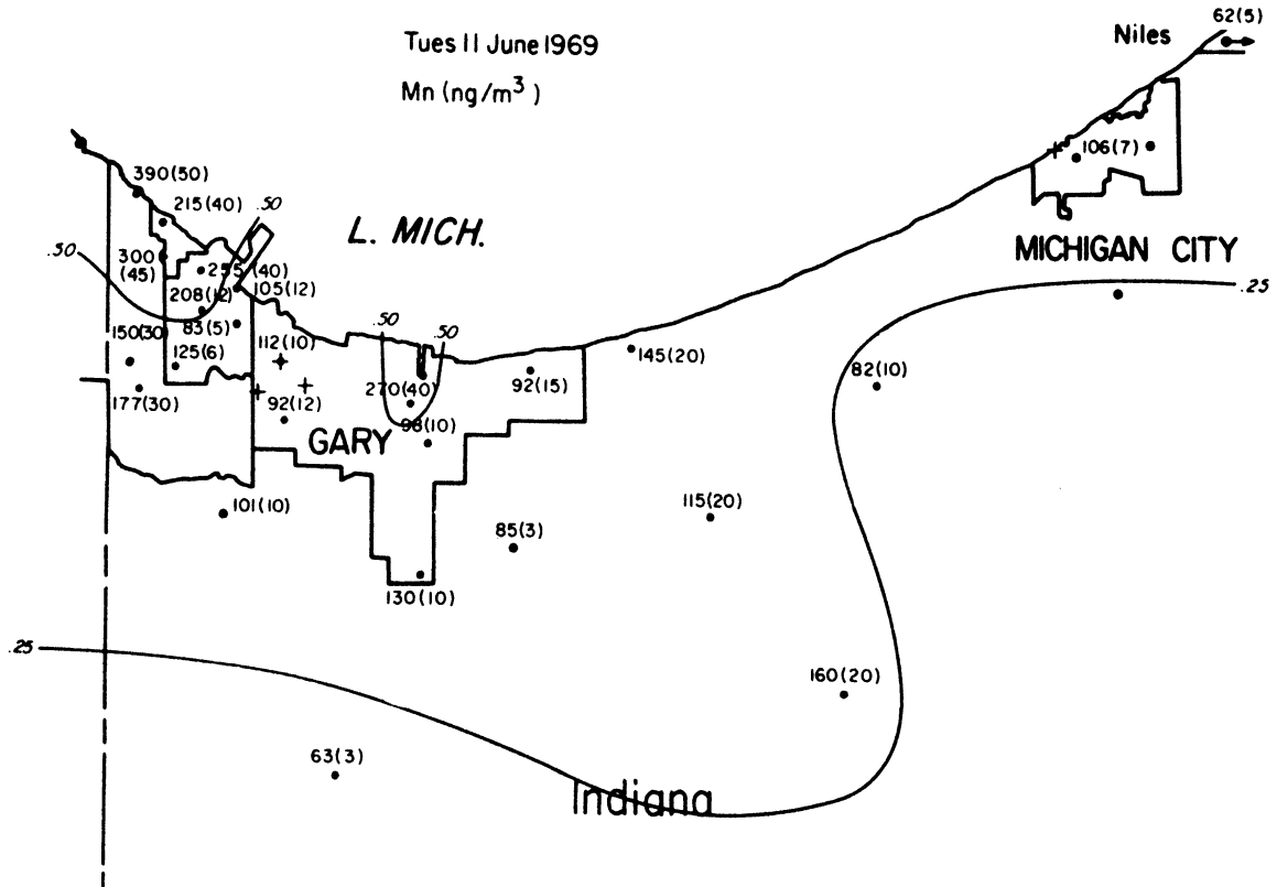
Figure VI-15 Concentration Distribution of Manganese
