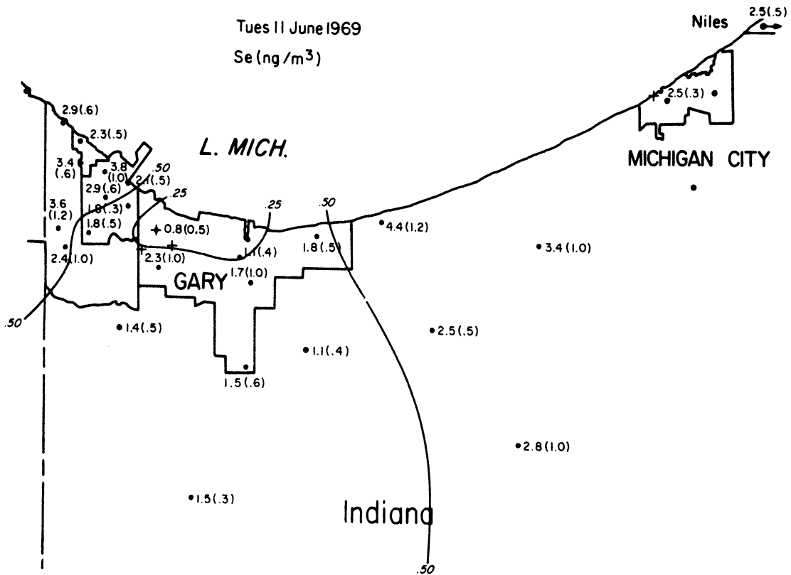
Figure VI-18 Concentration Distribution of Selenium
