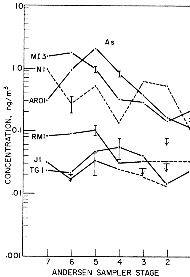
Figure III-11 Particle Size Distributions of As, Canadian Summer Experiment
