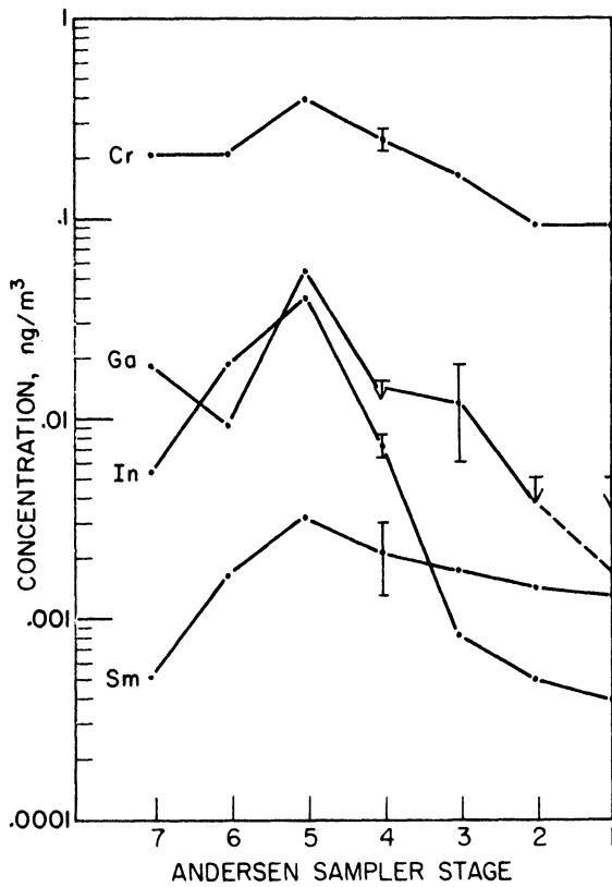
Figure V-4 Andersen Sample AR02 - M-Type Elements
