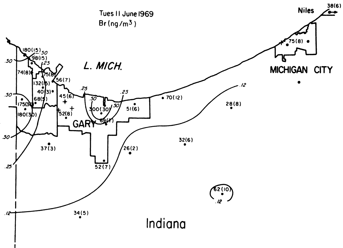
Figure VI-8 Concentration Distribution of Bromine
