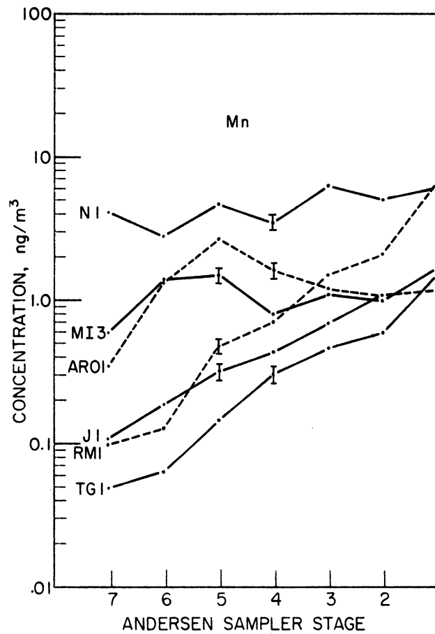
Figure III-10 Particle Size Distributions of Mn, Canadian Summer Experiment
