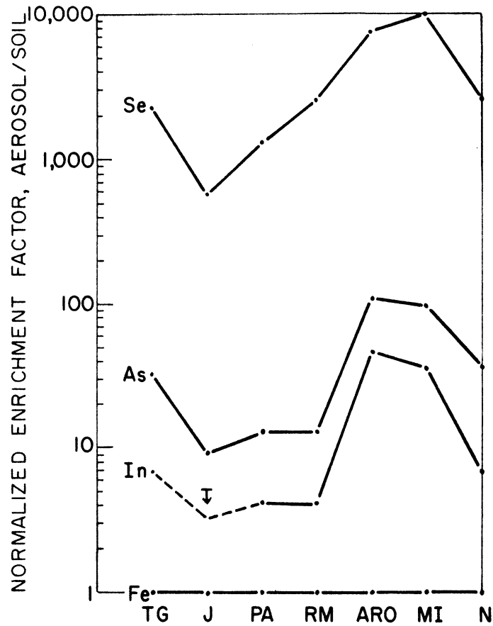
Figure III-19 Normalized Enrichment Factors, Canadian Summer Experiment
