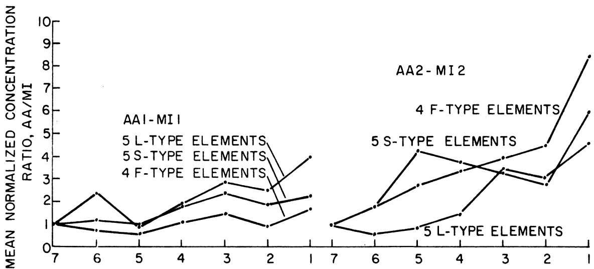
Figure IV-24 Mean Normalized Concentration Ratios by Subgroup, AA/MI
