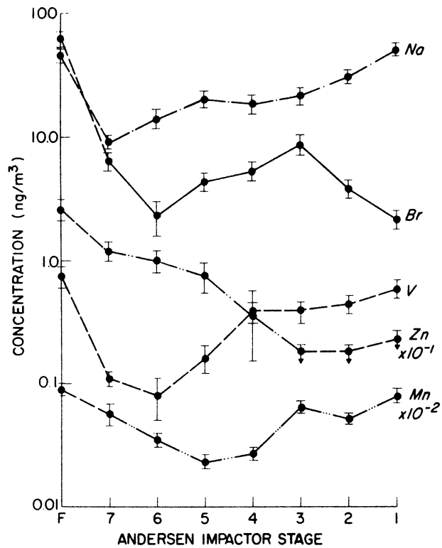
Figure VII-7 Particle Size Distribution of 5 Elements During Sampling
