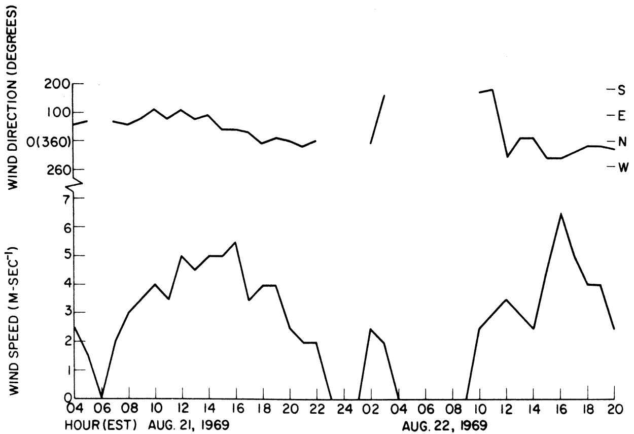
Figure VII-2 Wind Speed and Direction During Sampling
