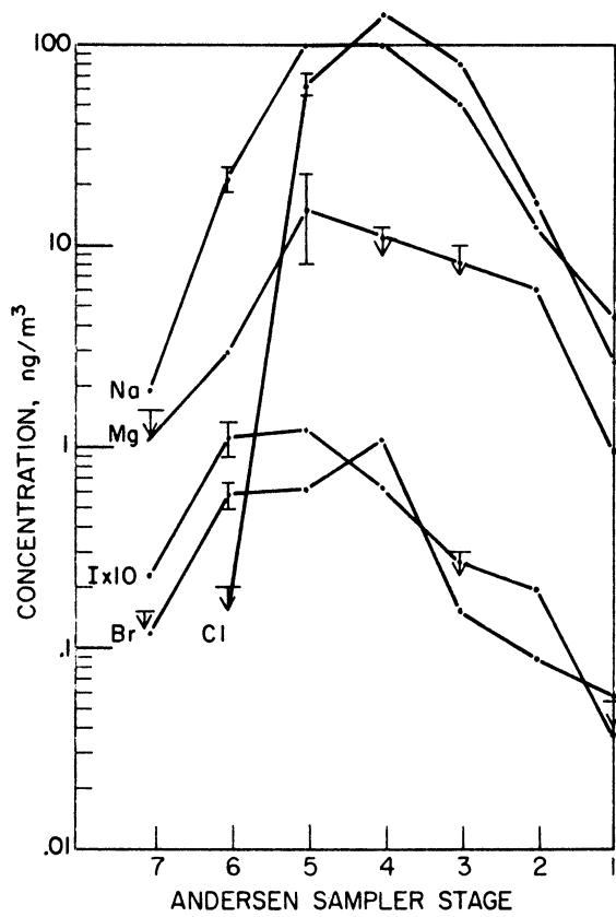
Figure IV-32 Andersen Sample TG2 - M-Type Elements
