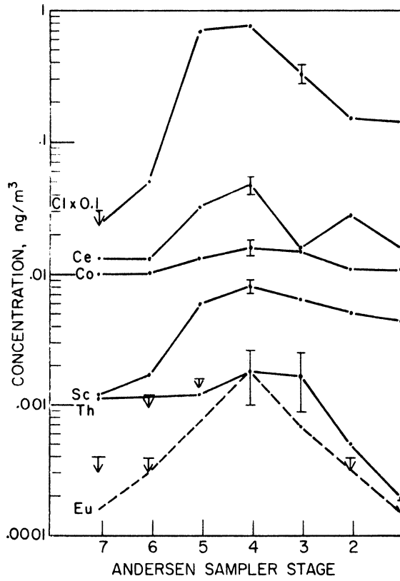
Figure V-5 Andersen Sample AR02 - M-Type Elements
