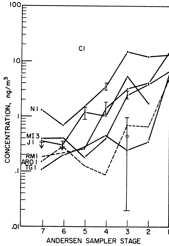
Figure IV-35 Cl Spectra - Canadian Summer Experiment
