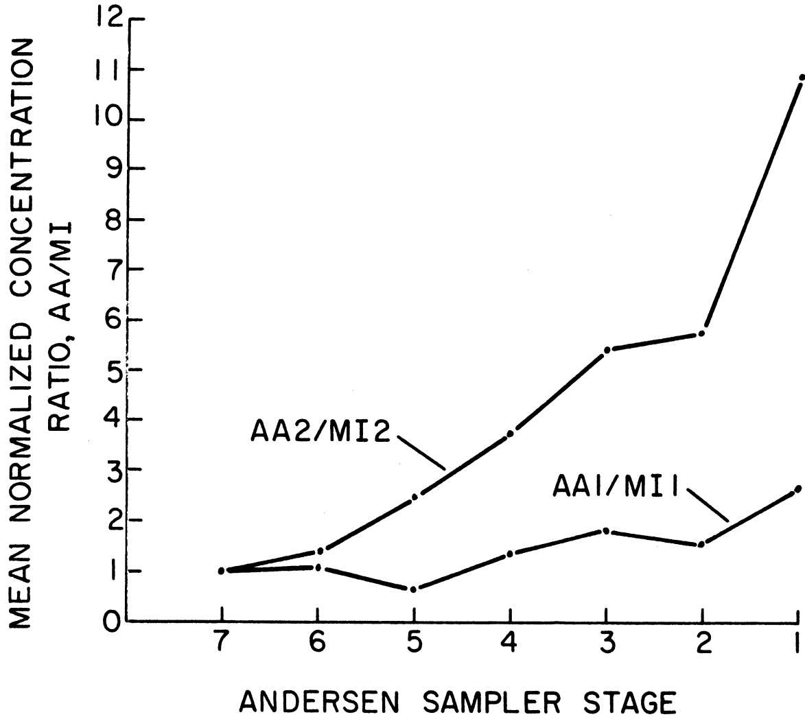
Figure IV-23 Mean Normalized Concentration Ratios, AA/MI
