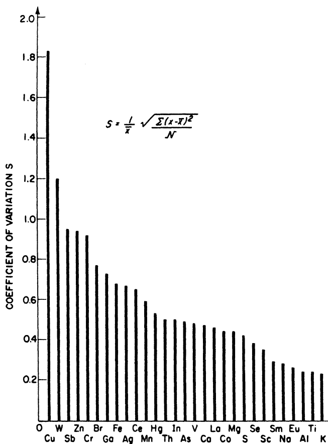
Figure VI-29 Coefficient of Variation
