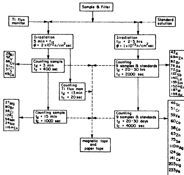
Figure 1. Irradiation-counting scheme
