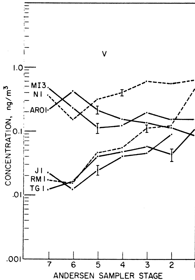
Figure III-8 Particle Size Distributions of V, Canadian Summer Experiment
