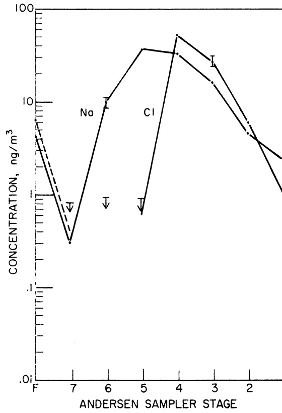
Figure IV-37 Na - Cl Comparison - TG3
