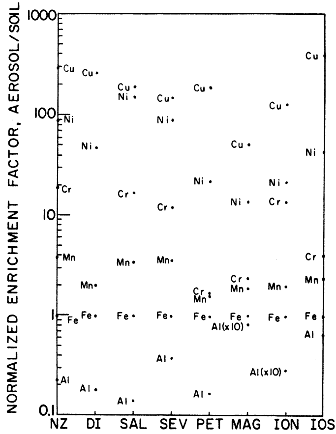
Figure III-15 Normalized Enrichment Factors, USSR
