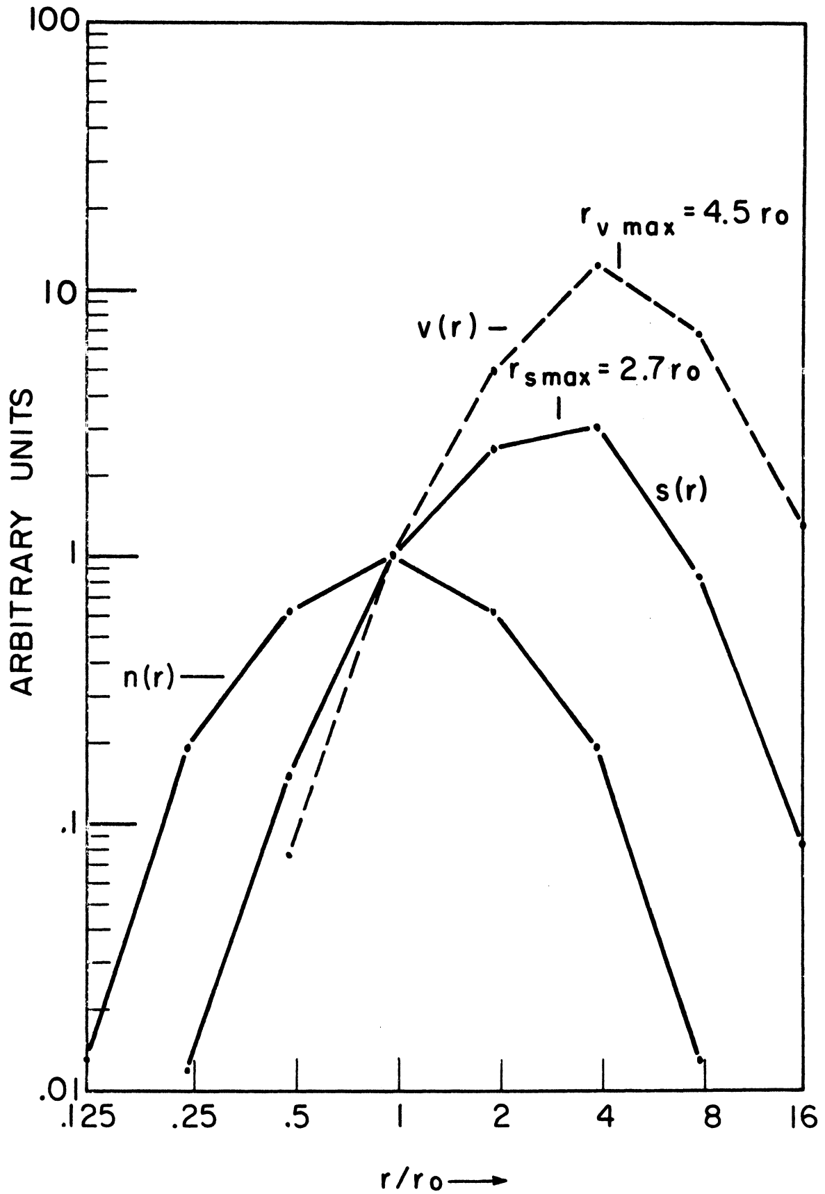
Figure V-7 Number, Surface, and Volume Distributions for a Log-Normal
