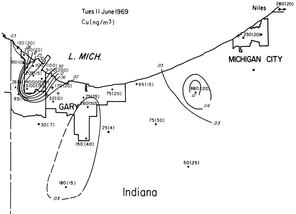
Figure VI-5 Concentration Distribution of Copper
