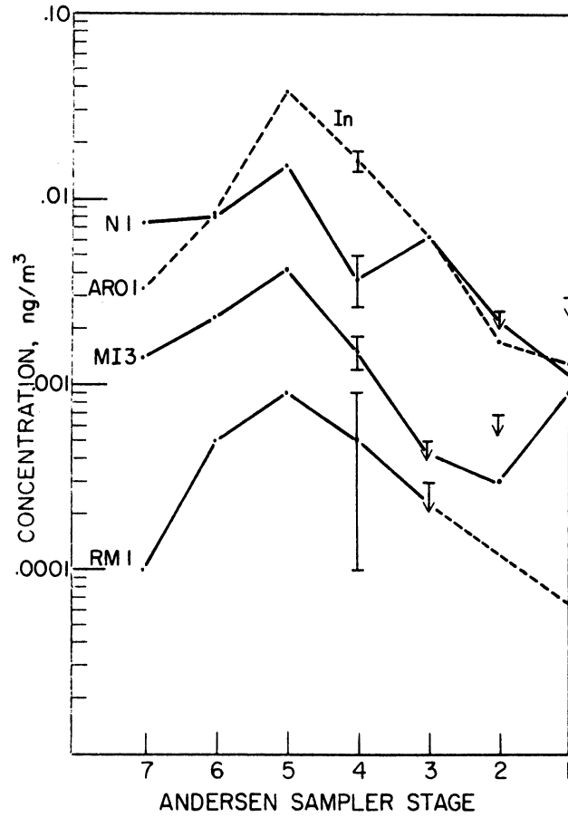
Figure III-5 Particle Size Distributions of In, Canadian Summer Experiment
