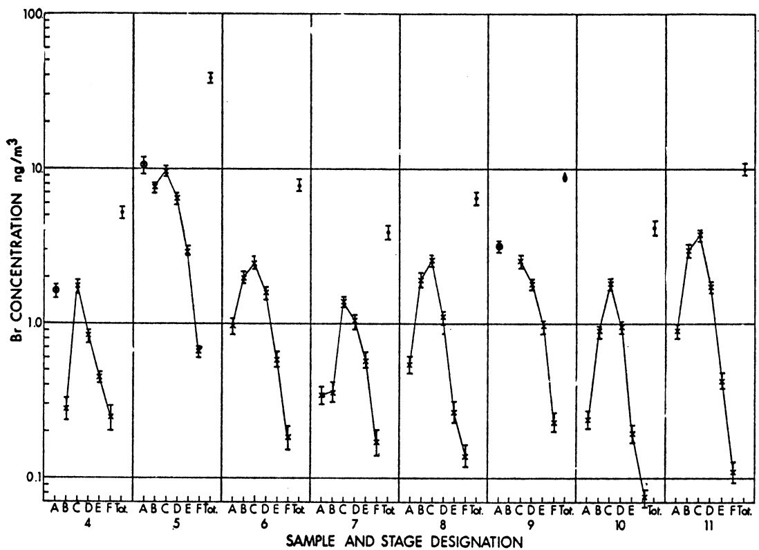
Figure IV-40 Cl and Br Particle Size Distributions in Fresh Marine
