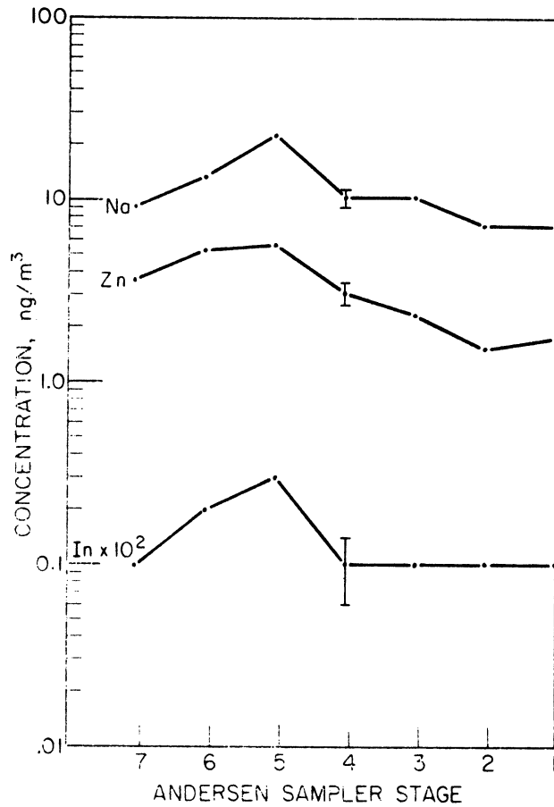
Figure IV-8 Andersen Sample M11 - M-Type Elements
