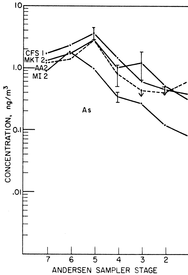
Figure IV-16 Mackinac Island - Ann Arbor - East Chicago Comparison - As
