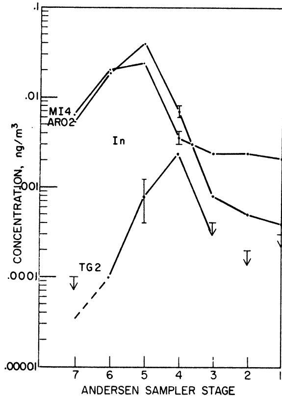
Figure IV-27 In Spectra - Canadian Winter Experiment
