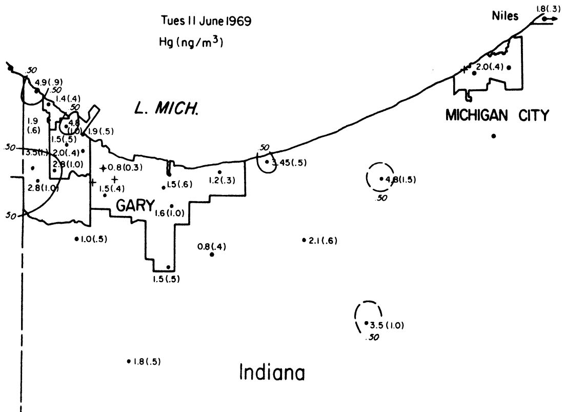
Figure VI-16 Concentration Distribution of Mercury
