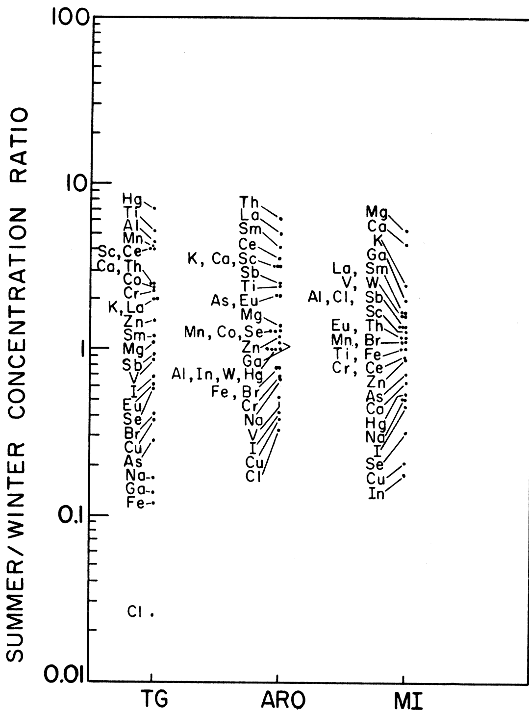
Figure III-21 Seasonal Concentration Ratios, TG, ARO, MI
