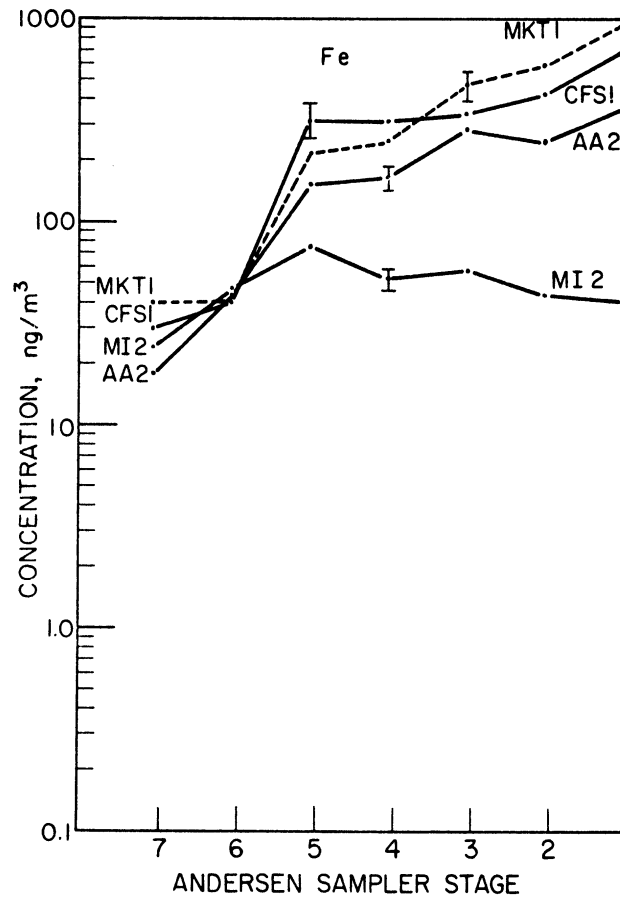
Figure IV-10 Mackinac Island - Ann Arbor - East Chicago Comparison - Fe
