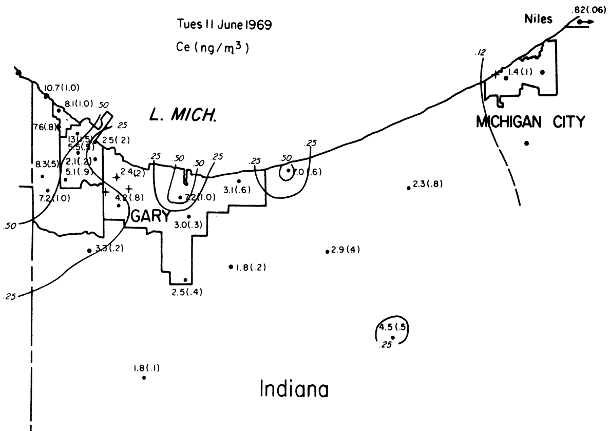
Figure VI-12 Concentration Distribution of Cerium
