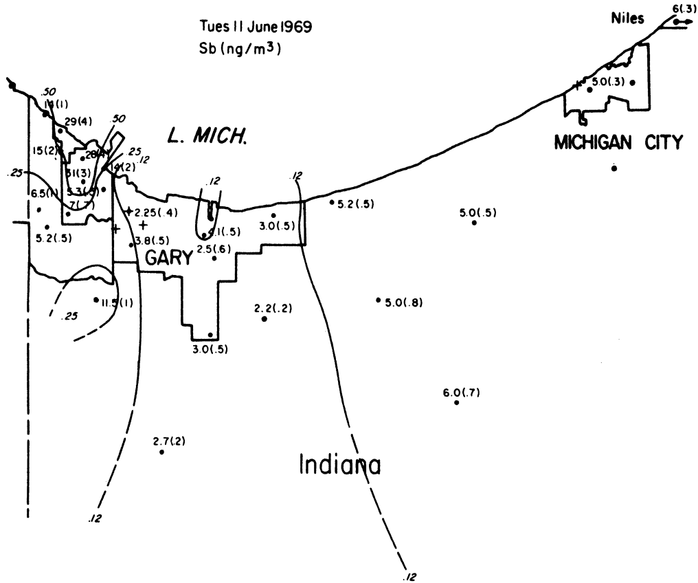
Figure VI-7 Concentration Distribution of Antimony
