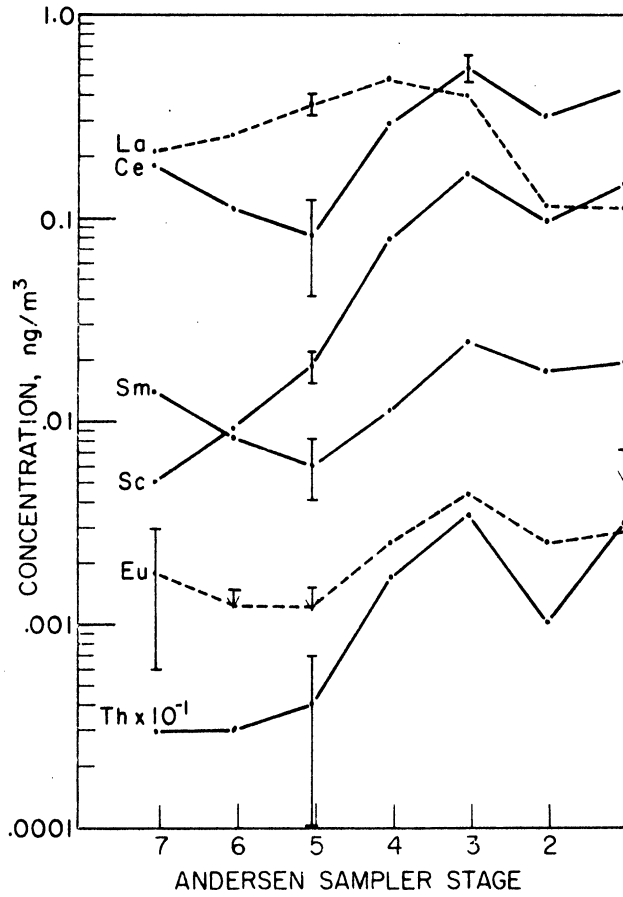
Figure IV-3 Andersen Sample AAl - L- and M-Type Elements
