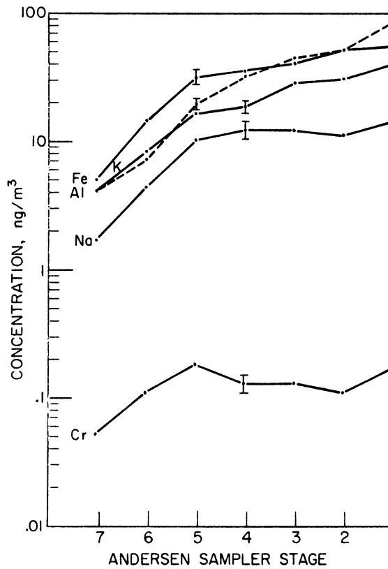
Figure V-2 Andersen Sample AR01 - L-Type Elements
