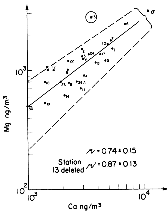
Figure VI-36 Concentration Correlation of Ca/Mg Over 24 Sampling Stations, Station 13 Deleted
