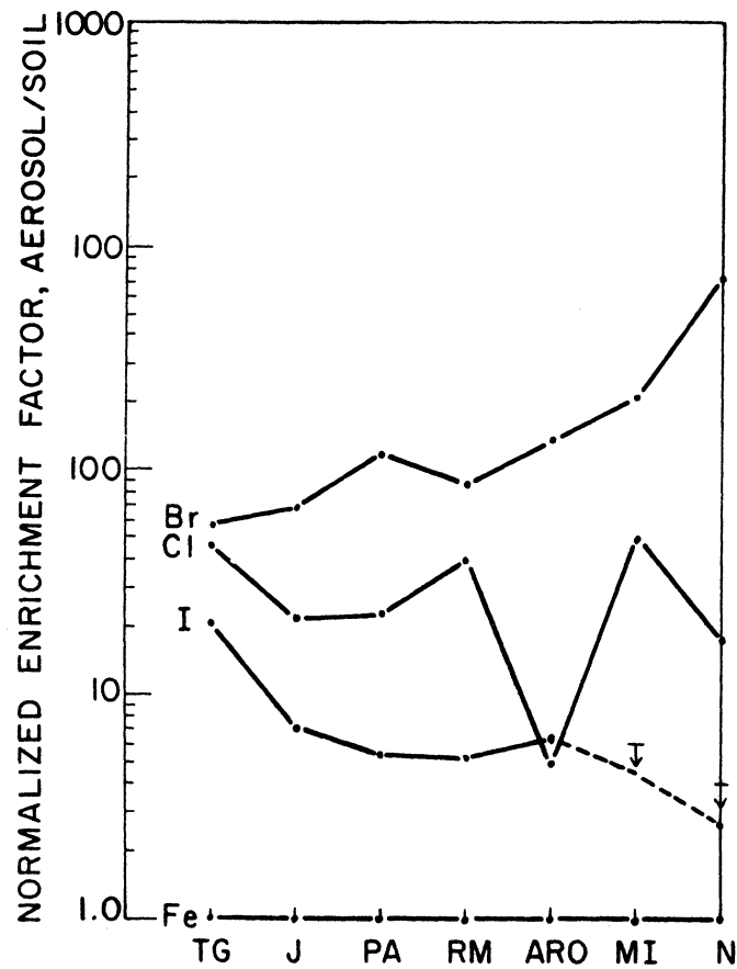
Figure III-17 Normalized Enrichment Factors, Canadian Summer Experiment
