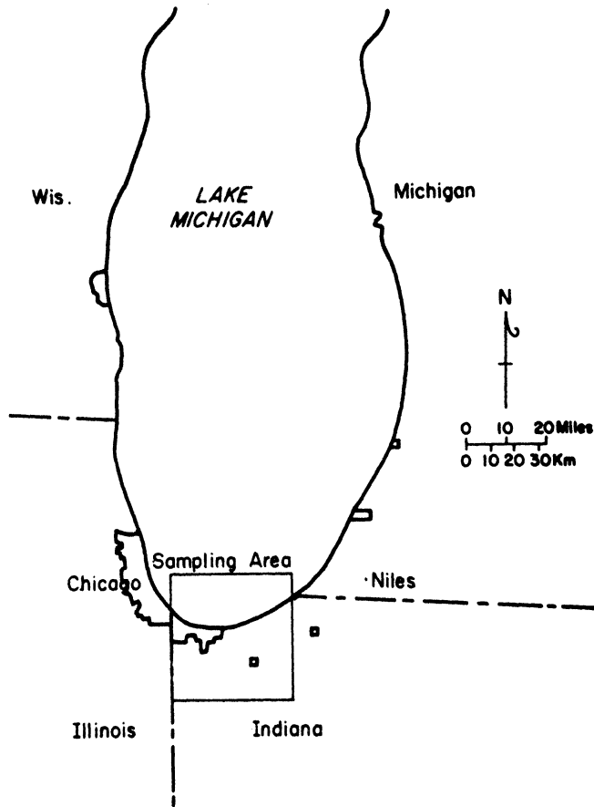
Figure VI-1 Map of Southern Lake Michigan
