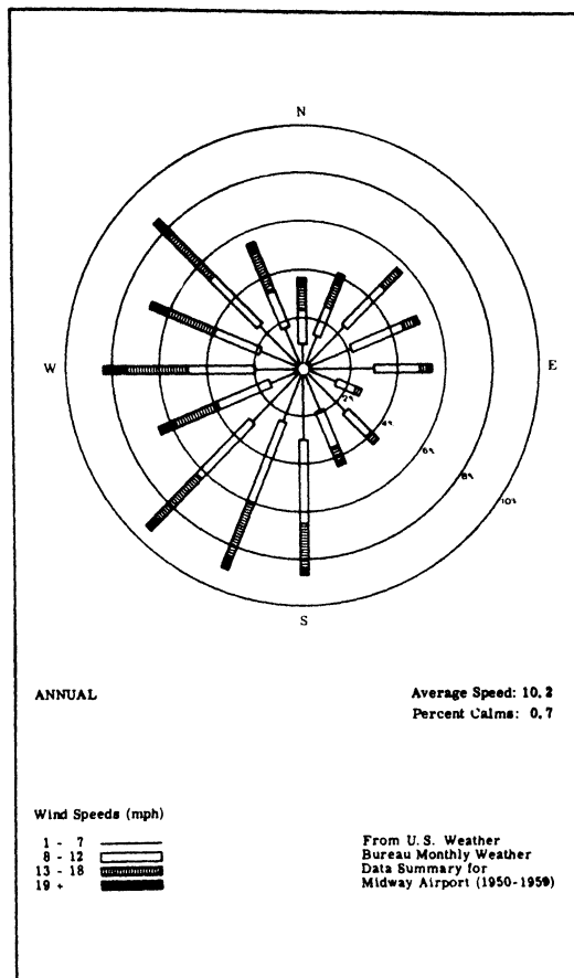
Figure VI-2 Wind Rose for the Chicago - Northwest Indiana Area
