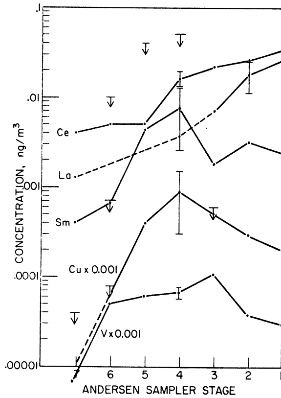
Figure IV-30 Andersen Sample TG2 - L- and M-Type Elements
