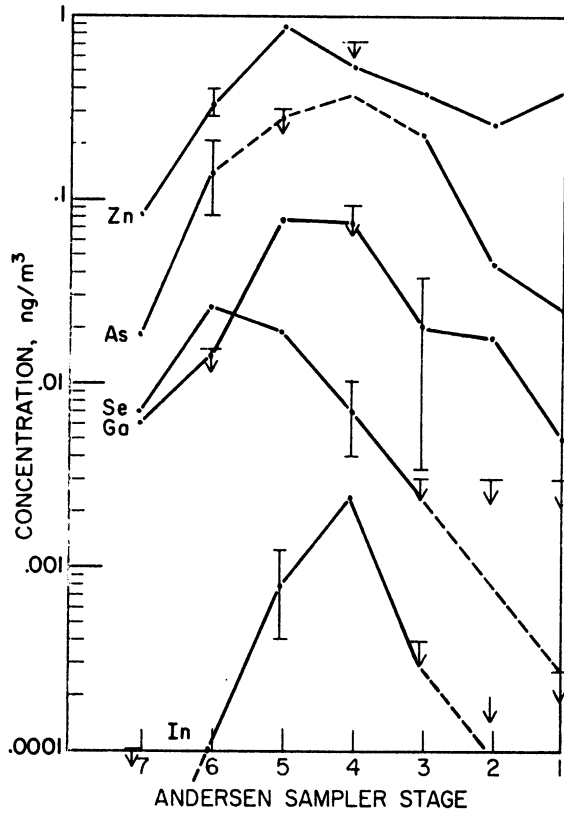
Figure IV-31 Andersen Sample TG2 - M-Type Elements
