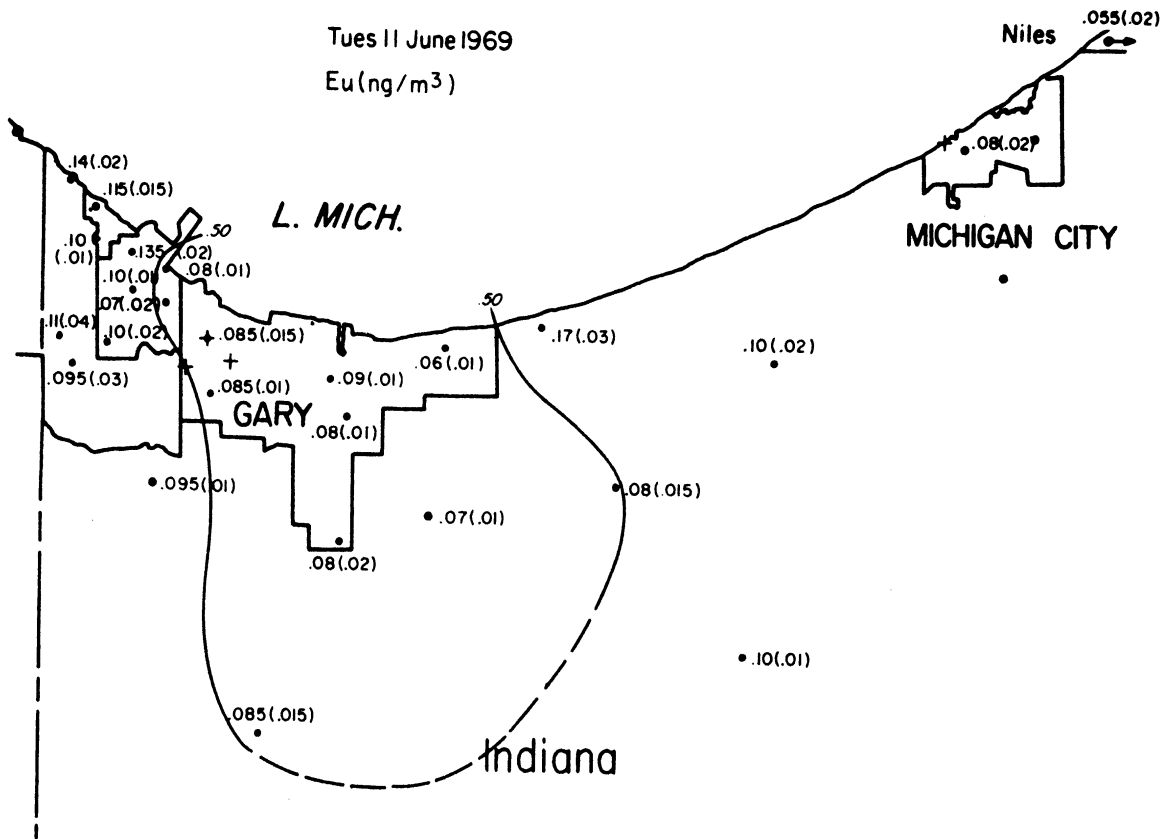
Figure VI-25 Concentration Distribution of Europium
