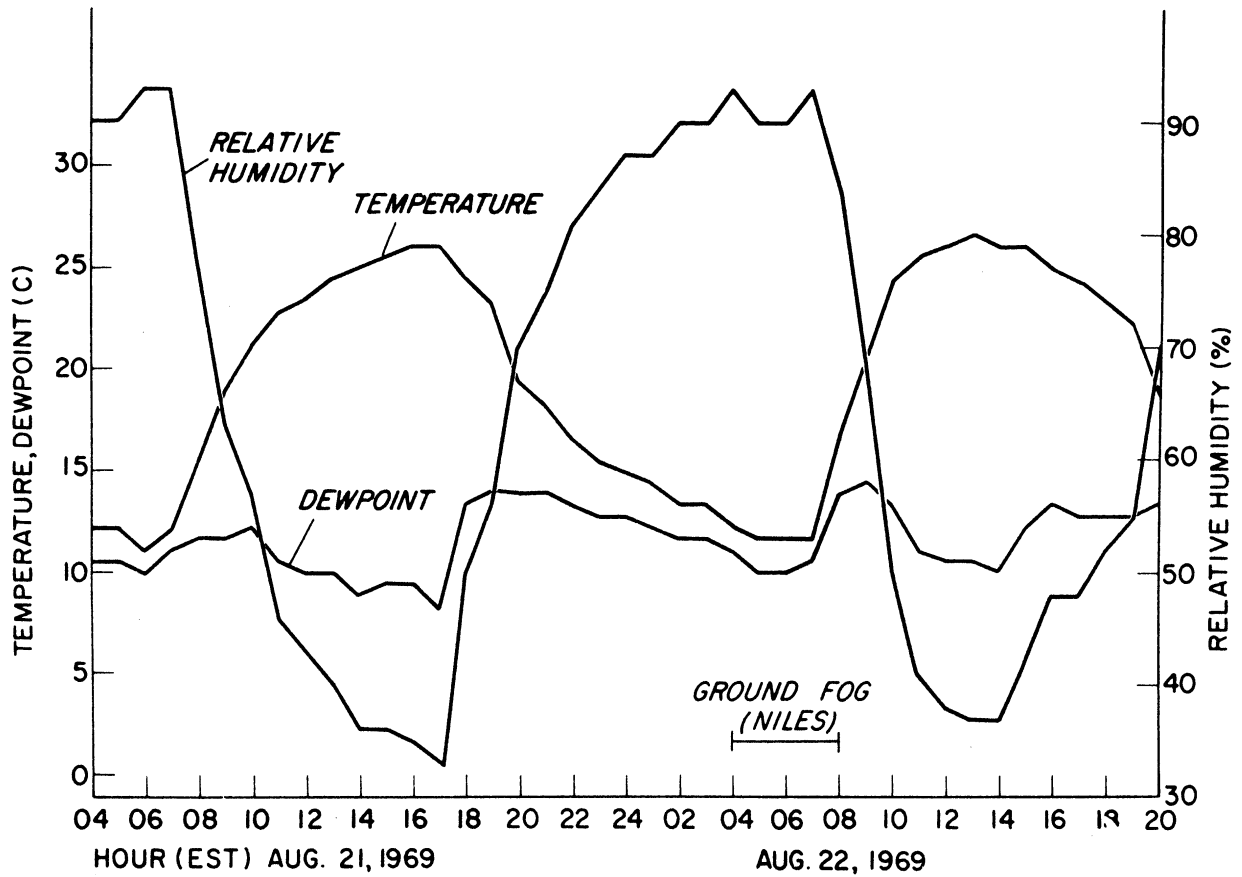
Figure VII-1 Relative Humidity, Temperature, and Dewpoint During Sampling
