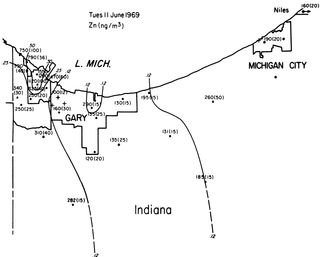
Figure VI-6 Concentration Distribution of Zinc
