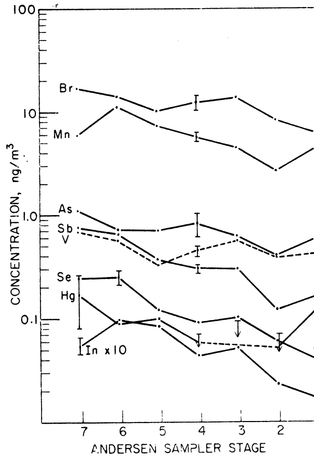
Figure IV-4 Andersen Sample AAl - S- and M-Type Elements
