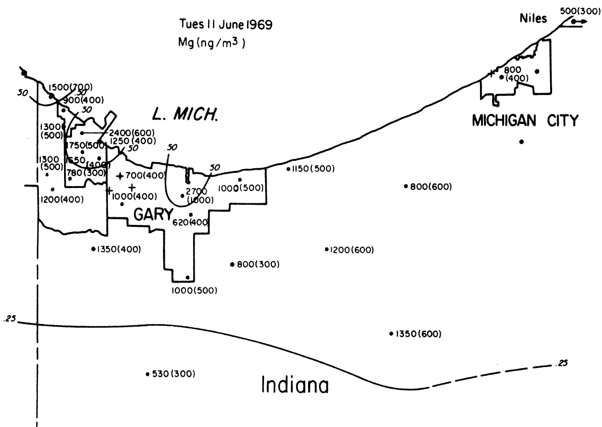
Figure VI-21 Concentration Distribution of Magnesium
