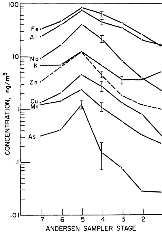
Figure V-3 Andersen Sample AR02 - M-Type Elements
