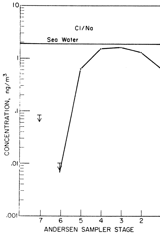
Figure IV-38 Cl/Na Ratios - TG2
