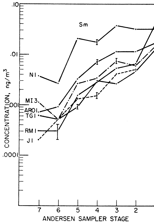
Figure III-4 Particle Size Distributions of Sm, Canadian Summer Experiment
