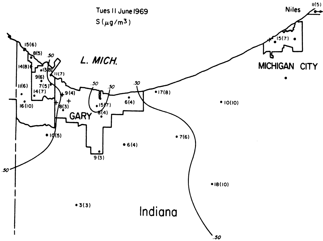
Figure VI-17 Concentration Distribution of Sulfur
