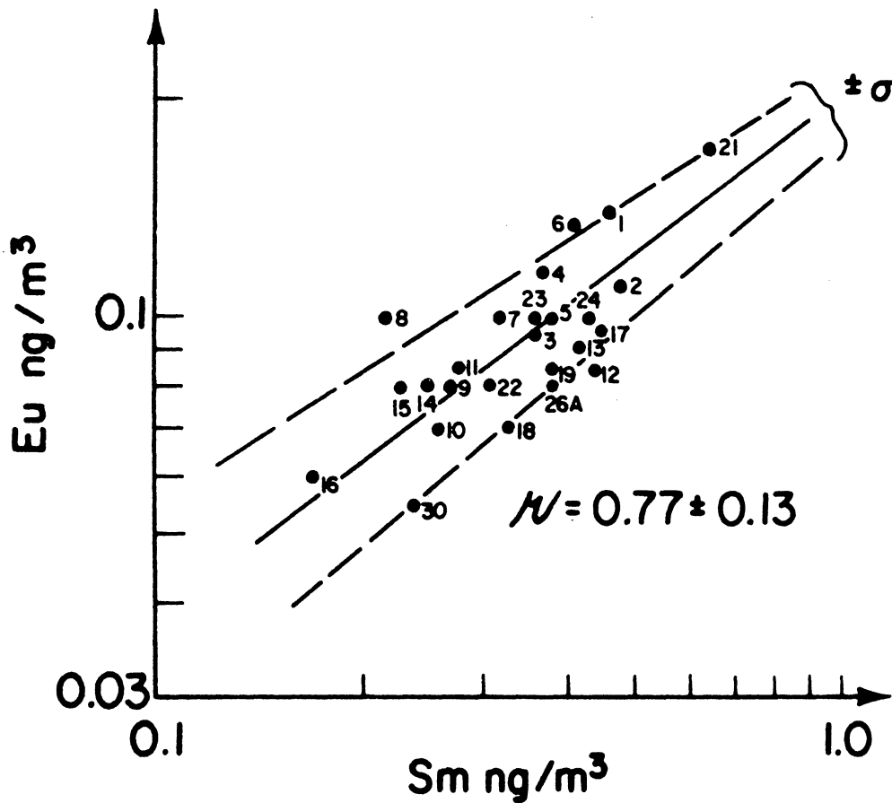
Figure VI-34 Concentration Correlation of Sm/Eu Over All 25 Sampling Stations
