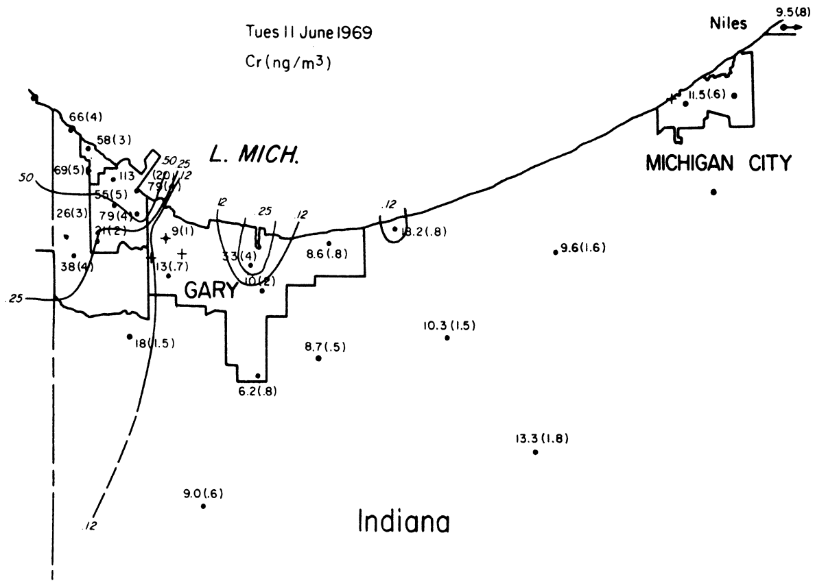
Figure VI-11 Concentration Distribution of Chromium
