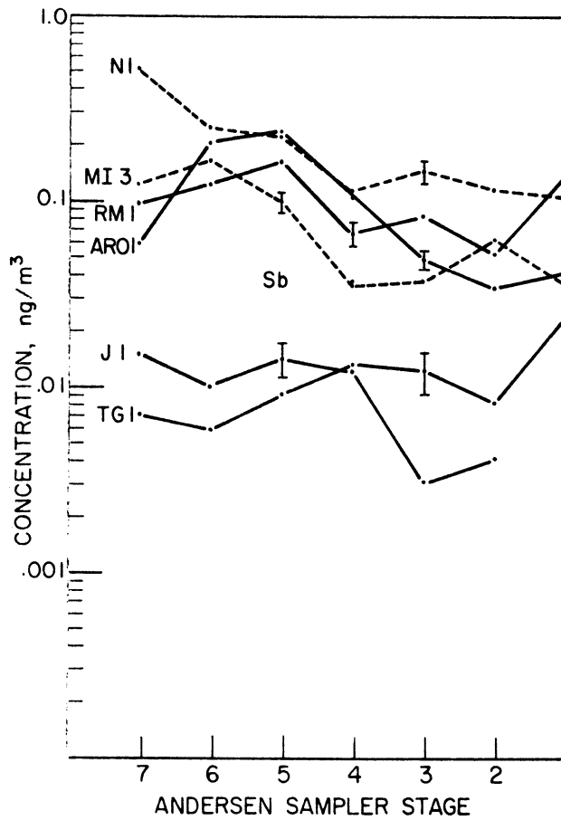
Figure III-7 Particle Size Distributions of Sb, Canadian Summer Experiment
