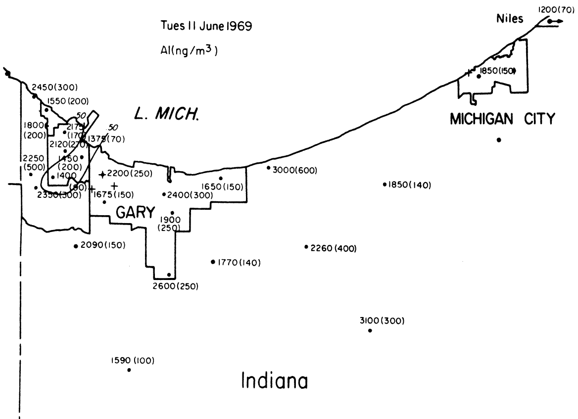
Figure VI-28 Concentration Distribution of Aluminum
