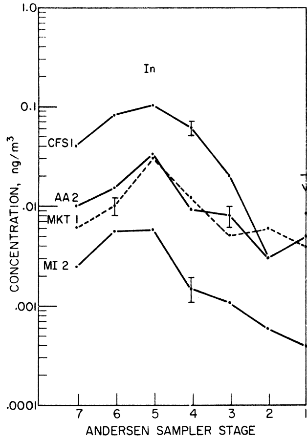
Figure IV-17 Mackinac Island - Ann Arbor - East Chicago Comparison - In
