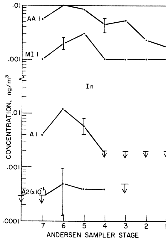
Figure IV-26 Miscellaneous In Spectra
