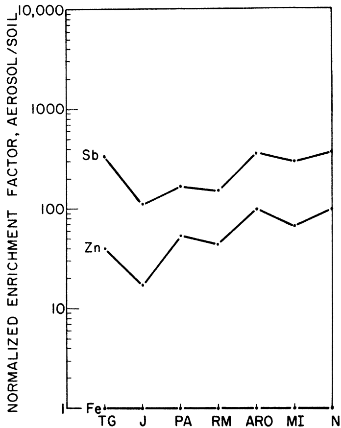
Figure III-20 Normalized Enrichment Factors, Canadian Summer Experiment
