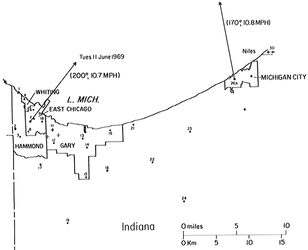
Figure VI-3 Map of Sampling Area with Numbers and Locations of Sampling Sites and Wind Direction for 11 June 1969
