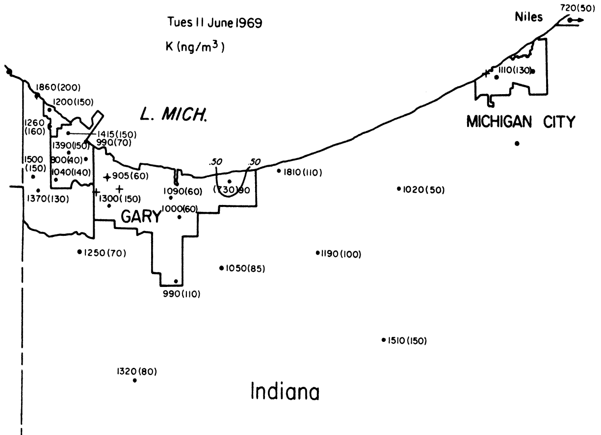
Figure VI-27 Concentration Distribution of Potassium
