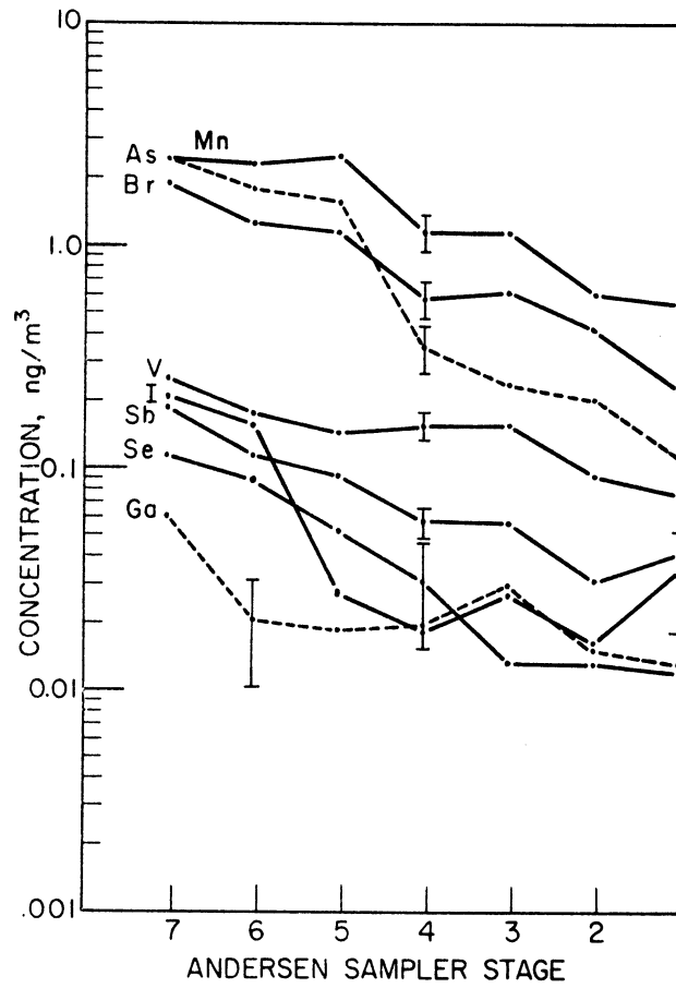
Figure IV-9 Andersen Sample MI1 - S-Type Elements
