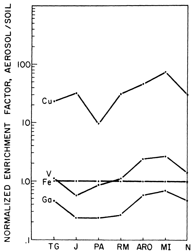
Figure III-18 Normalized Enrichment Factors, Canadian Summer Experiment
