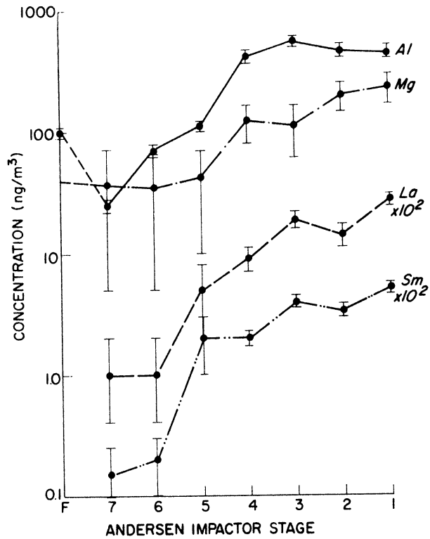
Figure VII-6 Particle Size Distribution of 4 Elements During Sampling
