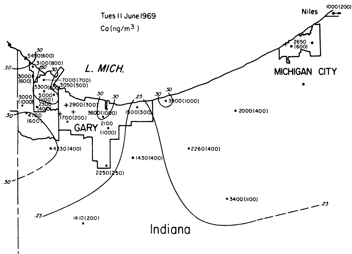
Figure VI-22 Concentration Distribution of Calcium
