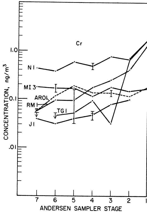
Figure III-13 Particle Size Distributions of Cr, Canadian Summer Experiment
