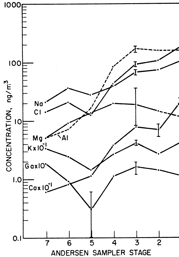
Figure IV-2 Andersen Sample AAl - L-Type Elements
