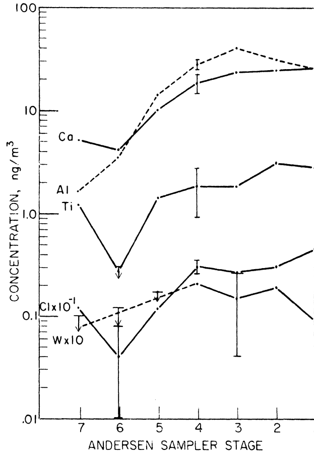
Figure IV-5 Andersen Sample M11 - L-Type Elements
