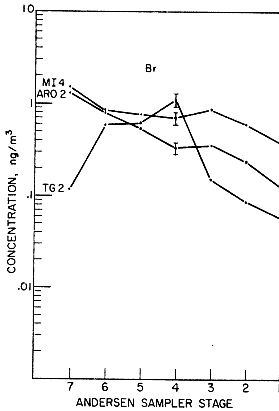
Figure IV-25 Br Spectra - Canadian Winter Experiment
