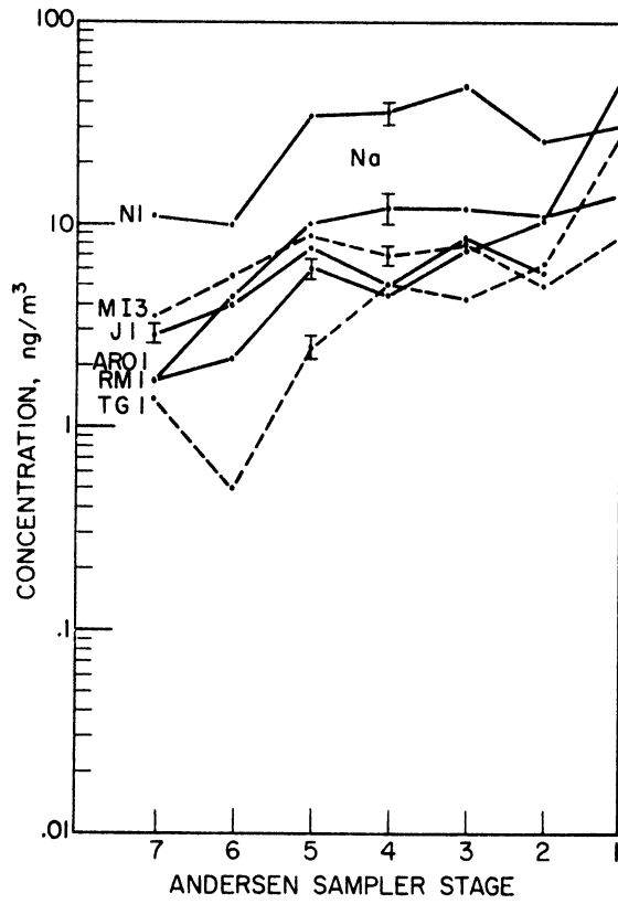
Figure IV-33 Na Spectra - Canadian Summer Experiment
