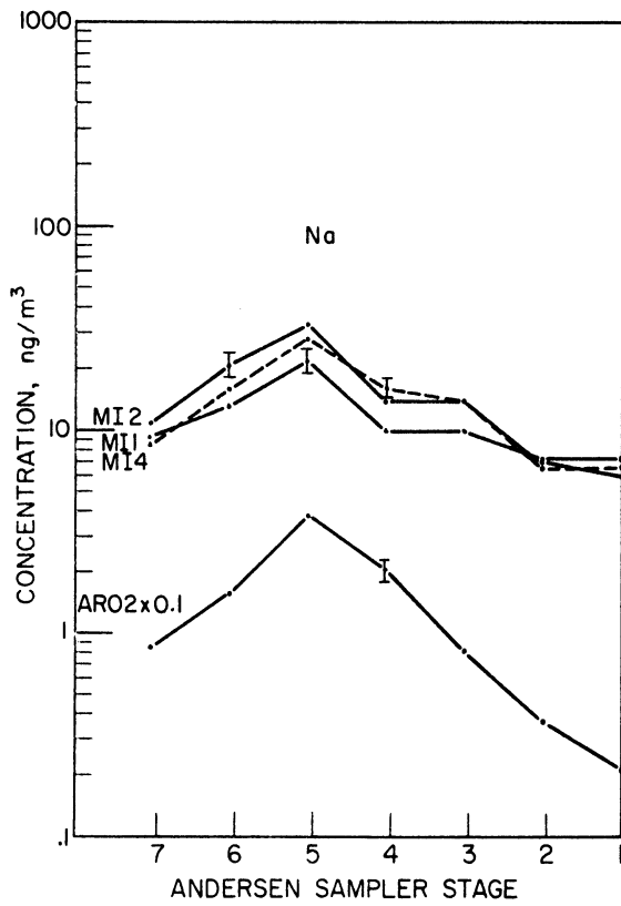
Figure IV-34 Na Spectra - Winter Samples
