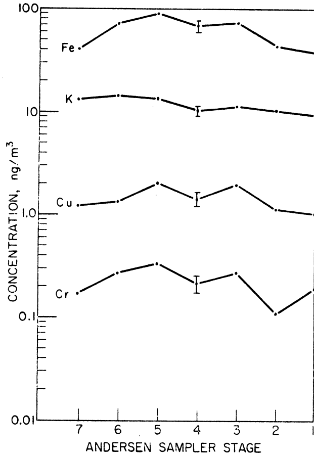
Figure IV-7 Andersen Sample M11 - F- and M-Type Elements
