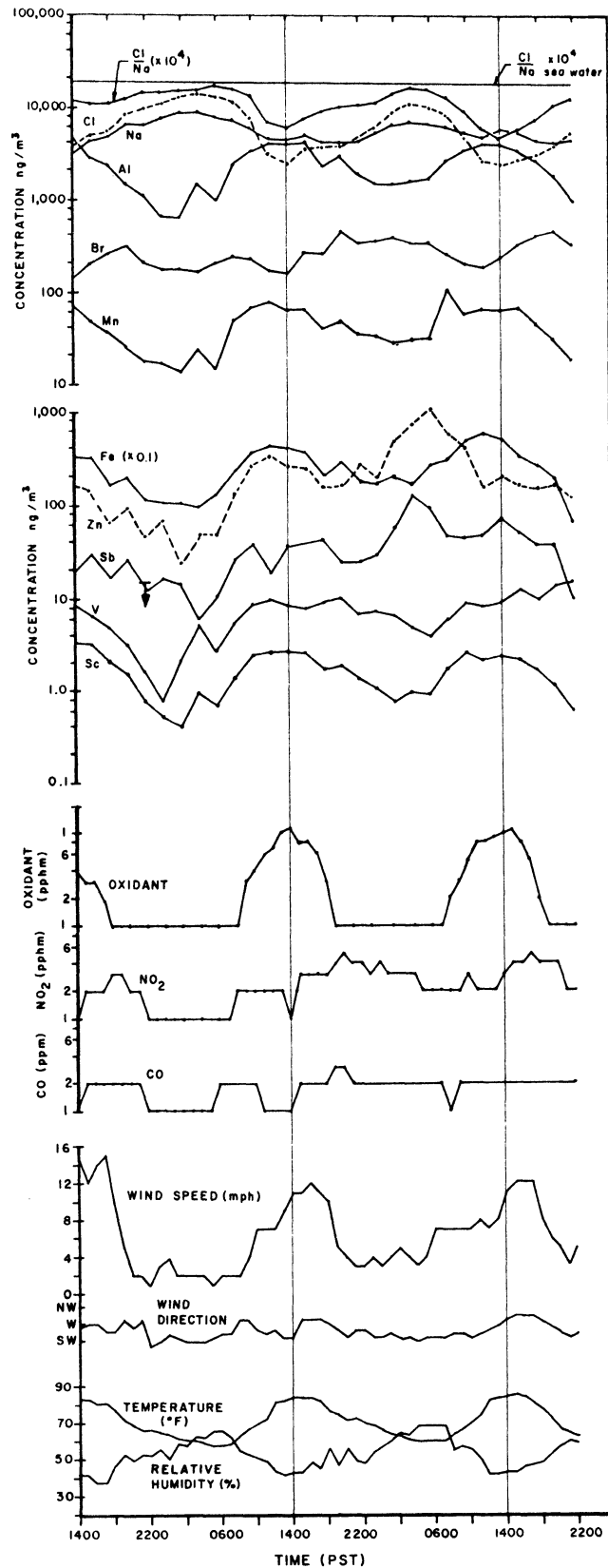
Figure VIII-1 Results of Measurements of Diurnal Variations of Aerosol
