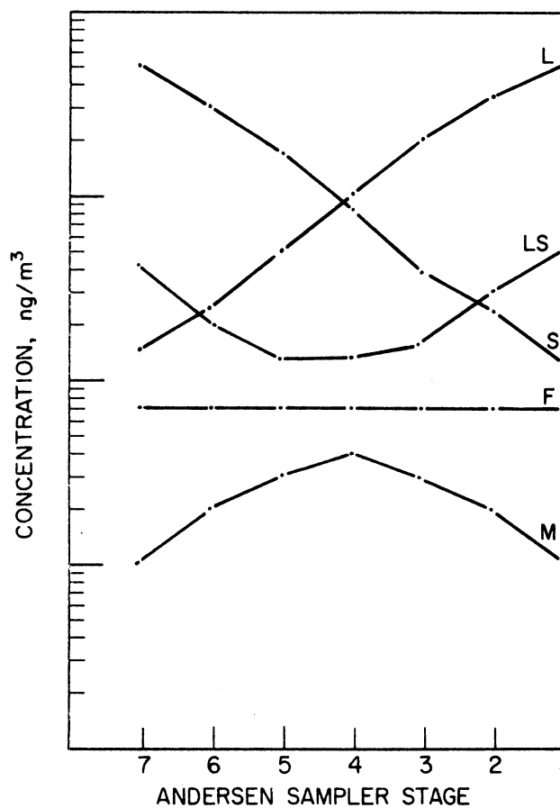
Figure III-1 Idealized Particle Size Distribution Shapes
