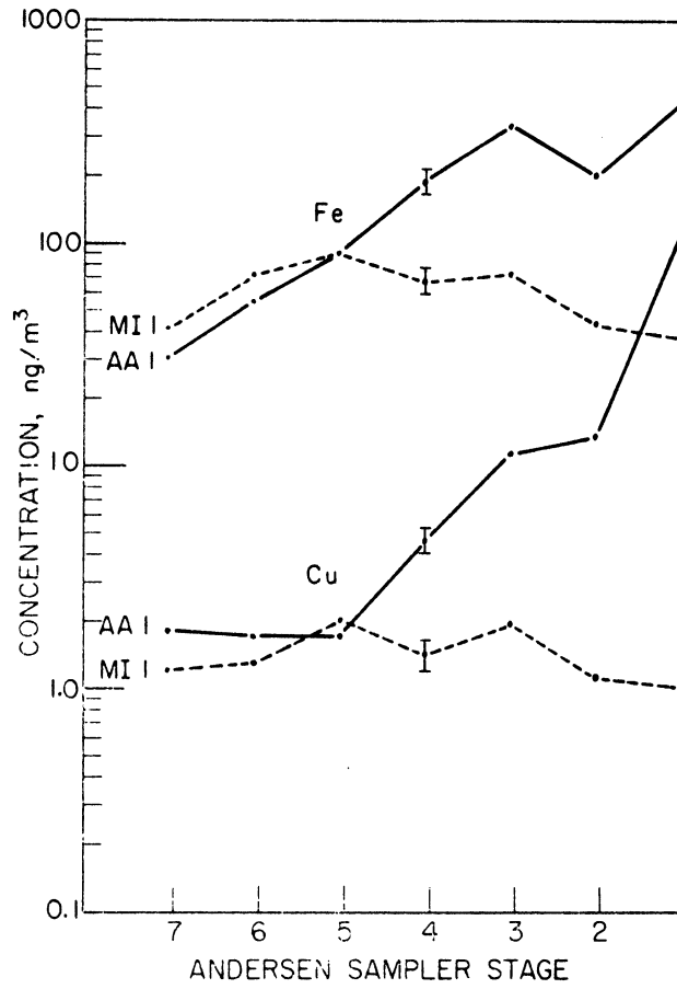
Figure IV-19 AAI - MII Comparison - Fe, Cu
