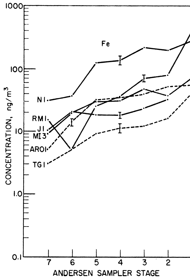
Figure III-3 Particle Size Distributions of Fe, Canadian Summer Experiment
