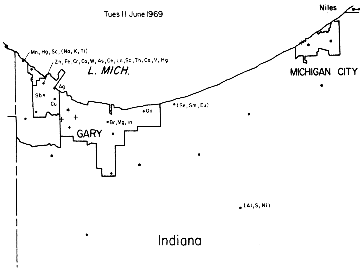
Figure VI-30 Locations of Maximum Concentrations of the Elements
