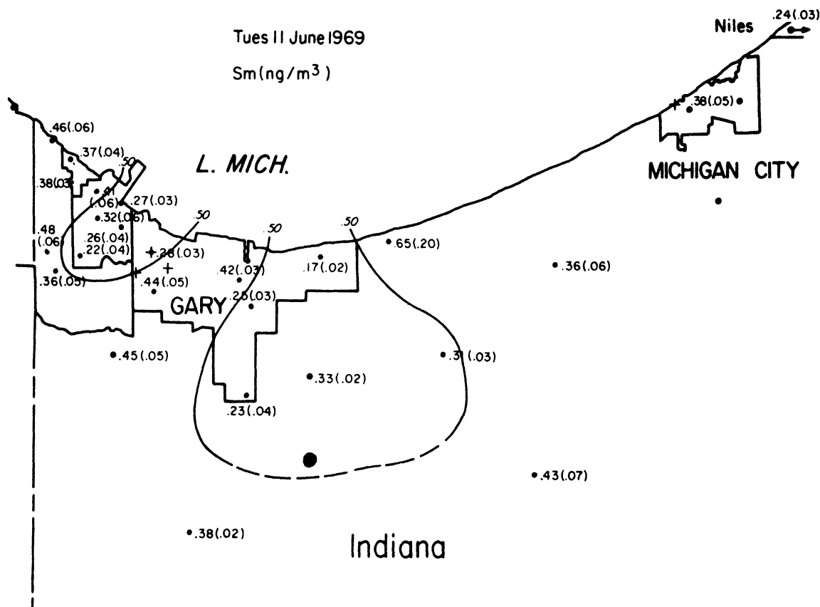
Figure VI-24 Concentration Distribution of Samarium
