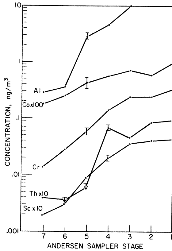
Figure IV-28 Andersen Sample TG2 - L-Type Elements
