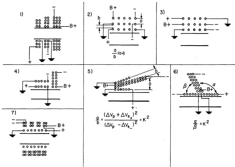
Fig. 3.11. Winding configurations.
