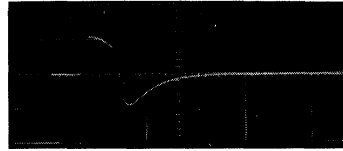
(b) Plate waveform 100 volts/major division 100 \mu sec/major division
