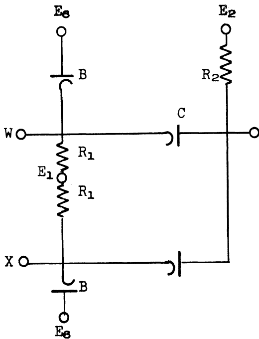
Typical "and" gate W \cdot X
