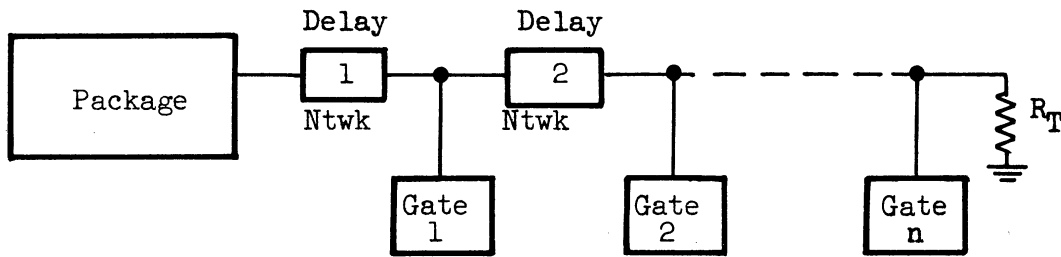
Fig. 4.2. Interconnection through singly terminated cable.
