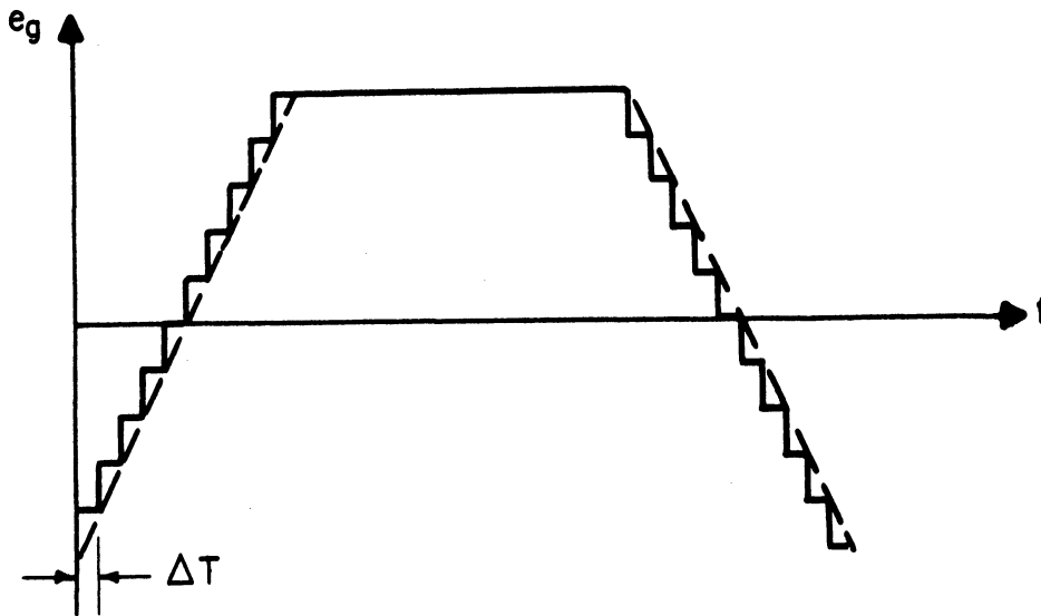
Fig. 1.13. Approximation of a waveform by steps.
