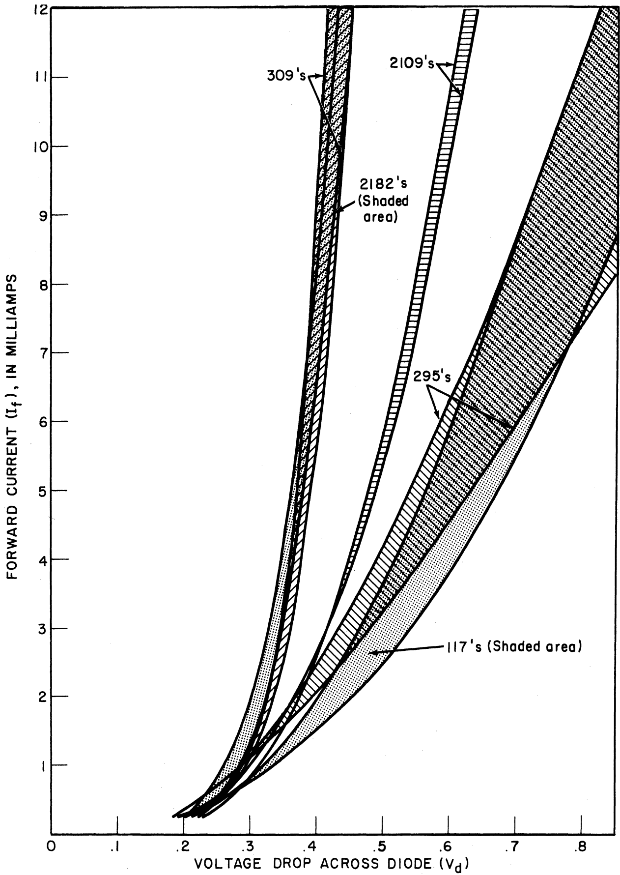
Fig. 2.6. Deviation of static characteristics.
