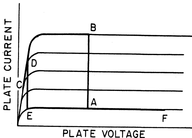
Fig. 1.1. Pentode operating path.
