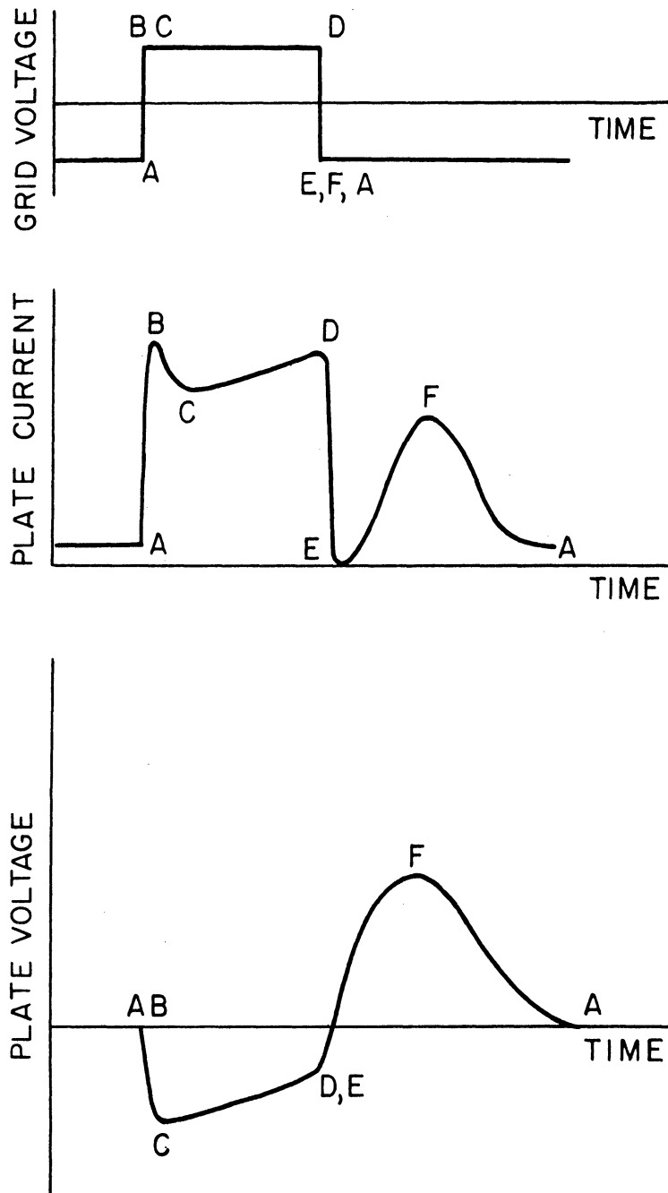
Fig. 1.4. Triode waveforms.
