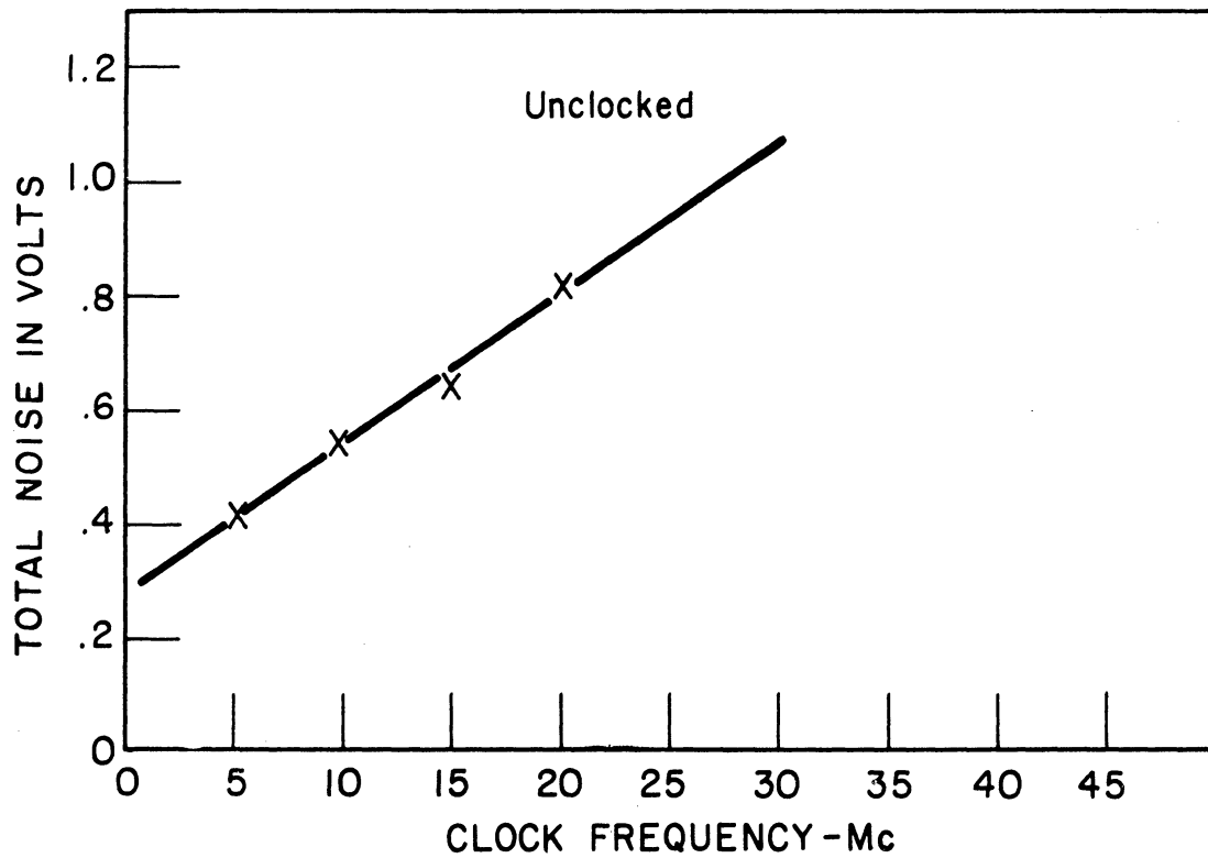
Fig. 2.29. Upper limit of performance.
