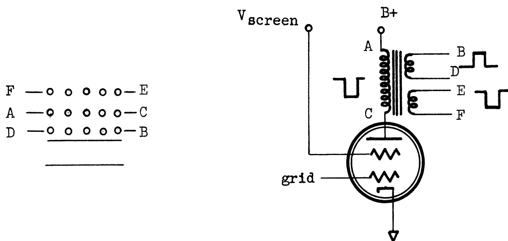
Fig. 3.10. Final winding form.
