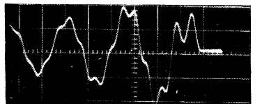
Fig. 3.9. Pulse response when the magnitude of the stray parameters is increased.
