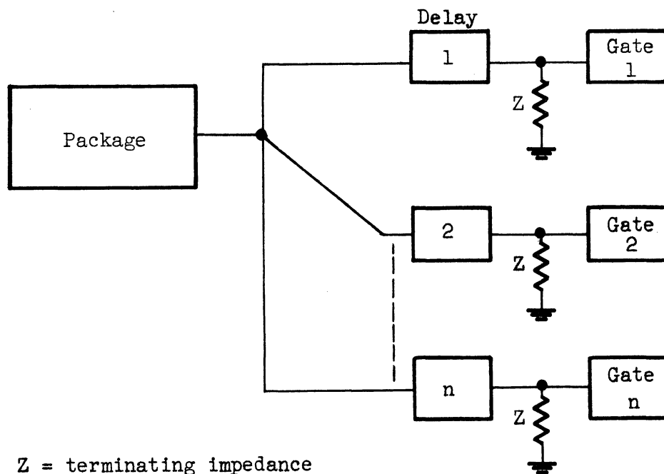
Fig. 4.1. Interconnection through n terminated cables.
