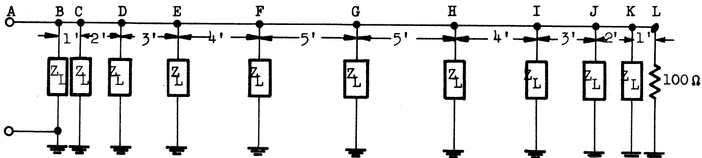
Fig. 4.3. Experimental model for reflection study.
