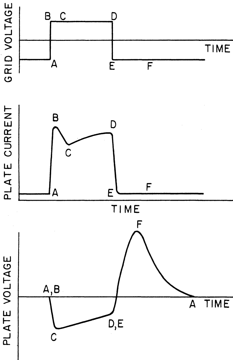
Fig. 1.2. Pentode waveforms.
