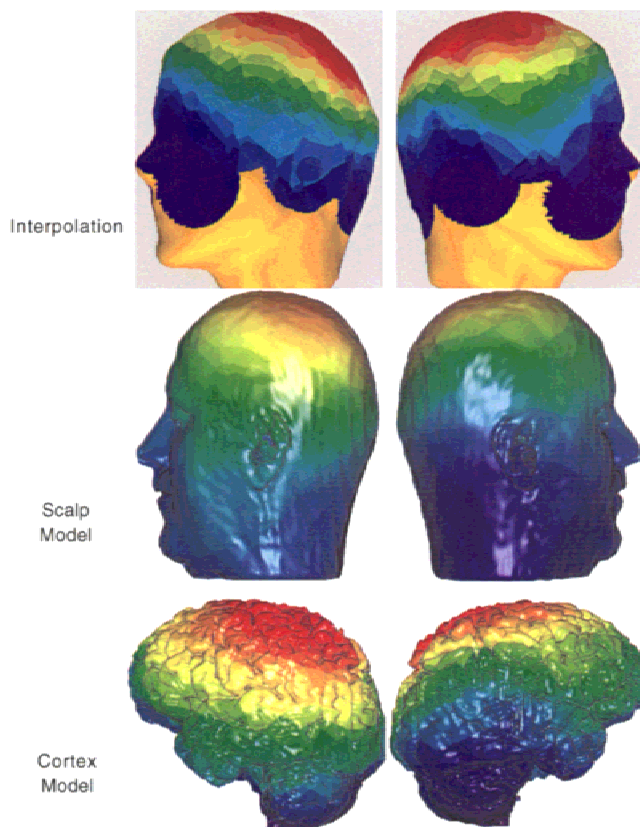
Figure 3. Spline interpolated P300 topography registered with a three-dimensional head using the SCIRun finite element modeling system. The top figures show the interpolated P300 distribution on the simulated head, the middle figures show the bioelectric model at the scalp using the subject's own MRI data, and the bottom figure shows the cortical surface model. The field distribution at the cortex more clearly shows the lateralized distribution of the P300 when the smearing effect of the higher resistance skull is removed (bottom). Dorsal positivity appears larger on the left, and ventral negativity appears larger on the right, suggestive of a transverse orientation of at least one of the P300 generators. Over both cortical hemispheres the contour of the field, as shown by color transitions, is parallel to the plane of the posterior superior temporal gyrus, with a sharp voltage gradient near that structure.
