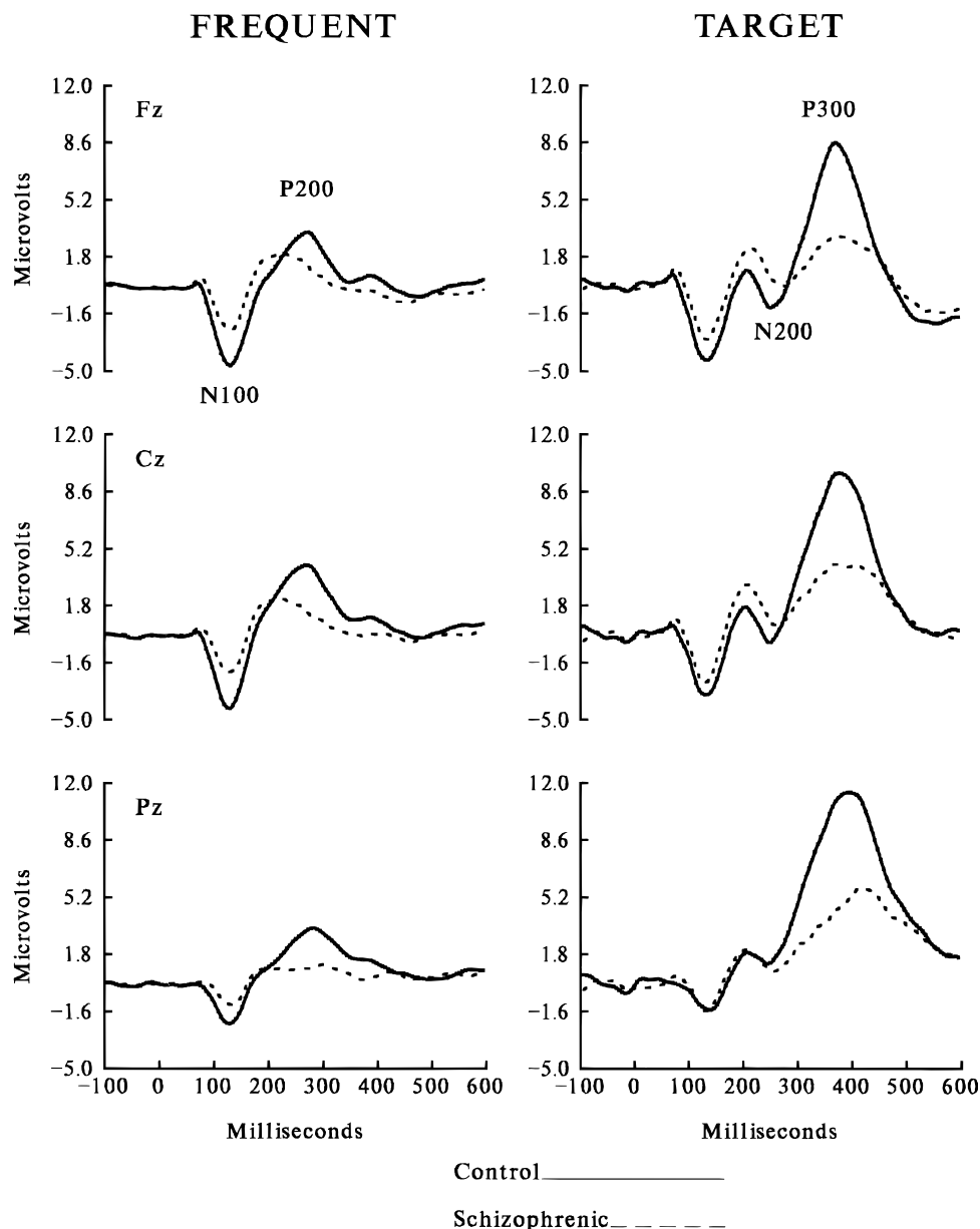
Figure 1. Grand average ERPs from normal subjects and age-, gender-, and handedness-matched patients with schizophrenia, showing marked P300 amplitude reduction to target tones at midline sites.
