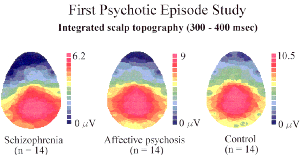
Figure 2. The voltage topography of the P300 component to target tones in normal subjects, first-episode patients with affective disorders and psychotic features, and first-episode patients with schizophrenia. Only patients with schizophrenia show a right-shifted P300 topography. Note the use of different microvolt scales for the different groups.
