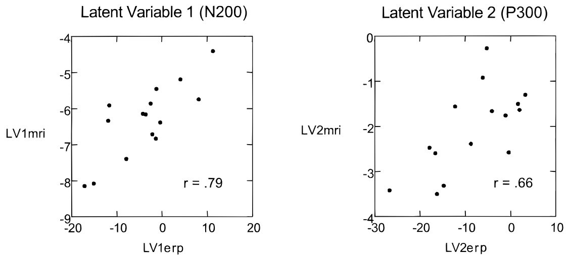
Figure 5. Scattergrams showing the relationship of ERP and MRI measures used in the partial least squares analysis for the latent variables, LV1 and LV2. For each latent variable, a subject had a score computed from the sum of the products of saliences and raw values on the ERP or MRI variable set. Plots of these scores show the nature and strength of the relationship for the N200 component (left scattergram) and the P300 component (right scattergram).
