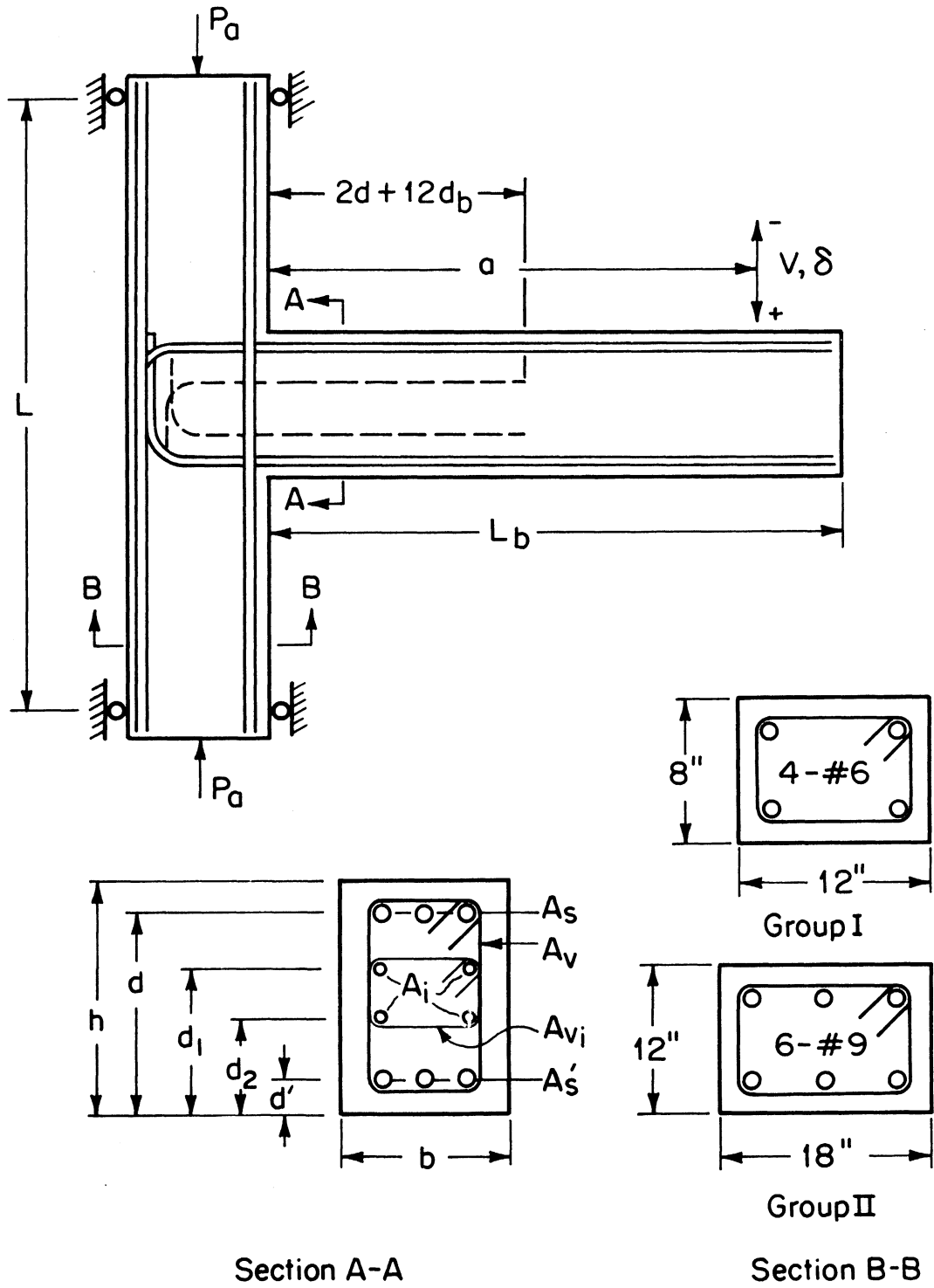
Fig. 2.1. Specimen Configuration and Dimension Designation.
