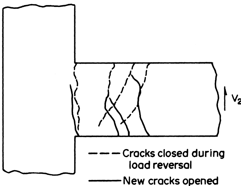
Fig. 3.7(b). Formation of Cracks during Negative Loading Half-Cycle - Specimen 1.
