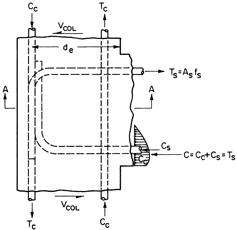
Fig. 4.7. Idealization of Forces at Beam-Column Joint.
