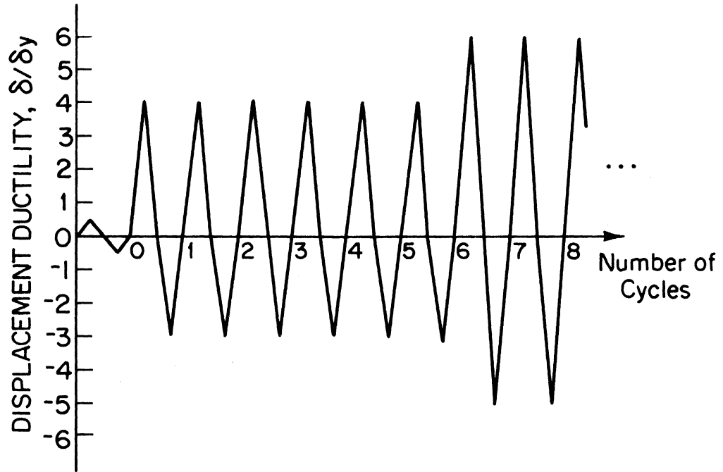
Fig. 2.4. Typical Loading Schedule.
