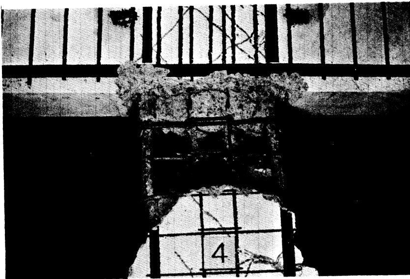
Fig. 3.17. Hinging Region of Specimen 4 after Removal of Loose Concrete.
