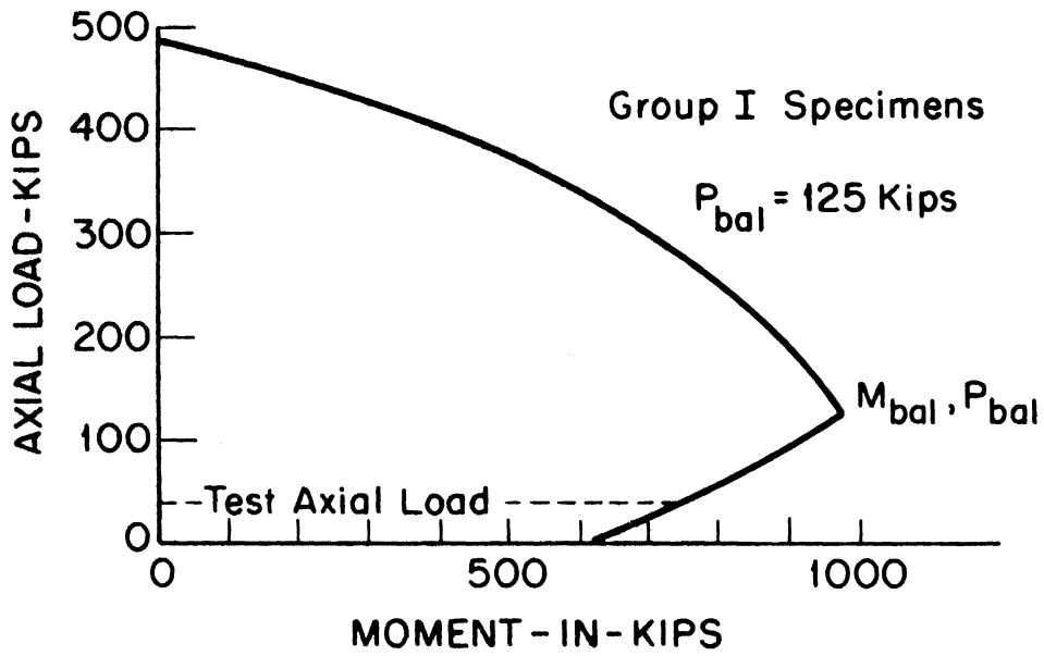
Fig. C.1(a). Interaction Diagram for Group I Specimens.
