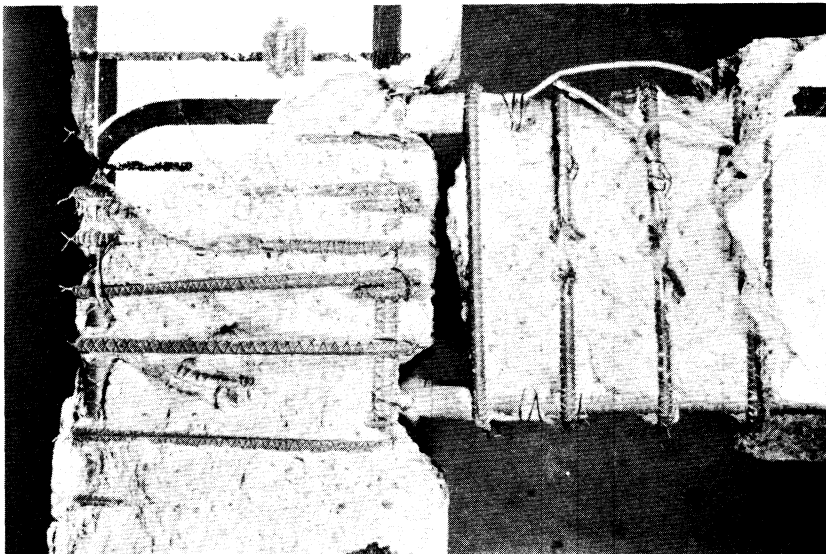
Fig. 3.25. Specimen 7 after Removal of Loose Concrete.
