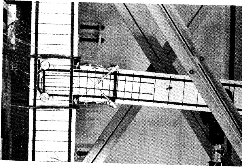
Fig. 3.38. Specimen 10 at Maximum Positive Displacement in First Inelastic Load Cycle.
