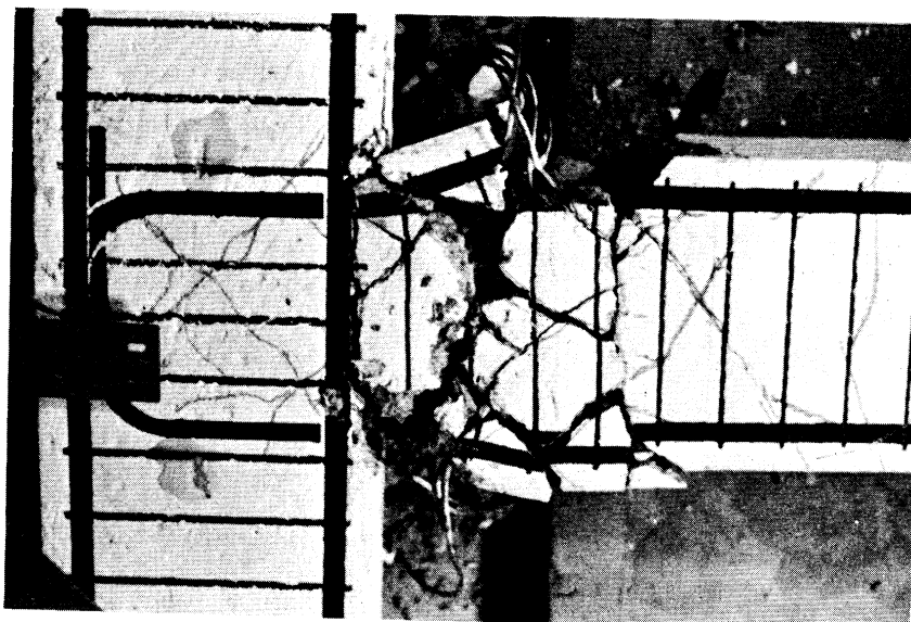
Fig. 3.20. Specimen 5 at the Conclusion of Testing.
