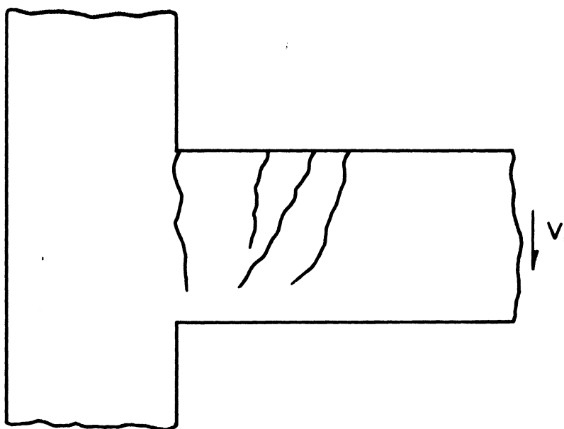
Fig. 3.7(a). Formation of Cracks during Positive Loading Half-Cycle - Specimen 1.
