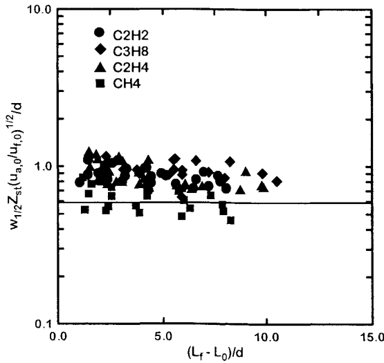
Fig. 4. Measured and predicted flame-sheet diameters as a function of air/fuel velocity ratios as a function of flame sheet length.
