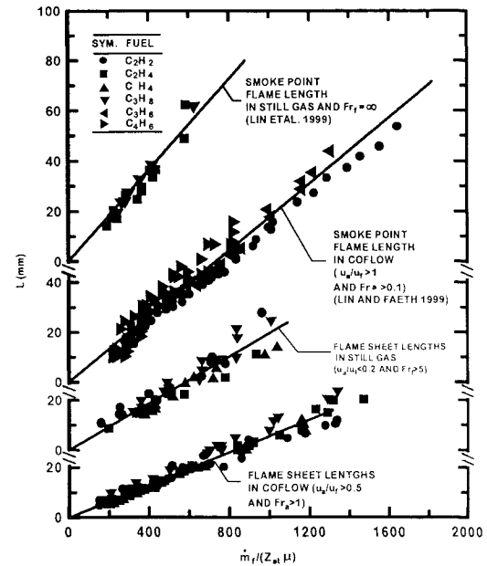
Fig. 3. Flame-sheet and luminous-flame lengths (the latter at the laminar-smoke point) of laminar jet diffusion flames in still air and coflowing air. Measurements from Lin et al. 5 , Lin and Faeth 9 and the present investigation.
