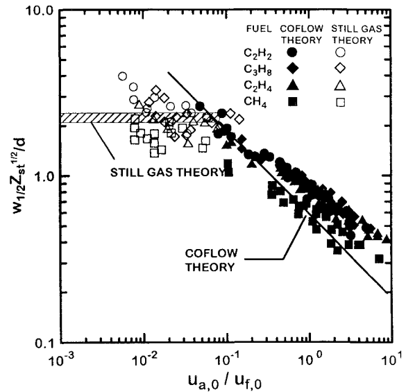
Fig. 6. Measured and predicted flame-sheet diameters as a function of air/fuel velocity ratios (small air/fuel velocity ratio limit).
