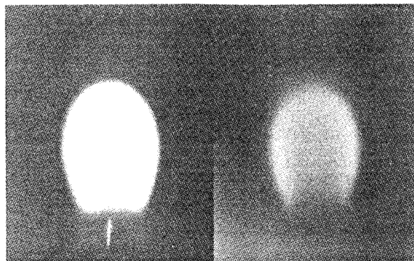
Fig. 1. Photographs of a soot-free acetylene-fueled laminar jet diffusion flame burning in coflowing air at the lift-off condition, without (left) and with (right) the C-H filter. Test conditions: d = 1.6 mm, p = 4.1 kPa and u_w/u_o = 0.05 .
