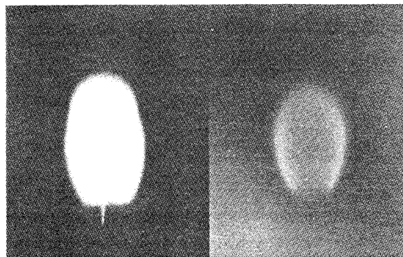
Fig. 2. Photographs of a soot-containing acetylene-fueled laminar jet diffusion flame burning in coflowing air at conditions between laminar soot- and smoke-points, without (left) and with (right) the C-H filter. Test conditions: d = 1.6 mm, p = 8.2 kPa and u_w/u_o = 0.06 .
