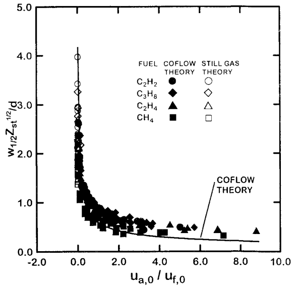
Fig. 5. Measured and predicted flame-sheet diameters as a function of air/fuel velocity ratios (large air/fuel velocity ratio limit).
