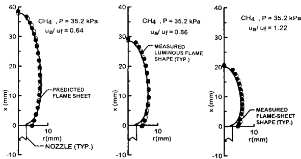
Fig. 7. Measured flame-sheet and luminous-flame shapes and predicted flame-sheet shapes for soot-free methane-fueled laminar jet diffusion flames having a burner diameter of 4.8 mm at various air coflow velocity ratios.
