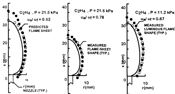
Fig. 8. Measured flame-sheet and luminous-flame shapes for soot-containing ethylene-fueled laminar jet diffusion flames having a burner diameter of 4.8 mm at various small air coflow velocity ratios.
