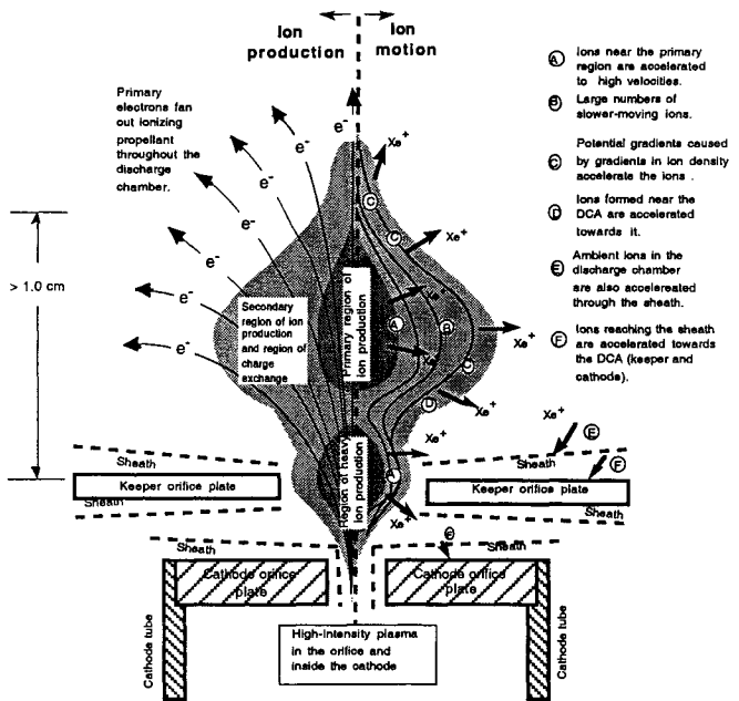
Fig. 8 Schematic of proposed Xe II acceleration mechanisms for kept operation (from Ref. 2).
