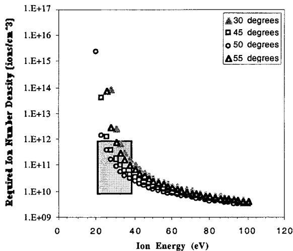
Fig. 9 Xe II number densities required for discharge cathode keeper erosion observed in 8200-hr wear test (Ref. 2).
