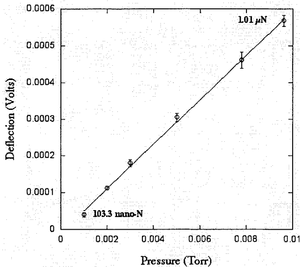
Fig. 11 Thrust stand deflection as a function of orifice stagnation pressure. The minimum thrust measured was 103 nN±20%.
