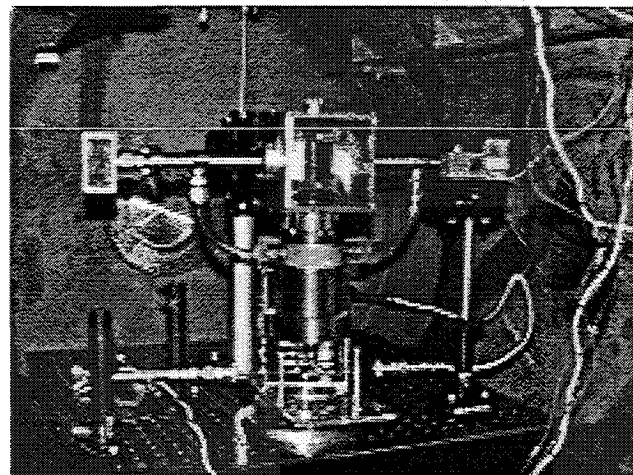
Fig. 10 USC nano-Newton torsional thrust stand.
