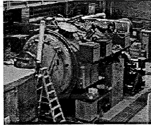
Fig. 4 TTU vacuum facility.
