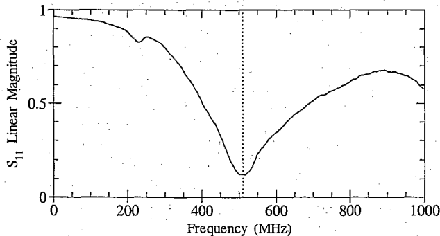
Fig. 6 Sample resonance-probe data (RP/LP-1, P5 cond. 4, 0° radial angle) showing linear magnitude of S_{11} . Minimum occurs at ~510 MHz.
