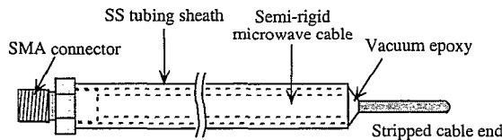
Fig. 4 Diagram of the construction of the resonance probe.
