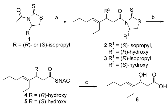
Scheme 1. Synthesis of N -acetylcysteamine (NAC) short chain TMC analogues. Reagents and conditions: a) trans -2-ethyl-2-hexenal, tin triflate, N -ethylpiperidine, CH_2Cl_2 , -78^\circ C , 70%; b) NAC, imidazole (3 equiv), CH_2Cl_2 , 85%; c) LiOH, H_2O_2 , 10% aq. THF, 90%.
