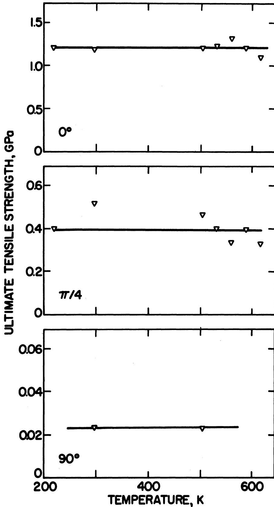
Dry Ultimate Tensile Strength of Hercules HT-S/710 Polyimide as a Function of Temperature. Data of Kerr et al. 1975 [5].
