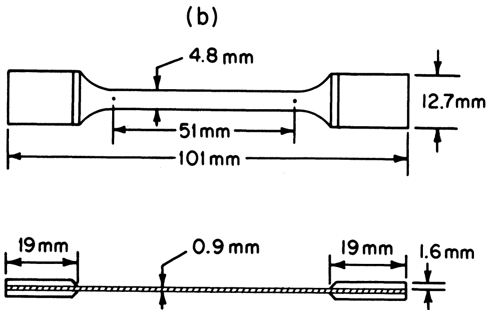
Geometry of the Test Specimen a) 0^\circ and \pi/4 Laminates, b) 90^\circ Laminates.
