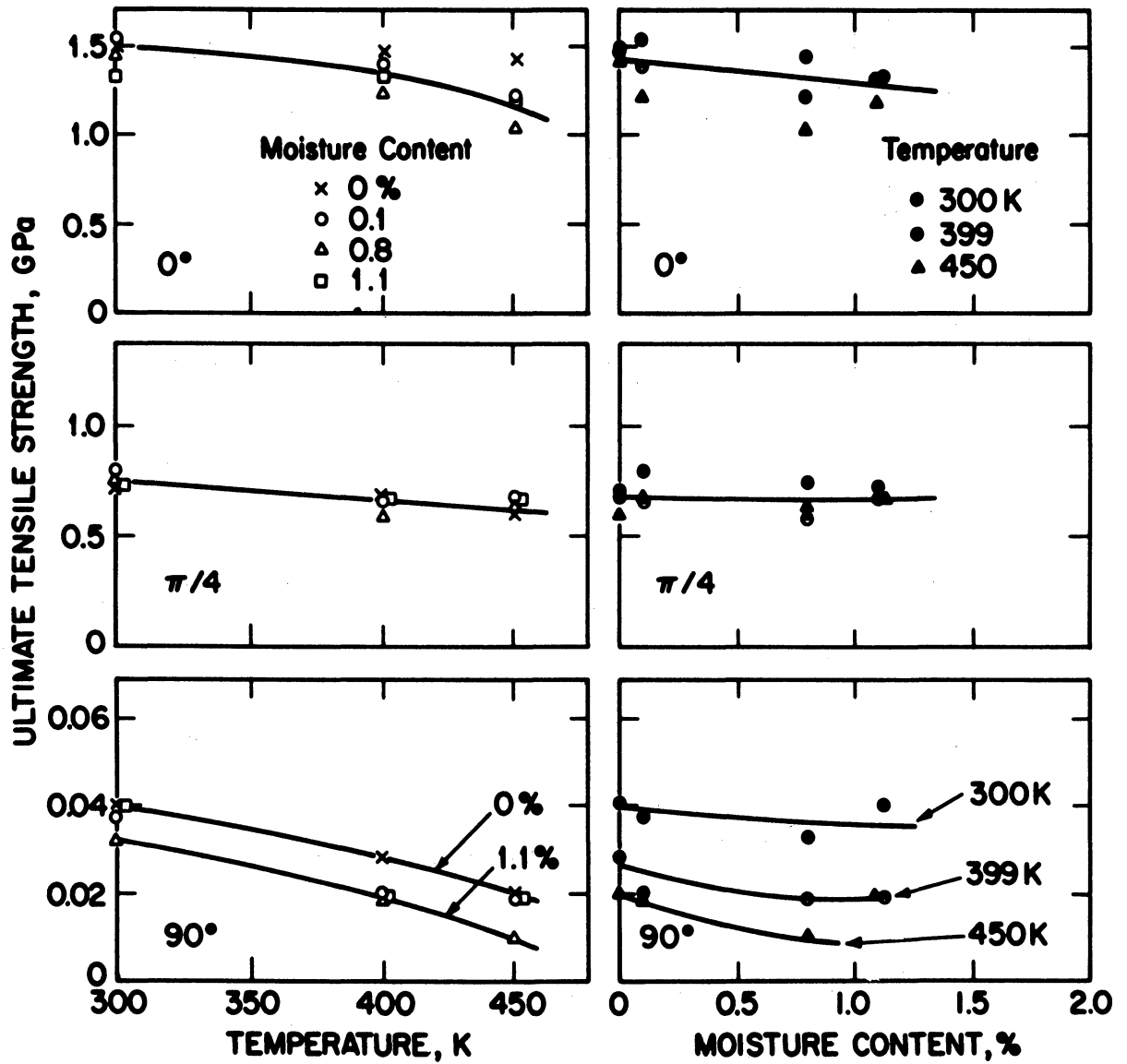
Ultimate Tensile Strength of Thornel 300/Narmco 5208 as a Function of Temperature and Moisture Content. Data of Hofer et al, 1975 [7].
