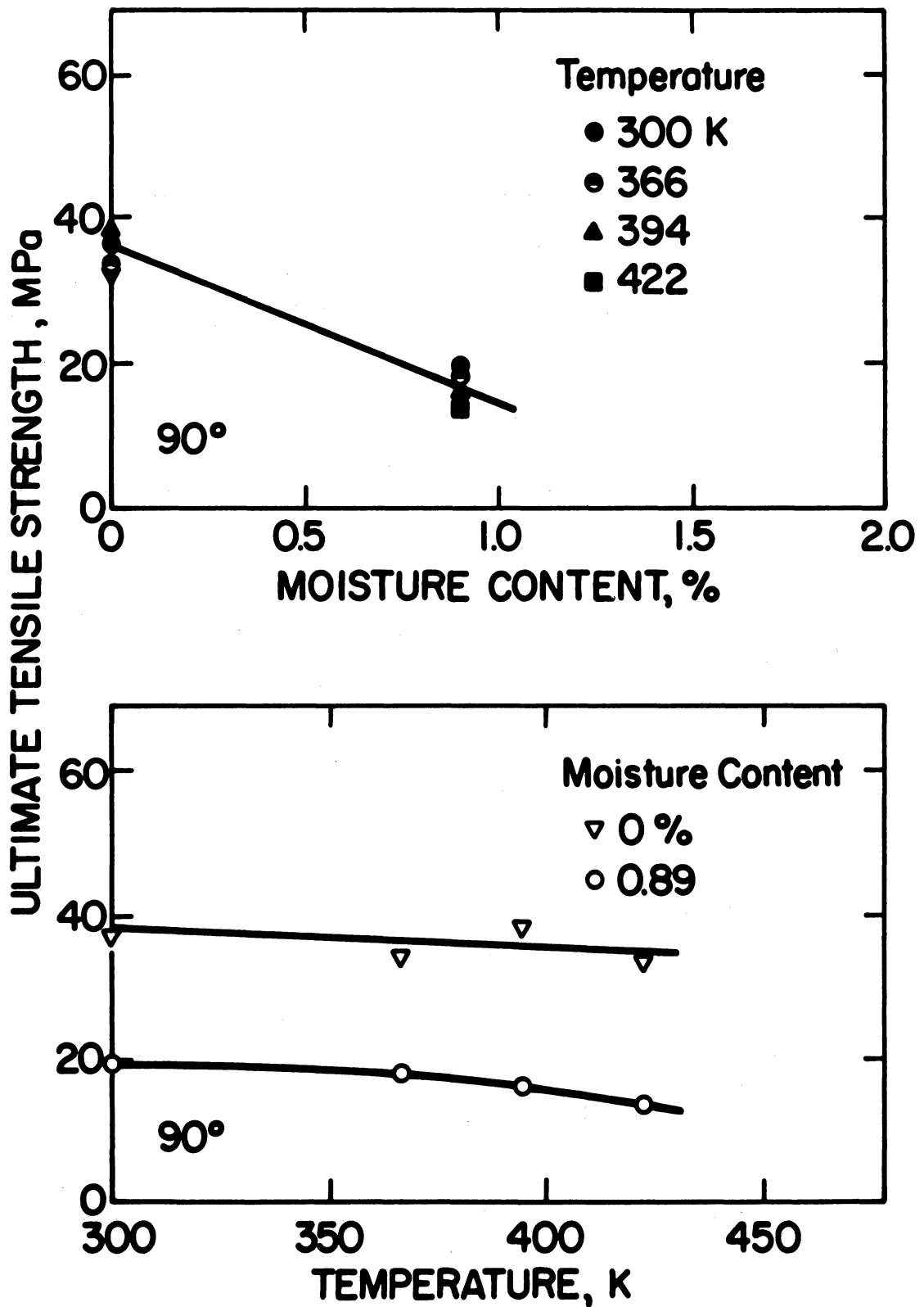
Transverse Ultimate Tensile Strength of Thorne1 300/Narmco 5208 as a Function of Temperature and Moisture. Data of Husman, 1976 [8].
