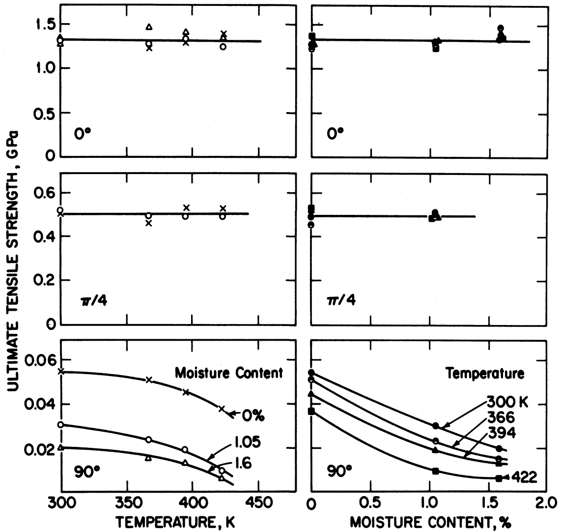
Ultimate Tensile Strength of Hercules AS-5/3501 as a Function of Temperature and Moisture Content. Data of Browning et al, 1976 [3].
