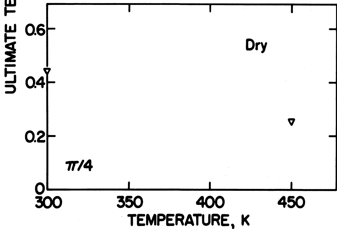
Quasi-Isotropic Ultimate Tensile Strength of HT-S/ERLA-4617 as a Function of Temperature and Moisture Content. Data of Browning, 1972 [10].
