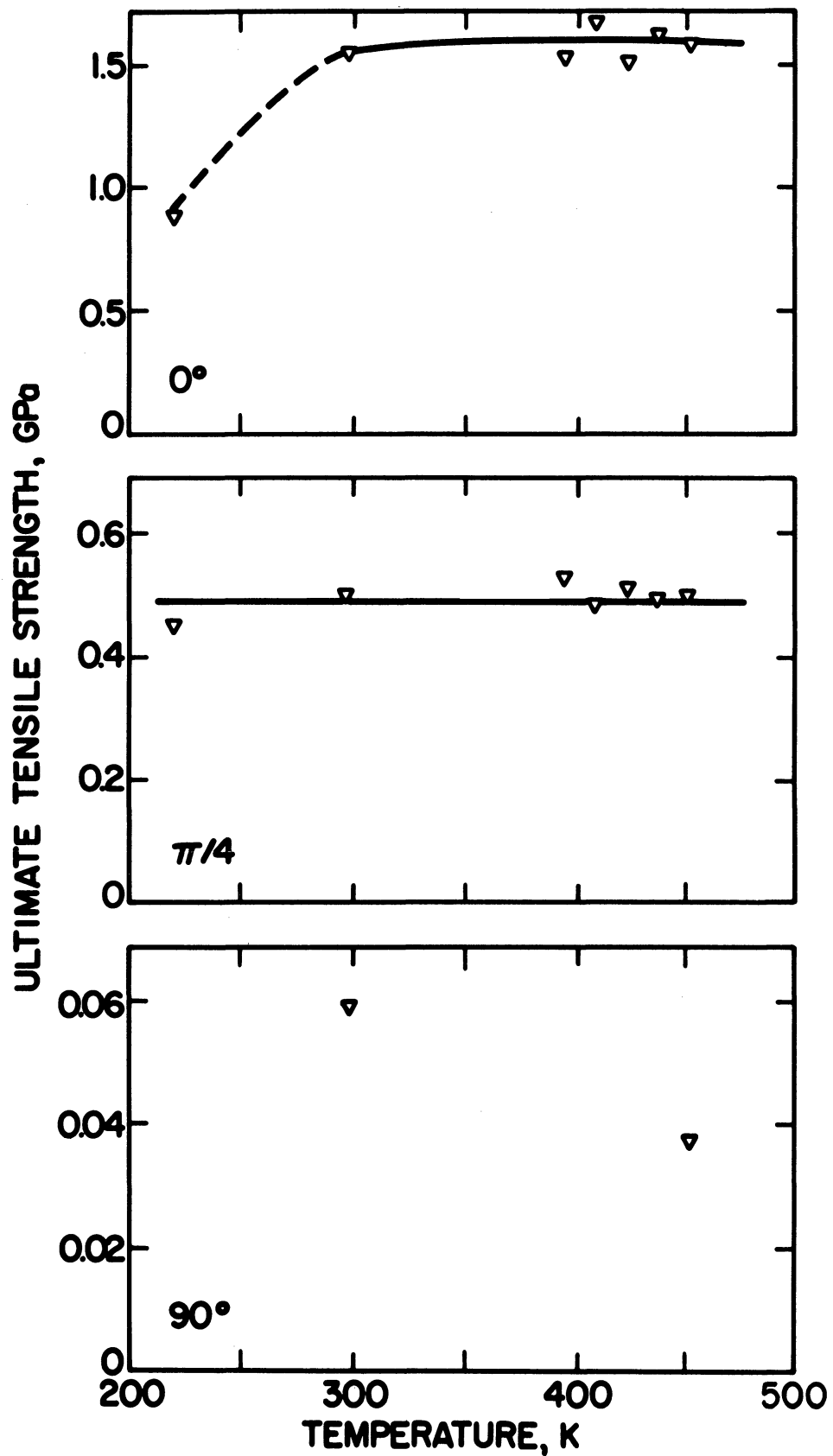
Dry Ultimate Tensile Strength of Hercules AS-5/3501 as a Function of Temperature. Data of Kerr et al. 1975 [5].
