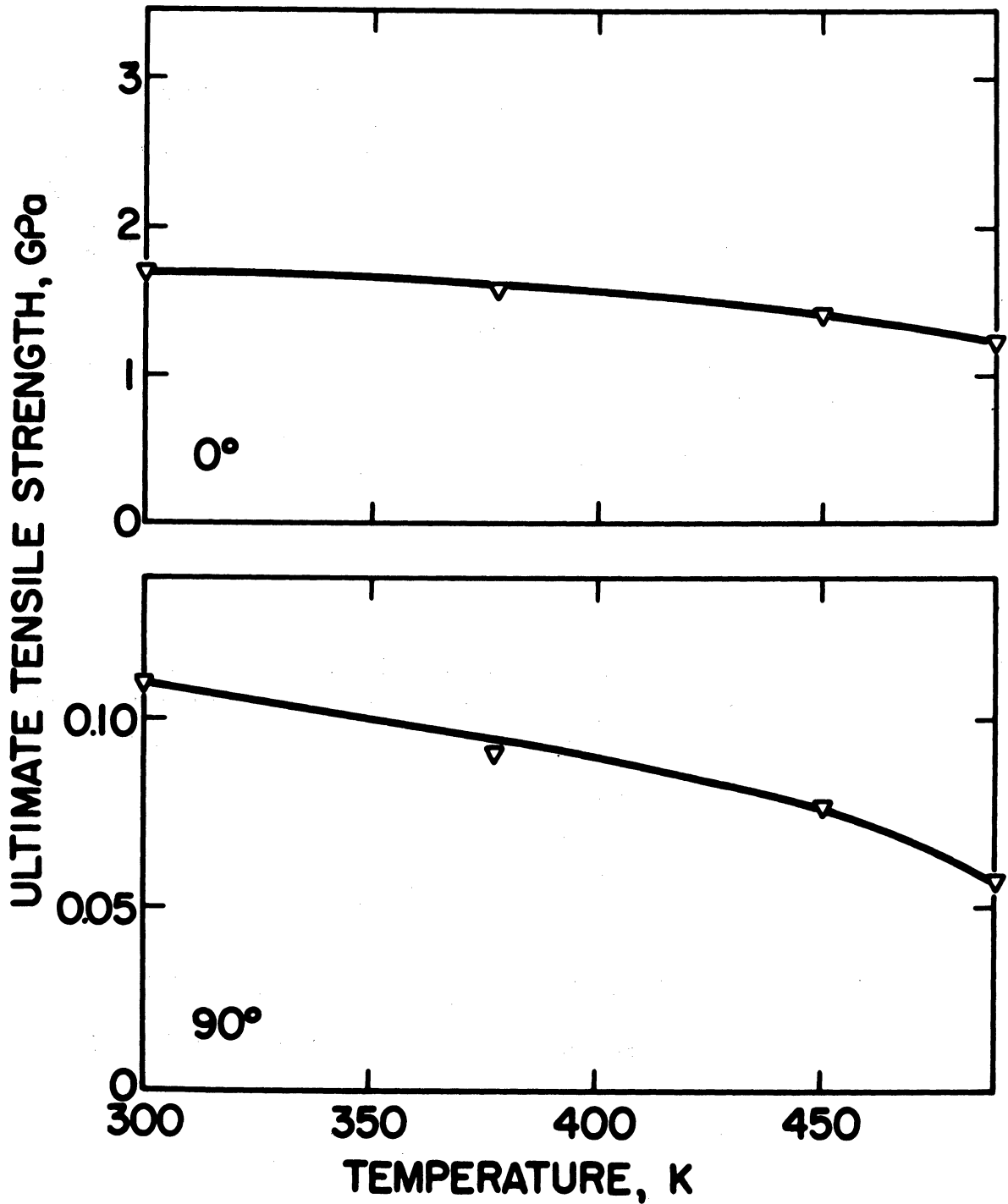
Dry Longitudinal and Transverse Ultimate Tensile Strengths of Boron/Narmco 5505 as a Function of Temperature. Data of Kaminski, 1973 [13].
