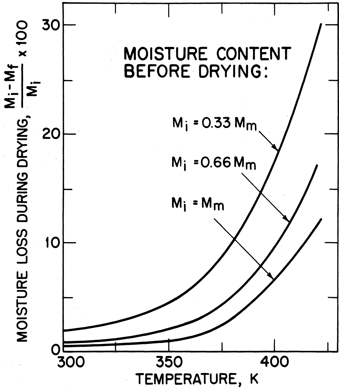
Moisture loss of specimen during three minutes of drying at different temperatures. M_i and M_f are the moisture contents before and after drying. M_m denotes moisture content at full saturation.
