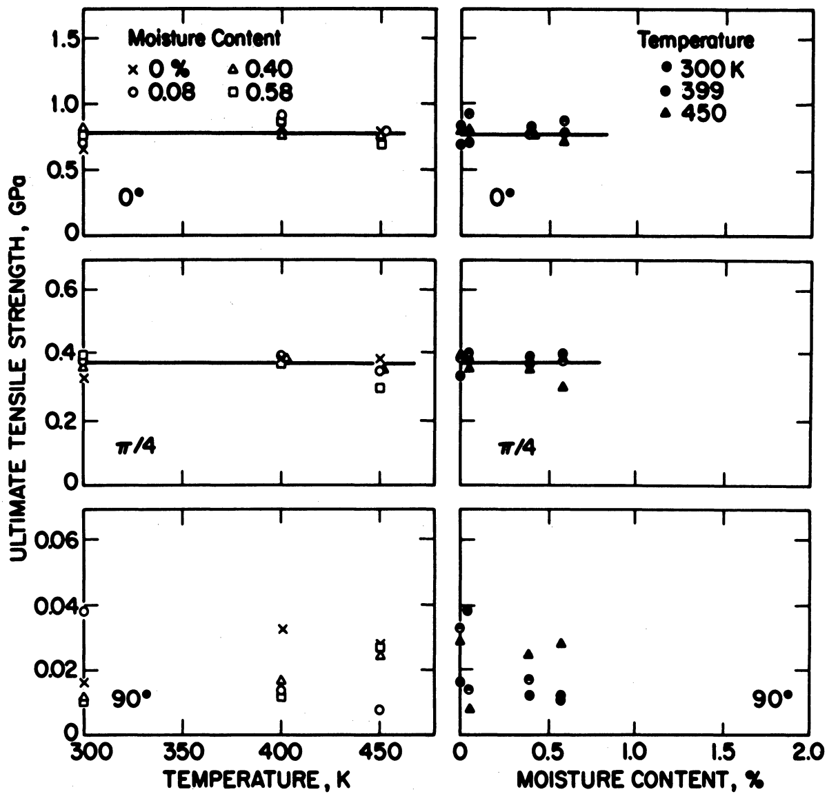
Ultimate Tensile Strength of Courtaulds HMS/Hercules 3002M as a Function of Temperature and Moisture Content. Data of Hofer et al. 1974 [9].
