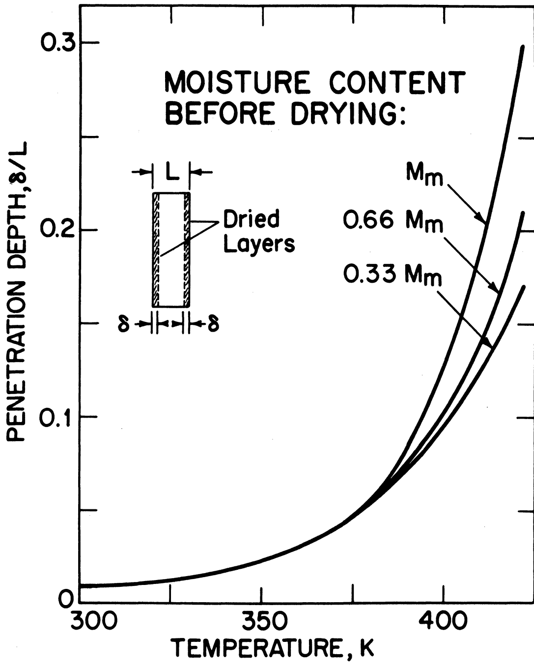
Thickness of the layer affected by three minutes of drying at different temperatures. Within "penetration depth" effect of drying is greater than 1%. M_m denotes moisture content at full saturation.
