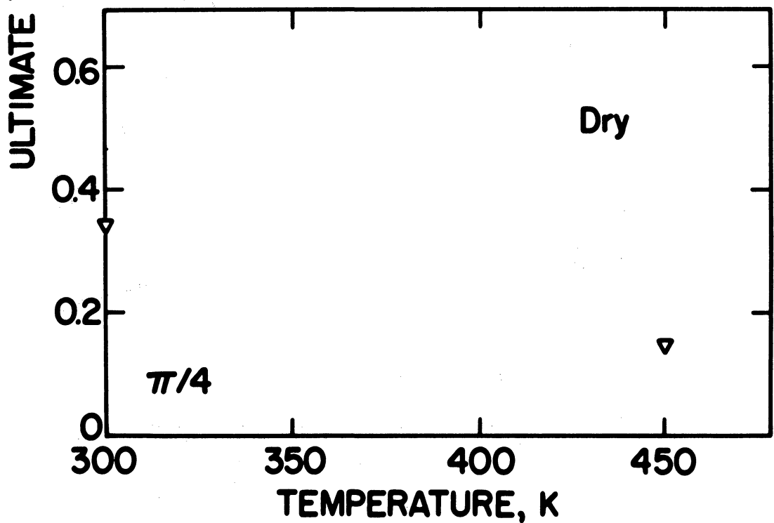
Quasi-Isotropic Ultimate Tensile Strength of HT-S/Hysol ADX-516 as a Function of Temperature and Moisture Content. Data of Browning, 1972 [10].
