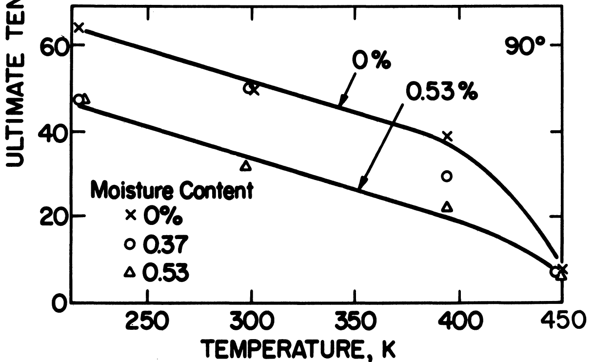
Transverse Ultimate Tensile Strength of HT-S/(8183/137-NDA-BF 3 : MEA) as a Function of Temperature and Moisture Content. Data of Hertz, 1973 [12].
