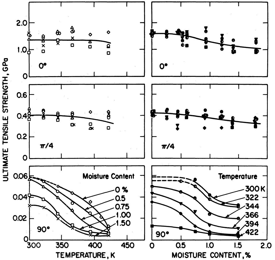
Ultimate Tensile Strength of Thornel 300/Fiberite 1034 as a Function of Temperature and Moisture Content. Present Data.
