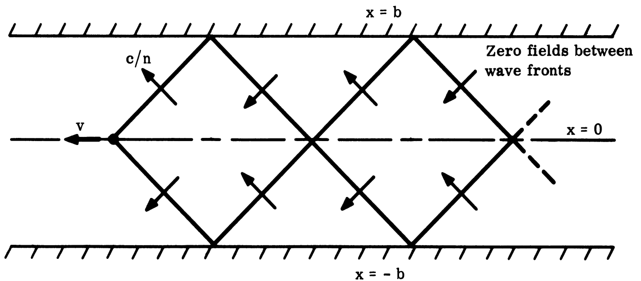
FIG. 3: SHOCK WAVE GEOMETRY, PARALLEL PLATE BOUNDARY
