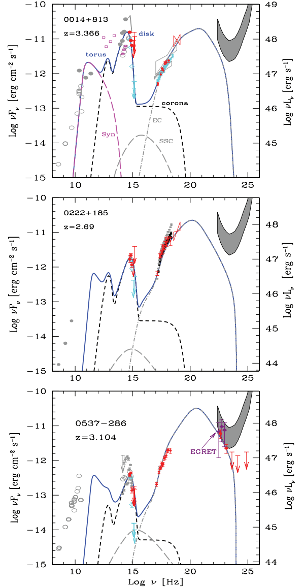
Figure 4. SEDs of S5 0014+813, 0222+185 (i.e. RBS 315) and PKS 0537–286 together with the fitting models, with parameters listed in Table 4. De-absorbed UVOT, XRT and BAT data are indicated by darker symbols (red in the electronic version), while archival data [from NASA/IPAC Extragalactic Database (NED)] are in light grey. Diamonds (and lower arrows, cyan in the electronic version) indicate UVOT data not de-absorbed by intervening Lyman \alpha clouds. The magenta square symbols for S5 0014+813 are IRAS and Two Micron All Sky Survey (2MASS) data points. The short-dashed line is the emission from the IR torus, the accretion disc and its X-ray corona. The long-dashed and the dot-dashed grey lines are the synchrotron self-Compton and the external Compton components, respectively. The thick solid (blue) line is the sum of all components.
