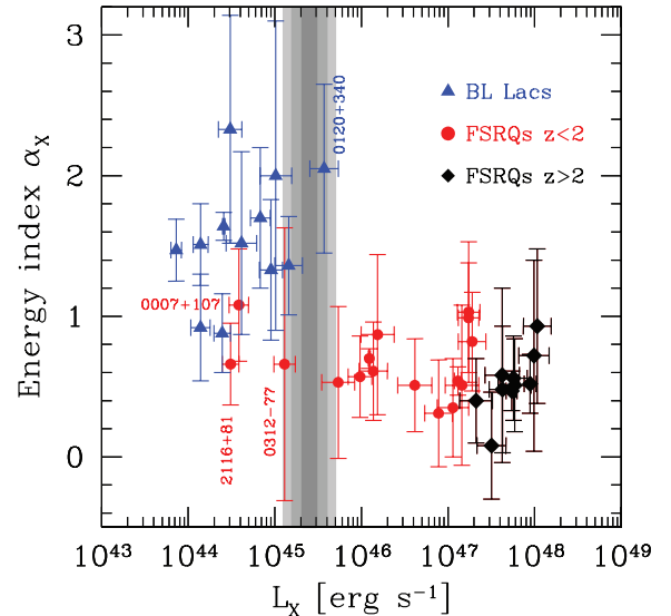
Figure 2. The X-ray energy spectral index \alpha_X as a function of the luminosity in the BAT energy range 15–55 keV. In this plane BL Lacs (triangles) and FSRQs (circles and diamonds) are clearly separated. We also mark (black diamonds) the FSRQs with z > 2 . The labelled sources are the BL Lac IES 0120+340 ( z = 0.272 ) and the three sources classified as FSRQs by A09 to the left-hand side of the divide. Note that of these three objects, B0007+107 (i.e. Mkn 1501) is a Seyfert 1 galaxy at z = 0.09 with a superluminal jet (Brunthaler et al. 2000) and S5 2116+81 ( z = 0.084 ) is a radio galaxy (Stickel, Kühr & Fried 1993). The grey stripes indicate the X-ray luminosity dividing BL Lacs from FSRQs.
