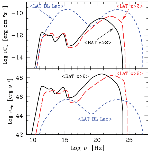
Figure 12. Average SEDs for the sources in our samples, for all FSRQs detected by Fermi and for the subsample of the eight Fermi blazars at redshift z > 1.8 . The top and the bottom panels show the fluxes and luminosities, respectively. The shown frequencies are calculated in the rest frame of the source for the luminosity plot, and are the observed ones for the flux plot. In Table 4 we list the parameters used to construct the shown SEDs for FSRQs, while, for the LAT BL Lacs, we report the same SED as shown in G10.
