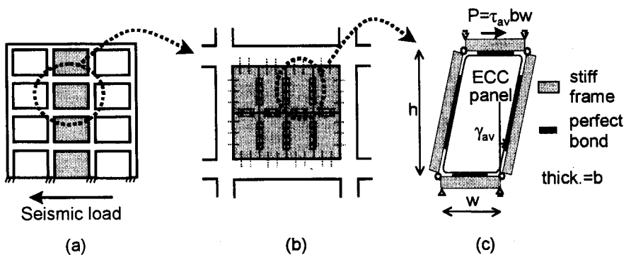
Fig. 6 Retrofit shear wall and its simplified model
