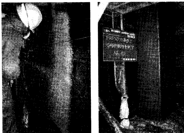
Fig. 3 Process of FRP reinforcement (left) and FRP retrofitted RC column (right).
