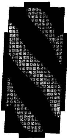
Fig. 7 Deformed shape and cracking strain distribution of ECC panel with steel plates/dowels along vertical and horizontal joints
