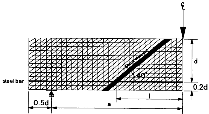
Fig. 1 Finite element mesh for analysis of shear crack growth
