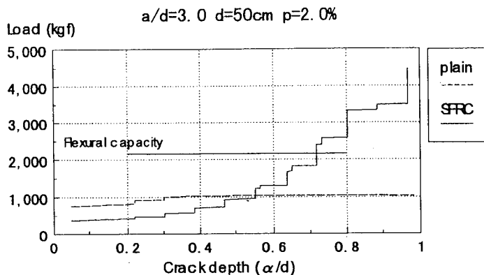
Fig. 2 Load vs. crack depth for RSFC and RC beams
