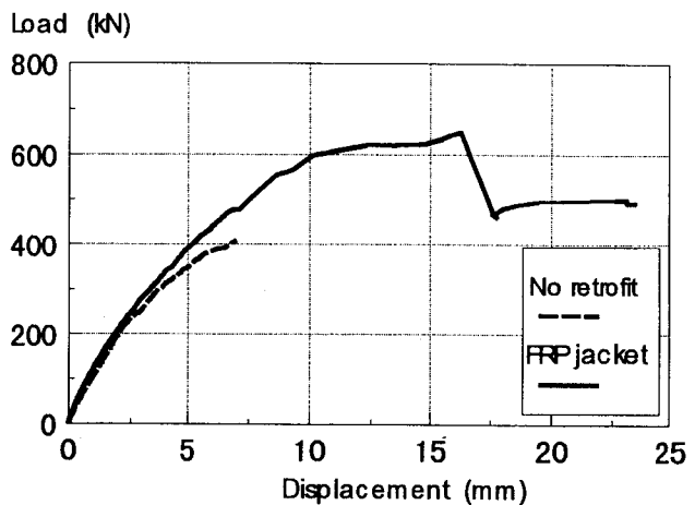
Fig. 5 Load vs. displacement measured in tests
