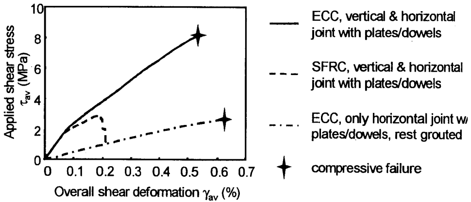
Fig. 9 Computed overall shear stress-overall shear deformation curves for retrofit panels
