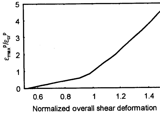
Fig. 10 Relationship between the maximum compressive plastic strain and the overall shear deformation
