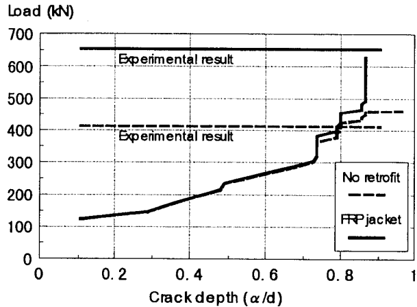
Fig. 4 Load vs. crack depth for RC columns with and without FRP jacketing
