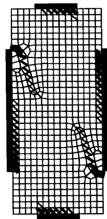
Fig. 8 Discrete cracking pattern in quasi-brittle SFRC panel
