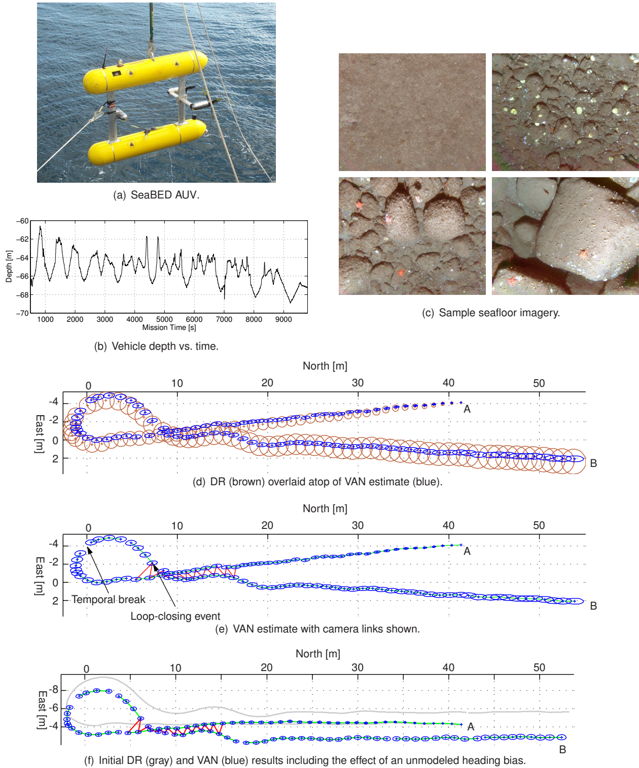
Fig. 16. A depiction of the Stellwagen Bank data set and a comparison between the resulting VAN and DR trajectory estimates; the survey started at A and ended at B. (a) The SeaBED AUV used for the experiment. (b) A plot of vehicle depth vs. time for this mission. Since the vehicle was trying to maintain constant-altitude, the depth plot serves as a proxy for terrain variation. Note that depth excursion are on the order of several meters. (c) A sampling of imagery collected during the survey. The seafloor topography ranges from pure sand (upper left) to large boulders (lower right). (d) Shown in blue is the XY plot of 100 estimated camera poses with 3\sigma confidence ellipses. For comparison, overlaid in brown is the DR estimated trajectory. Notice that the DR error monotonically increases while the VAN error is bounded for images in the vicinity of the cross-over point. (e) The same 100 estimated camera poses, but with image constraints superimposed. The green links indicate that a camera-derived measurement was made between temporally consecutive image pairs, while the red links indicate that a cross-track measurement was made. In all, there are 19 cross-track measurements. (f) The initial DR and VAN results, each of which includes an unmodeled heading bias. Notice that the DR trajectory (gray) does not lie within the 3\sigma VAN estimate (blue). This discrepancy comes from an unmodeled compass bias, which when accounted for, produces the results shown in (d).
