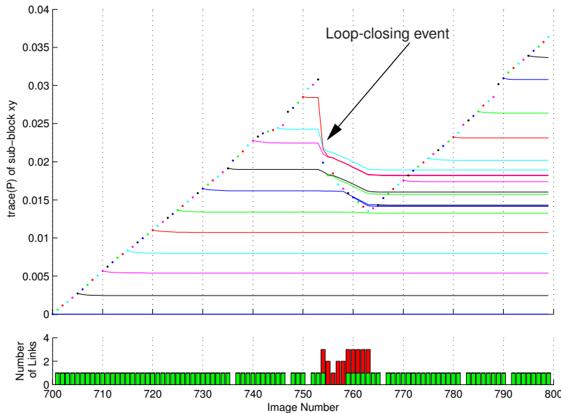
Fig. 17. A depiction of the time-evolution of the Stellwagen Bank pose-network uncertainty. (top) For each delayed-state entry in \xi_t (i.e., for each vehicle pose \mathbf{x}_{p_i} ), the trace of its 2 \times 2 XY covariance sub-block is plotted versus image frame number. The dots depict the pose uncertainty at image insertion and the lines show their time evolution for every 5 th delayed-state. A couple of key events are worth pointing out. First, notice the monotonically increasing uncertainty in XY position between frames 700–753. This initial period corresponds to only sequential pairwise camera measurements. Second, notice the regional smoothing and sharp decrease in uncertainty at frame number 754; this is the first cross-track camera measurement. The pose uncertainty continues to decrease as more cross-track measurements are made (frames 755–763). Finally, from frame 764 onward, uncertainty begins to increase again as no more spatial measurements can be made. (bottom) A bar graph of the number of successfully registered image pairs for each frame number. Sequential camera measurements are green and cross-track measurements are red. Notice that the decrease in XY uncertainty in the covariance plot coincides with the first cross-track measurement.
