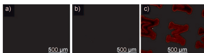
Figure 2. Chemical reactivity comparison of polymers 1 and 2 under copper-free condition using \mu\text{CP} for 3 h at room temperature. CVD polymer coatings on samples: a) poly( p -xylylene) (no reactive functional group, R = H in Scheme 1); b) polymer 1 (with nonactivated alkyne groups); c) polymer 2 (with activated alkyne groups). After CVD coating, the same treatment was applied to samples all 3 samples: \mu\text{CP} of biotin-PEG-azide followed by TRITC-streptavidin solution incubation. Scale bars represent 500 \mu\text{m} .
