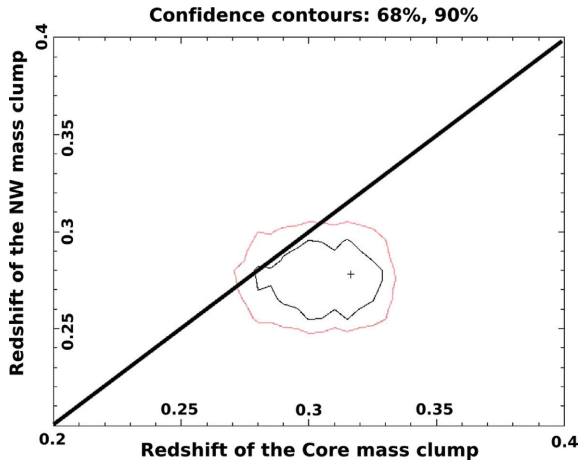
Figure 6. Simultaneous fits to the redshifts of the Core region and the NW substructure using two ACIS-I and one ACIS-S pointings. The two contours correspond to 68 per cent (inner) and 90 per cent (outer) confidence levels, and the diagonal line indicates equal redshifts to guide the eye. The Core mass clump appears significantly redshifted when compared to the NW mass clump.
