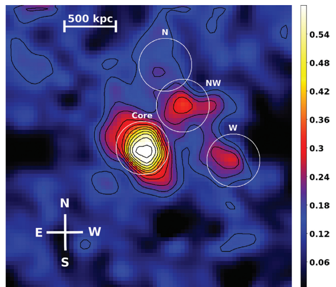
Figure 3. The convergence map of the cluster field for a source redshift of z_s = \infty and a field size of 600 \times 600 \text{ arcsec}^2 , translating to \sim 2.7 \text{ Mpc} on a side. The black contours start at \kappa_0 = 0.14 with a linear spacing of \Delta\kappa = 0.047 . The four white circles with labels indicate identified sub-clumps and the radius within which their mass is calculated. The radius of all four circles is 55.4 \text{ arcsec} \approx 250 \text{ kpc} .
