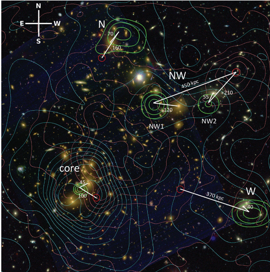
Figure 1. The field of Abell 2744, with different interesting features. The false-colour background is provided by HST/ACS (the two pointings can be identified by the higher, blue background noise level), VLT and Subaru images on a field size of 240 \times 240 arcsec 2 ( \sim 1.1 Mpc on a side). Overlaid in cyan are the surface mass density contours most concentrated in the ‘core’ area and in magenta the more evenly distributed X-ray luminosity contours. The peak positions of the core, N, NW and W clumps are indicated by the green likelihood contours, derived from the bootstrap samples. Contours are 86 per cent, 61 per cent and 37 per cent of the peak likelihood for each clump. (Assuming a Gaussian probability distribution, these would correspond to 0.3\sigma , 1\sigma and 2\sigma confidence contours.) Note that the NW clump most likely peaks in the area indicated by NW1 (in 95 per cent of the bootstrap realizations), but peaks also at NW2 in 54 per cent of the bootstrap realizations. The small red circles show the position of the local overdensities in the gas distribution, associated with each individual dark matter clump. The white rulers show the separation between dark matter peaks and the bright clusters galaxies and local gas peaks.
