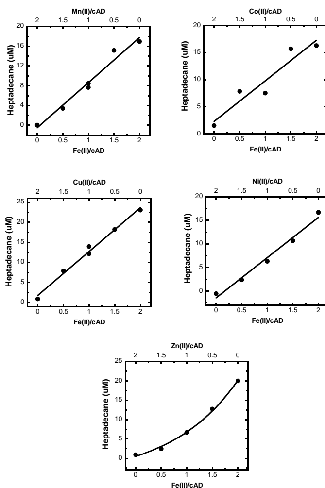
Figure S4. Dependence of heptadecane formation upon reconstitution of apo-cAD with Fe (II) and other most relevant biologically active metals at a total metal equivalency of 2 per cAD active site. Assay conditions: 20 µM apo cAD, 300 µM octadecanal, 100 µM PMS and 1 mM NADH were reacted at 37 °C for 1 hour as described above in assay procedures and heptadecane was quantified by GC.
