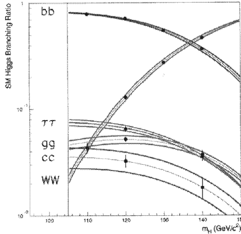
FIGURE 2. Predicted SM Higgs branching ratios, together with the measured values obtainable with 500 \text{ fb}^{-1} at \sqrt{s} = 350 \text{ GeV} , from the study in Ref. [13].
