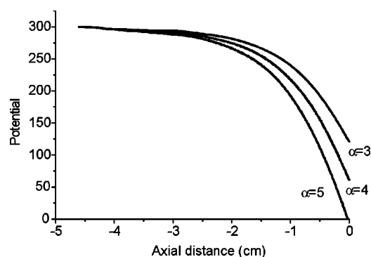
FIG. 10. Simulation results: Potential distribution inside the Hall thruster channel. Bohm anomalous conductivity effect. \alpha is the empirical coefficient in Eq. (7).
