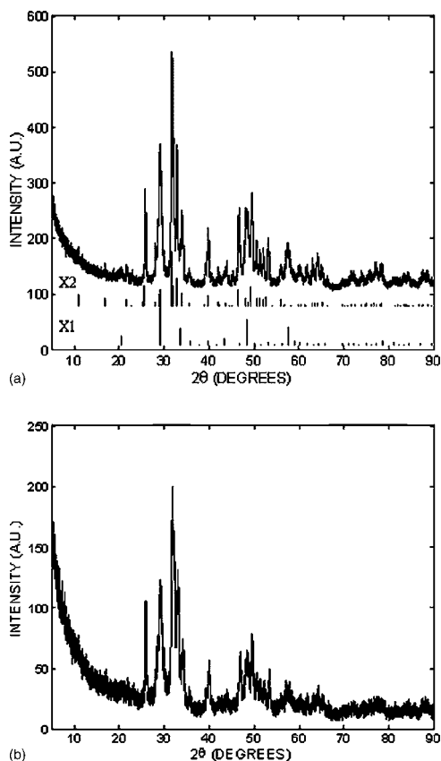
FIG. 1. X-ray diffraction pattern of \text{Y}_2\text{O}_3:\text{Eu}^{3+} coated HA particles. Samples are annealed at (a) 850^\circ\text{C} and (b) 650^\circ\text{C} . Principal diffraction peaks of the \text{Y}_2\text{O}_3 (X1) and \text{Ca}_{10}(\text{PO}_4)_6(\text{OH})_2 (X2) are shown (Refs. 24 and 25).
