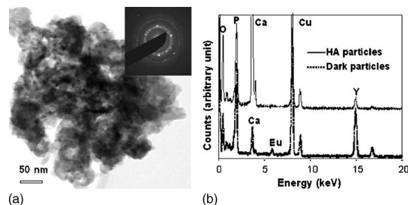
FIG. 2. Bright-field TEM image showing the typical morphology of \text{Y}_2\text{O}_3:\text{Eu}^{3+} coated HA particles heated at 850^\circ\text{C} , and the inset is the selected area electron diffraction pattern from the HA substrate. (b) EDS spectra acquired from the HA nanoparticle substrate and \text{Eu}-\text{Y}_2\text{O}_3 nanoparticles.
