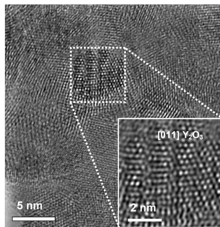
FIG. 3. High resolution TEM image showing the crystalline feature of HA nanoparticles heated at 850^\circ\text{C} . The lattice image (inset in Fig. 3) of a nanoparticle showing dark contrast can be indexed by the structural data of the cubic \text{Y}_2\text{O}_3 phase.
