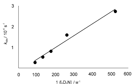
Figure 3. Plot of k_{\text{obs}} versus 1/[\text{C}_5\text{D}_5\text{N}] for reductive elimination from 3\text{-BF}_4 to form 6\text{-BF}_4 in \text{CD}_2\text{Cl}_2 at 45^\circ\text{C} . \gamma = (5.65 \times 10^{-7})x - 1.39 \times 10^{-5} ; R^2 = 0.979 .
