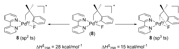
Scheme 5. Calculated energies for \text{C}(\text{sp}^3)\text{-F} versus \text{C}(\text{sp}^2)\text{-F} bond-forming reductive elimination from 8 (ts = transition state).
