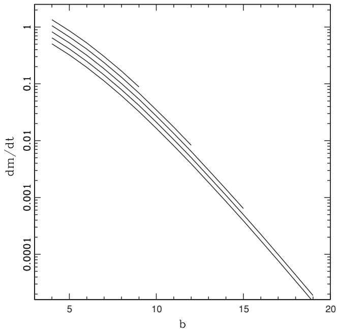
Figure 5. Dimensionless mass outflow rate vs. dimensionless depth b of the gravitational potential well of the planet. The curves show the results for different values of the magnetic field strength parameter \beta , from \beta = 0.0005 (bottom curve) to \beta = 0.008 (top curve).
