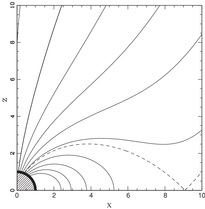
Figure 1. Magnetic field lines centered on the planet for field configurations with background parameter \beta \approx 0.0014 . The solid curves show a set of field lines for starting values of \sin\theta that are evenly spaced. The dashed curve shows the field line that passes through the X-point. The field lines near the poles are open and join onto the background field lines provided by the star and stellar wind. The field lines near the equator are closed and end back on the planetary surface. In this coordinate system, distances are measured in units of the planet radius, and the star is located at position (x, y, z) = (100, 0, 0) .
