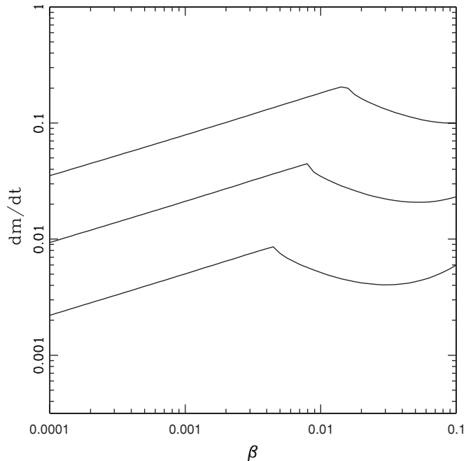
Figure 6. Dimensionless mass outflow rate vs. magnetic field strength parameter \beta . The curves show results for different values of the dimensionless depth b of the gravitational potential well of the planet, where b = 12 (bottom), b = 10 (middle), and b = 8 (top). Local maxima occur for the largest values of \beta that allow the flow along all of the open streamlines to pass smoothly through the sonic point (see the text).
