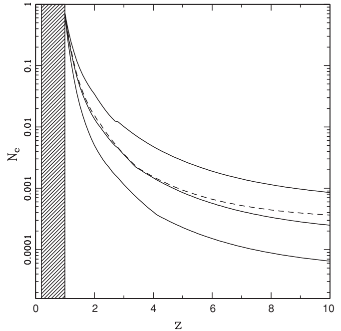
Figure 8. Dimensionless column density through the outflow as a function of vertical coordinate z (in units of the planet radius R_P ). Solid curves show the column density for magnetic field parameter \beta = 0.001 with three values of the dimensionless depth b of the planetary gravitational potential well: b = 8 (top), 10 (middle), and 12 (bottom). The dashed curve shows the b = 10 case with larger field strength parameter \beta = 0.002 . Optical depth is obtained from the dimensionless column density through the relation \tau = \mathcal{F} n_1 \sigma_{\text{uv}} R_P N_c \sim 20 N_c .
