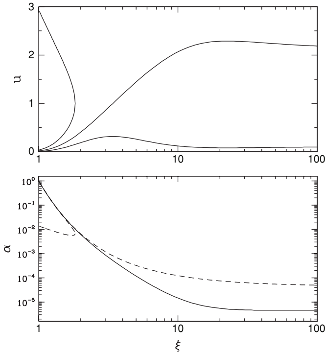
Figure 4. Top panel shows the velocity profiles for outflows from planetary surfaces for flow with q = 0 (from the planetary pole). The three curves show the velocity as a function of radius \xi for the critical value of \lambda/q (central curve), for a subcritical case (bottom curve), and a supercritical case (top curve). These velocity profiles were calculated using b = 10 and \beta = 10^{-3} . Bottom panel shows the corresponding density profiles. The critical case is shown as the solid curve, whereas the dashed curves show the subcritical case (which continues to large \xi ) and the supercritical case (which is confined to small \xi ).
