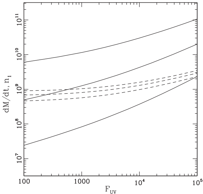
Figure 7. Mass outflow rates as a function of the UV flux from the star. The outflow rate dM/dt = \dot{M} is given in \text{g s}^{-1} , and the UV flux is given in \text{erg cm}^{-2} \text{s}^{-1} . Solid curves show the outflow rates for three values of the planet mass, from M_P = 0.5 M_J (top curve) to M_P = 1.0 M_J (bottom curve). Dashed curves show the number density n_1 (in \text{cm}^{-3} ) at the \tau = 1 surface for the same cases. The magnetic field strength parameter \beta = 0.001 for all cases shown.
