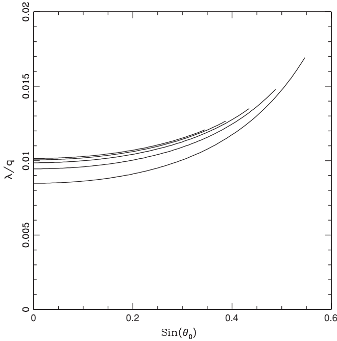
Figure 3. Values of the parameter \lambda/q that allow the outflow to pass smoothly through the sonic point. The parameters \lambda are shown here as a function of \sin \theta_0 = q(2 + \beta)^{-1/2} , which determines the starting point of the streamlines. All cases use b = 10 (where b = GM_P/(a_s^2 R_P) sets the depth of the gravitational potential of the planet). Curves are shown for a range of the parameter that sets the relative strength of the stellar and planetary magnetic fields: \beta = 0.008 (bottom curve), 0.004, 0.002, 0.001, and 0.0005 (top curve). For smaller values of \beta , the curves converge toward a well-defined locus (although the range in \sin \theta_0 shrinks).
