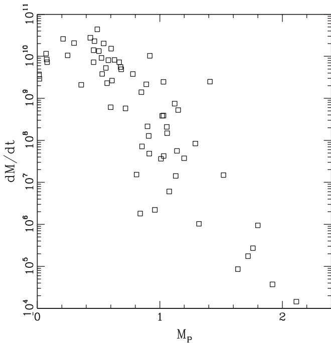
Figure 9. Rough estimates for mass outflow rates for the sample of extrasolar planets observed in transit. Mass outflow rates dM/dt = \dot{M} are given in \text{g s}^{-1} ; planetary masses are given in Jovian masses M_J .
