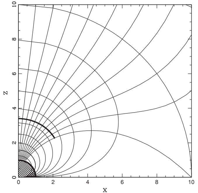
Figure 2. Sonic transition surface for the planet with dimensionless gravitational potential depth b = GM_p/(a_*^2 R_p) = 10 and background magnetic field strength parameter \beta = 10^{-3} . The heavy solid curve near \xi = 3.3 shows the location where the flow passes through the sonic point. The light solid curves show the underlying (p, q) coordinate system. The Cartesian coordinates x and z are given in units of the planetary radius.
