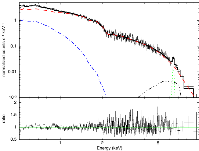
Figure 2. Same spectrum as Figure 1 but now includes a power law, disk blackbody, a narrow Fe K \alpha line, and a broad Fe K \alpha line, modeled with Xspec model phabs(po+diskbb+zgauss+laor)*zedge*zedge . We used the same Galactic absorption and absorption edges as in Figure 1. The power law is the red dashed line. The disk blackbody is the blue dot-dashed line. The narrow Fe K \alpha line is the green dotted line. The broad Fe K \alpha line is the black triple-dotted-dashed line. Finally, the solid black line is the sum of all the components. The fit produced a \chi^2/\nu = 368.0/353 .
