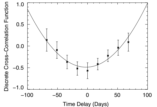
Figure 9. DCCF between X-ray and radio luminosities. We fit the DCCF with a quadratic function, and the minimum occurs at -2.5 \pm 5.3 days with a DCCF value of -0.48 \pm 0.1 . A negative delay implies that the radio is lagging the X-ray.
