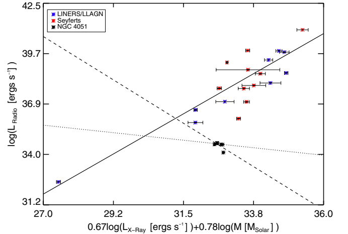
Figure 8. Projection of the fundamental plane of accretion onto black holes as described by Gültekin et al. (2009a). The red points are Seyfert galaxies, while blue points are LINERS or LLAGN. The solid black line is Gültekin et al. (2009a) best-fit line. Our data points are shown in black, with our best fit as the dashed line and dotted lines as described in Figure 7.
