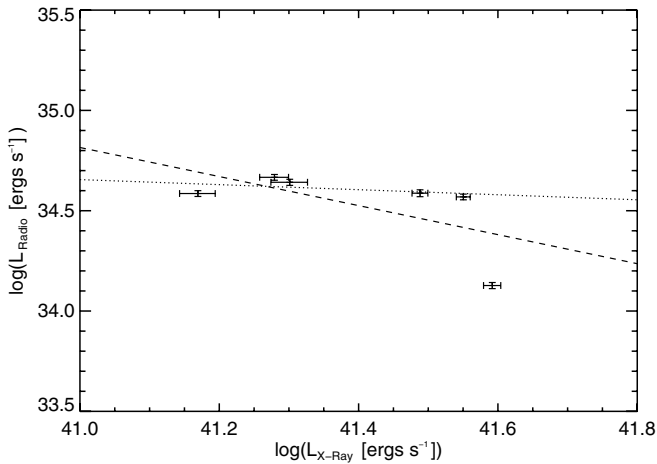
Figure 7. Inverse correlation between the X-ray and radio luminosities. We used the continuum flux from 2 to 10 keV, and we scaled the radio flux as F_\nu \propto \nu^{-0.5} (Ho 2002) from 8.4 GHz to 5 GHz in order to correctly compare to Gültekin et al. (2009a). The dashed line is a fit to our data given by the relation, \log L_{\text{radio}} = (-0.72 \pm 0.04) \log L_{X\text{-ray}} + (64 \pm 2) . The dotted line excludes the A configuration data point, and is described by the relation \log L_{\text{radio}} = (-0.12 \pm 0.05) \log L_{X\text{-ray}} + (40 \pm 2) .
