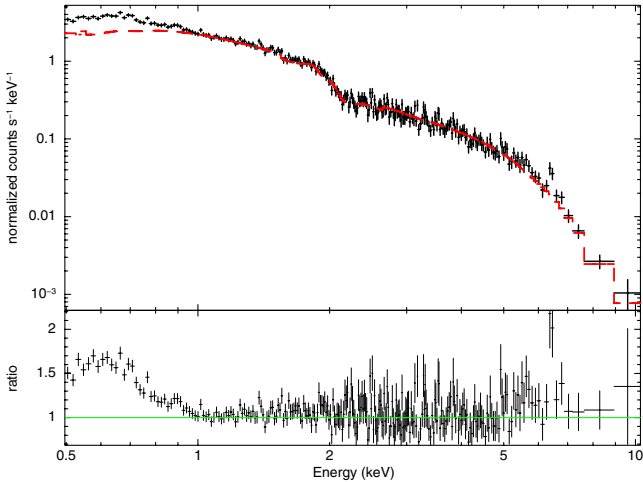
Figure 1. Sample spectrum from MJD 54943.1 modeled with just a power-law component, in red, as the Xspec model phabs(po)*zedge*zedge . The Galactic absorption was modeled as an effective H column density of 1.15 \times 10^{20} \text{ cm}^{-2} (Kalberla et al. 2005) and the K-shell absorption edges of O VII and O VIII were frozen at their respective rest energies of 0.739 keV and 0.871 keV. We initially fit the spectrum from 2 to 10 keV and then extended the model to lower energies. The fit produced a \chi^2/\nu = 1770/366 .
