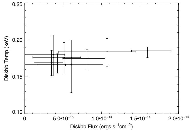
Figure 3. Comparison between the soft-excess disk blackbody temperature and its blackbody flux. A constant temperature independent of flux as seen here suggests a purely phenomenological interpretation of the disk blackbody component.
