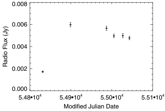
Figure 6. 8.4 GHz light curve taken by the VLA/EVLA. The radio flux density varies by more than a factor of three.
