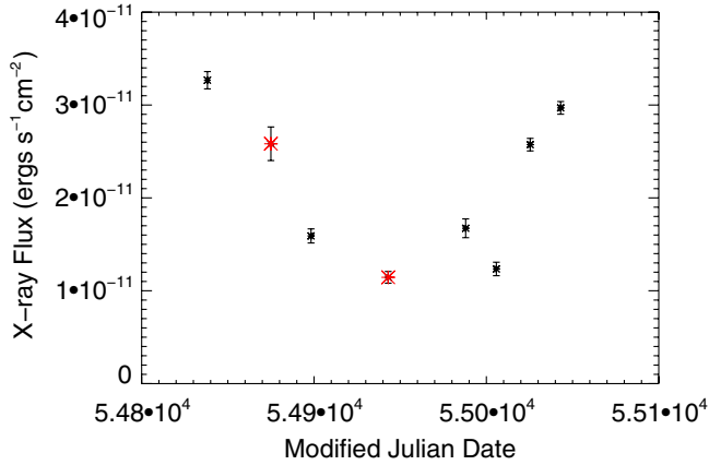
Figure 4. X-ray light curve taken by Chandra in the continuous clocking mode between 2 and 10 keV. It shows a variability of a factor of three. The points in red do not have simultaneous radio observations and are not used in the correlation analysis.
