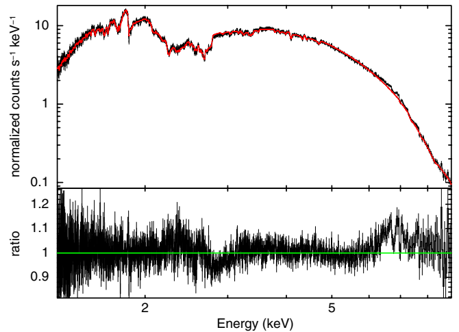
Figure 2. Time-averaged Chandra /HETGS spectrum of IGR J17480–2446, fitted with a simple blackbody plus power-law model. Note the broad Fe K emission line, and Fe xxv and Fe xxvi absorption lines in the data/model ratio. (A color version of this figure is available in the online journal.)
