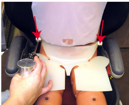
Figure 25 Checking that the X and Z values of the symmetrical points
