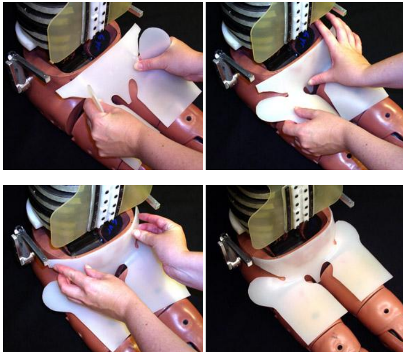
Figure 10. Attaching the lap form to the ATD
