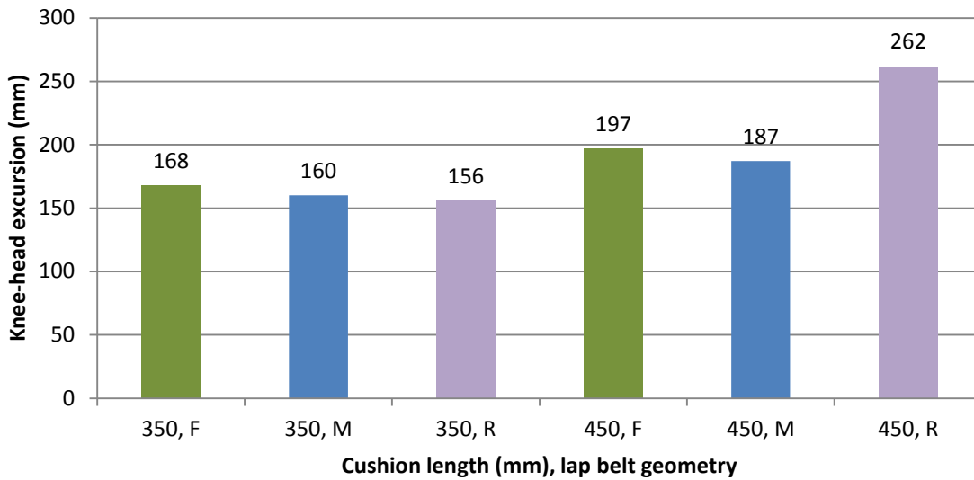
Figure 14. Knee-head excursion for 10YO ATD for each combination of cushion length (350 vs. 450) and lap belt anchorage location (F, M, R).
