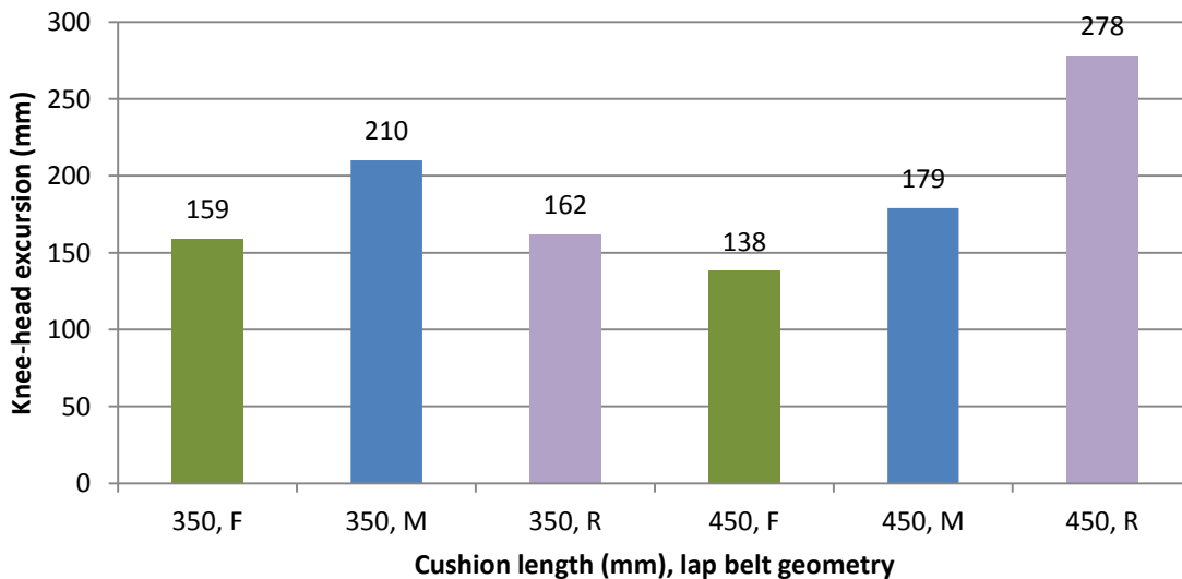
Figure 15. Knee-head excursion for 6YO ATD for each combination of cushion length (350 vs. 450) and lap belt anchorage location (F, M, R).
