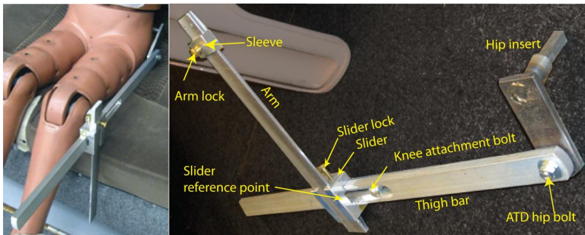
Figure 2. Example of a cushion length tool for six year-old ATD.
