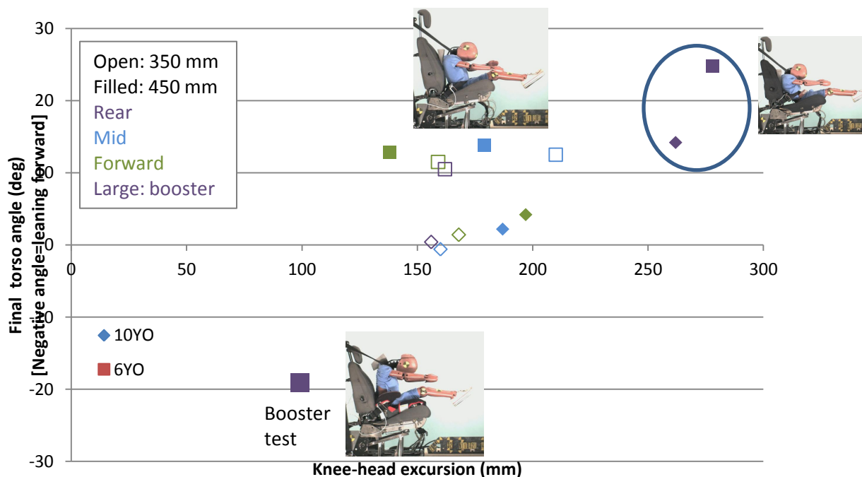
Figure 16. Peak torso angle vs. knee-head excursion for all tests. [Tests with clear submarining circled.]
