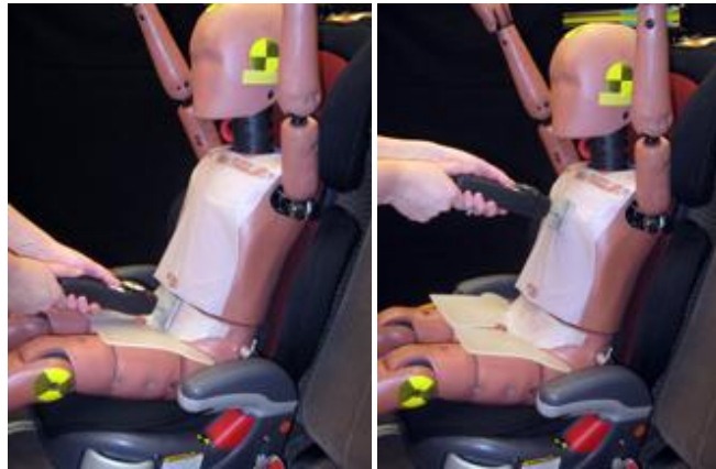
Figure 28. Applying 177 N of force to the pelvis and thorax of the ATD.
