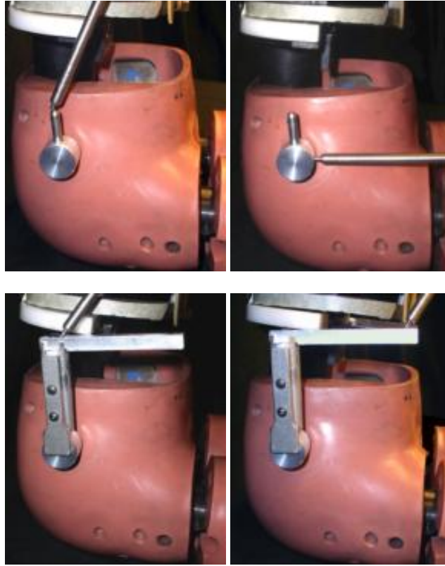
Figure 8. Digitizing the reference marks on the hip offset tools with the upright attachment on and off.
