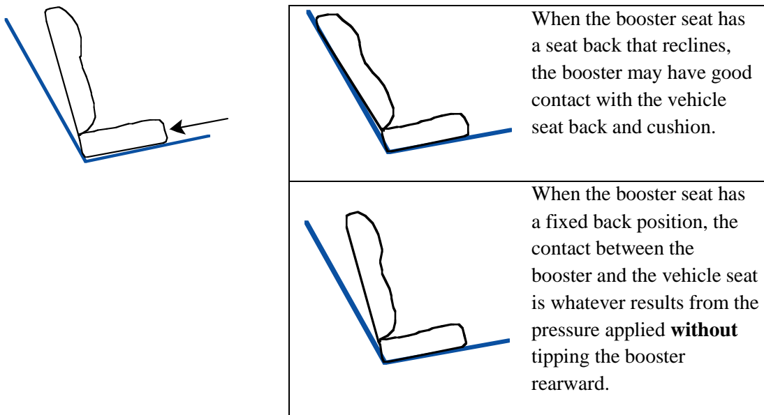
Figure D2. Apply 30 lb force to the front of the booster seat cushion. When the vehicle seat back is very reclined and/or the vehicle cushion very flat, boosters with a fixed back angle may not conform to the vehicle seat as much as boosters with seat backs that recline.
