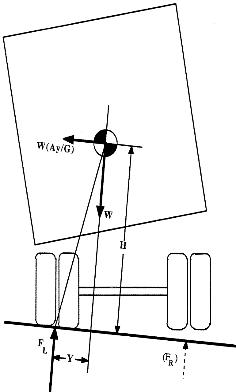
Figure 2.3.2.a Performance Measure b(1) - Dynamic Roll Stability
