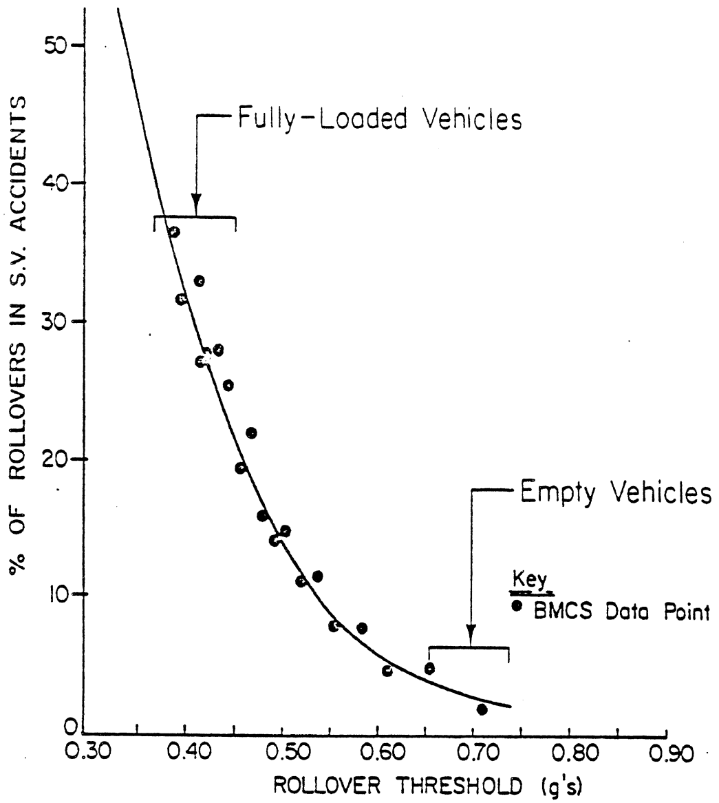
FIGURE 4.1.a Plot of rollover accident data versus calculated value of rollover threshold.
