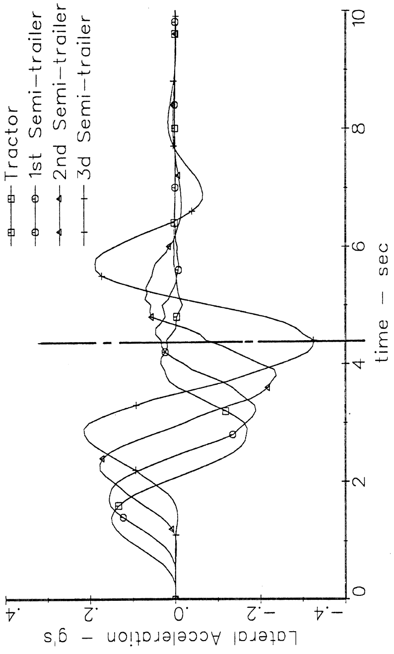
RTAC 8 axle C-train Triples (55t/121k GCW), conf. 4.1, var. 1.00
