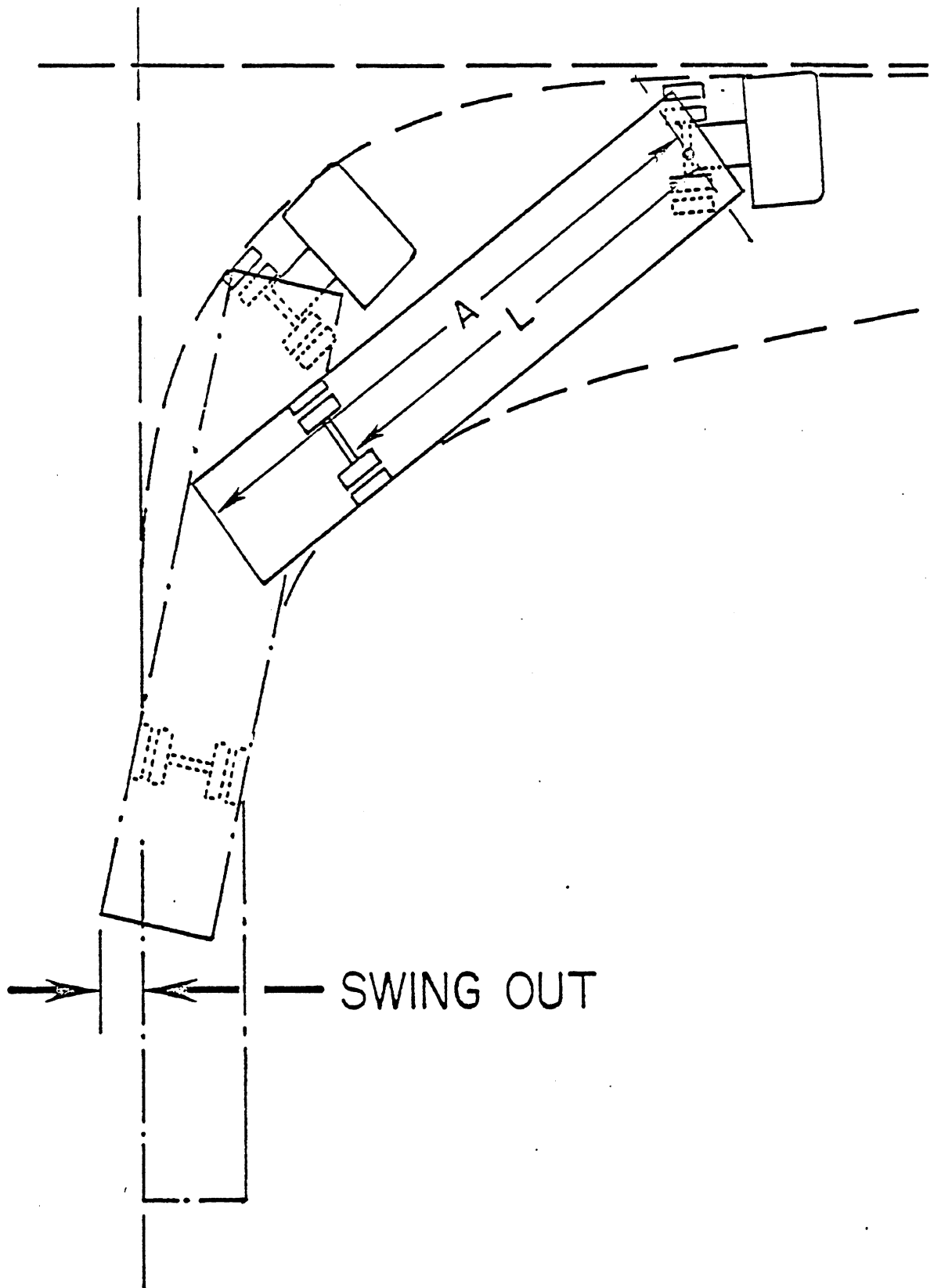
FIGURE 4.6.a The swing-out phenomenon occurring in a low-speed turn with a semitrailer having a relatively high value of A/L .
