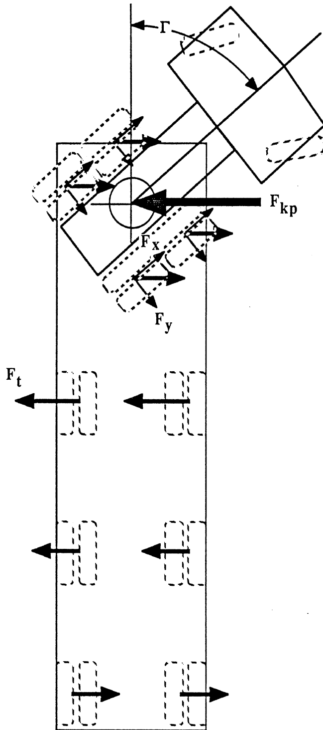
Figure 2.3.2.b Performance Measure c(2) - Tight Turn Jackknife Resistance
