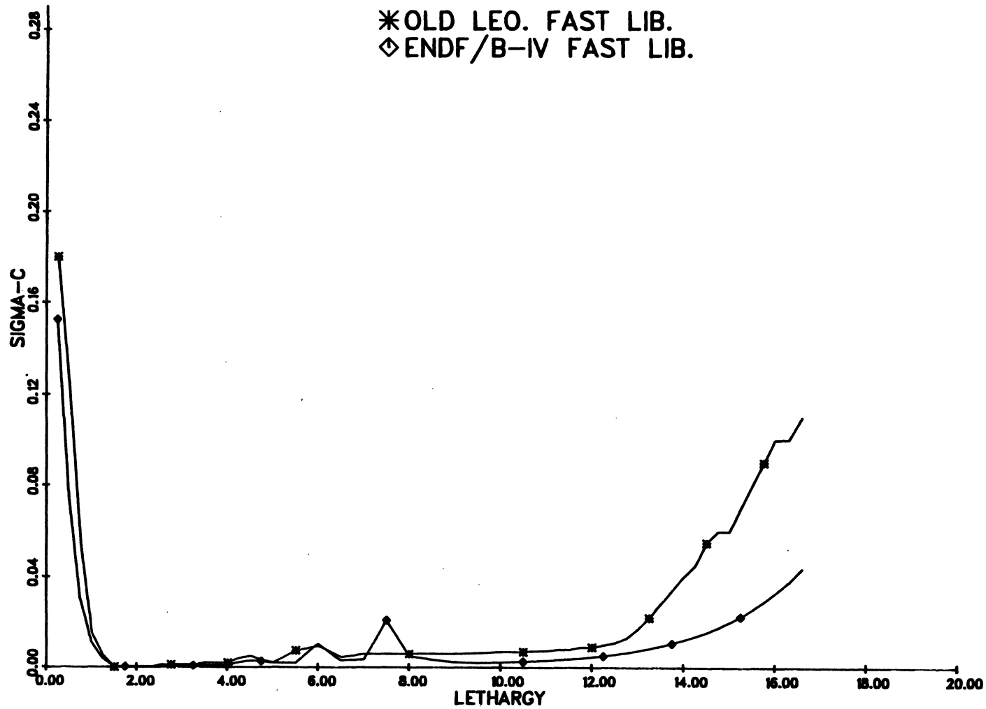
Figure 3. LEOPARD Library Comparison: 27 Al Capture Cross-Section vs. Lethargy
