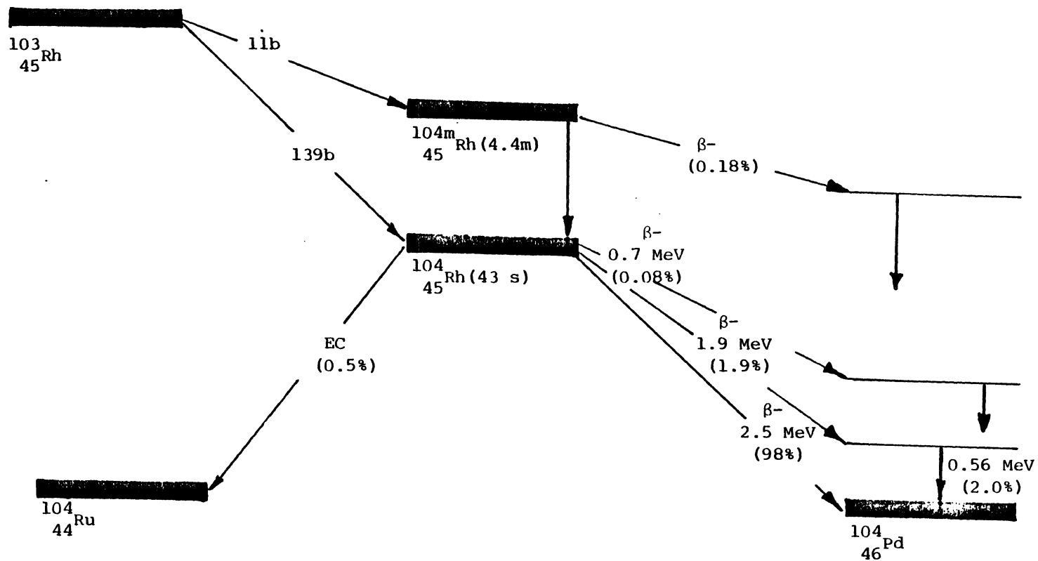
Figure 6. Rhodium Decay Scheme
