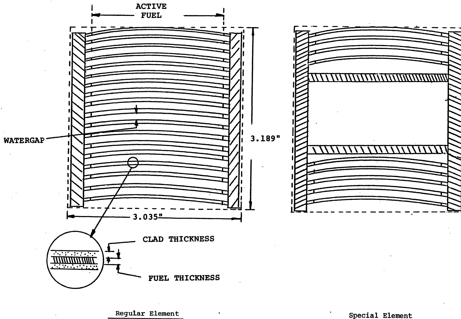
Fig. C-13. FNR Fuel Element Schematics
