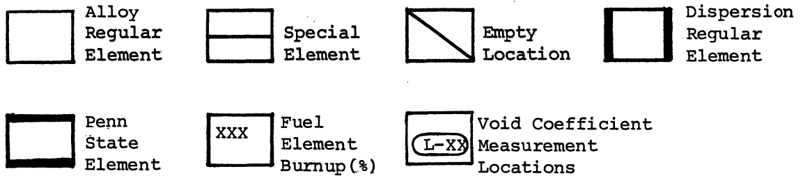
Figure 9. Core Configuration for Void Coefficient of Reactivity Experiment
