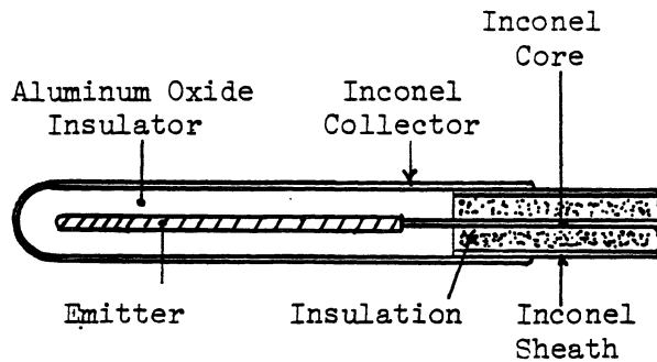
Figure 8. SPND Construction
