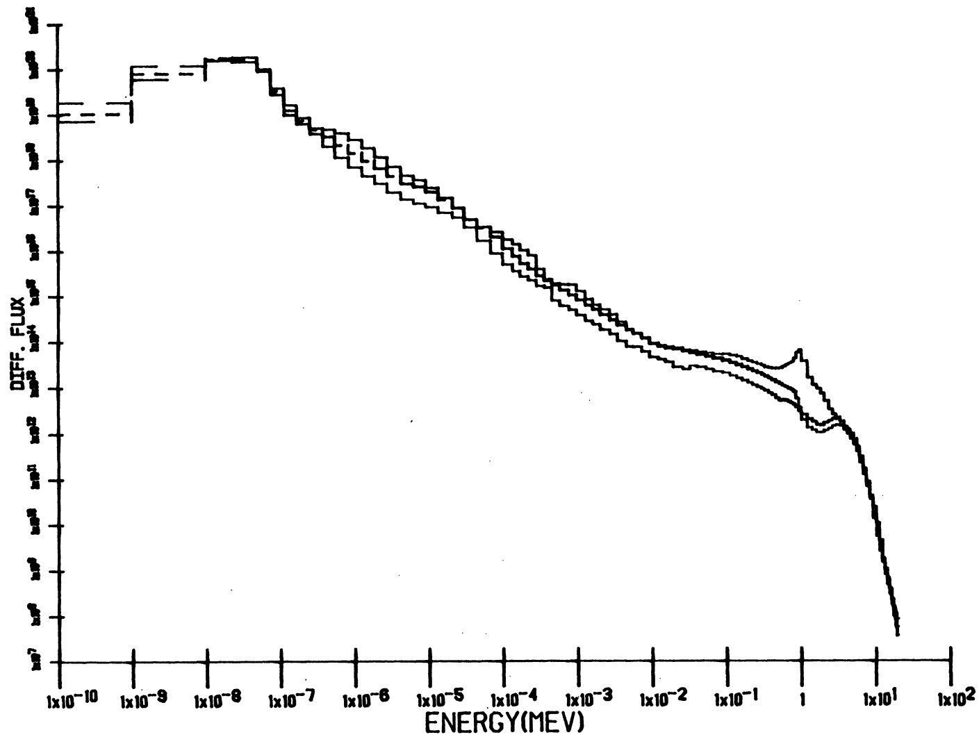
Figure 18. Unfolded in-core flux spectrum using five trial foils, along with upper and lower bounds on the solution.
