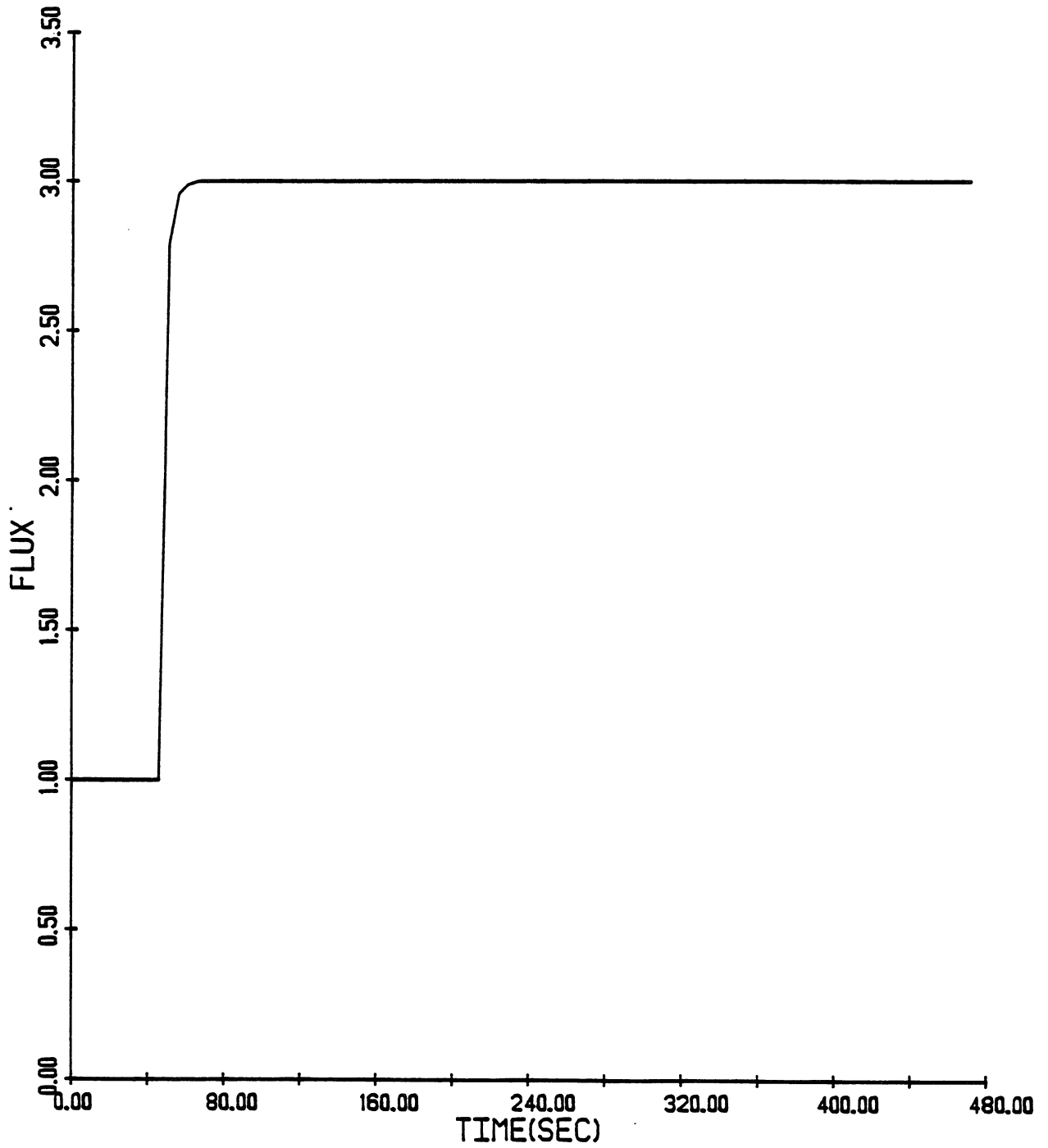
Figure 15. Code response to input data from Figure 14.
