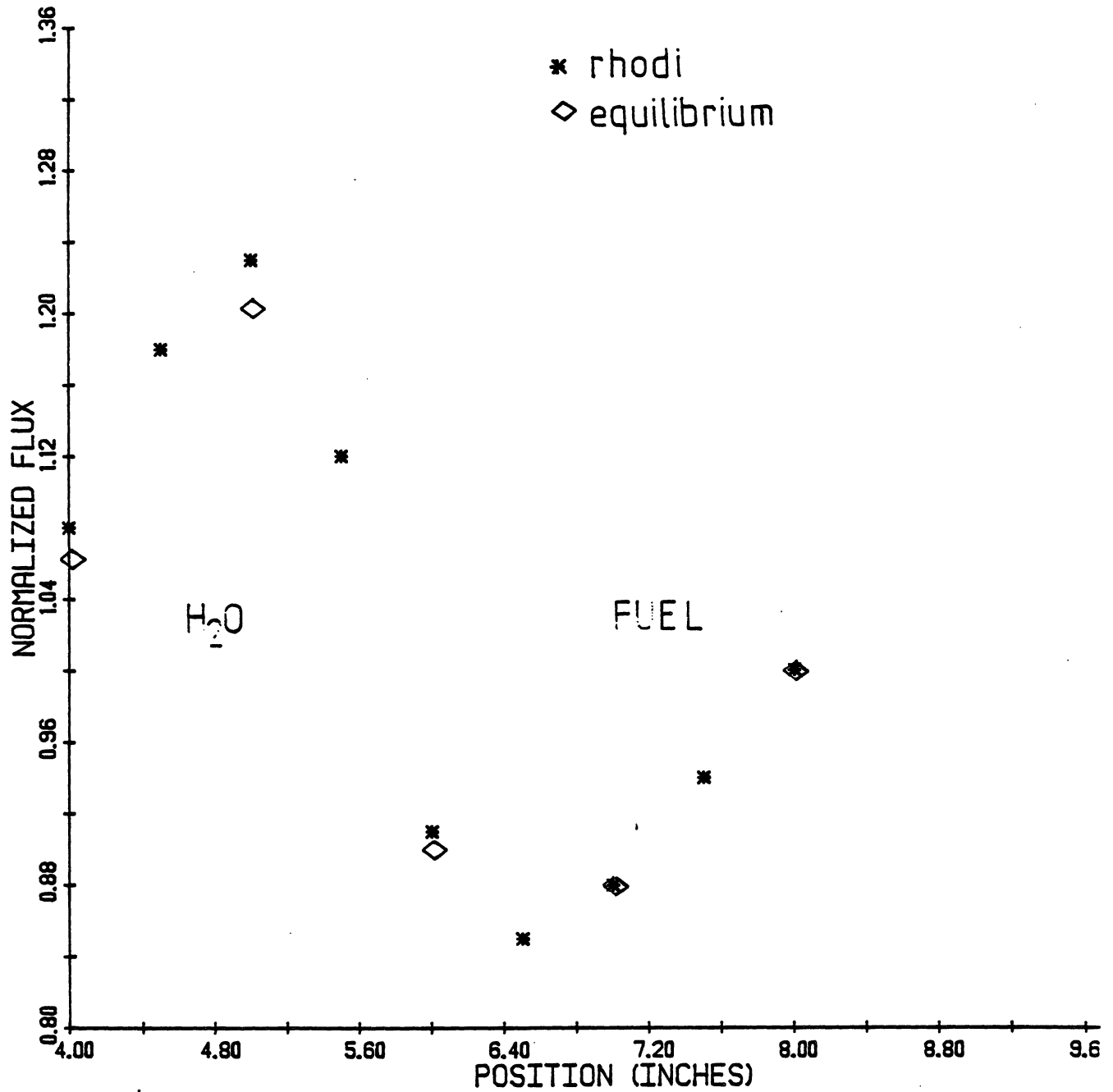
Figure 17. RHODI code response to data taken axially in H 2 O reflector below L-37 is compared to equilibrium data.
