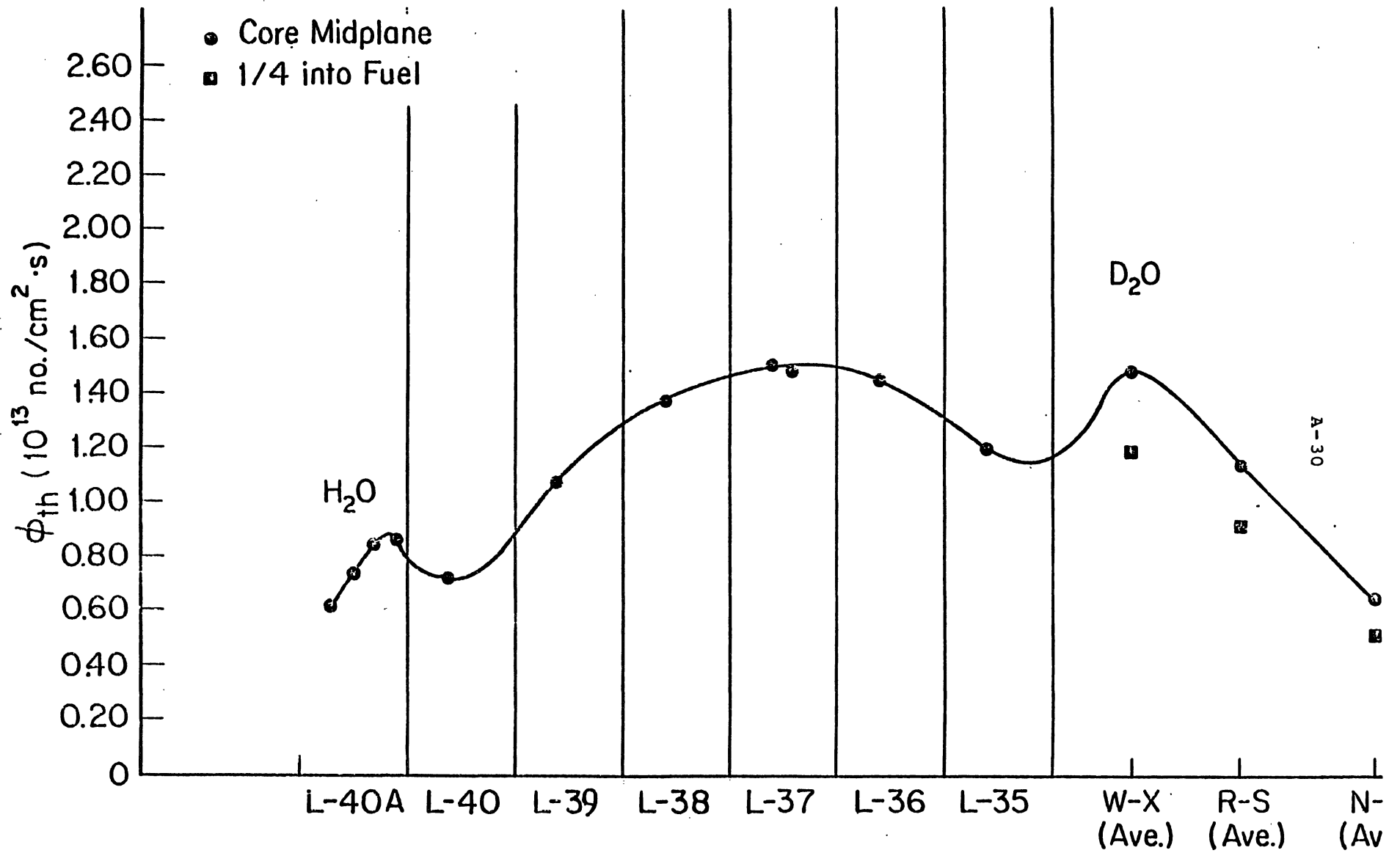
Figure 13. North-South Traverse Through L-37 Map #2
