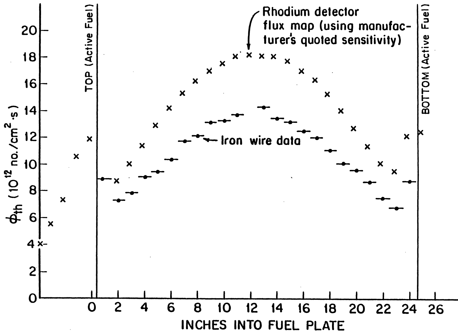
Figure 2. Wire Activation Results for \phi_{th} + \phi_{IT} -Location L-37-
