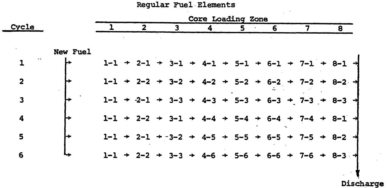
Figure 4. Equilibrium Core Shuffling Scheme
