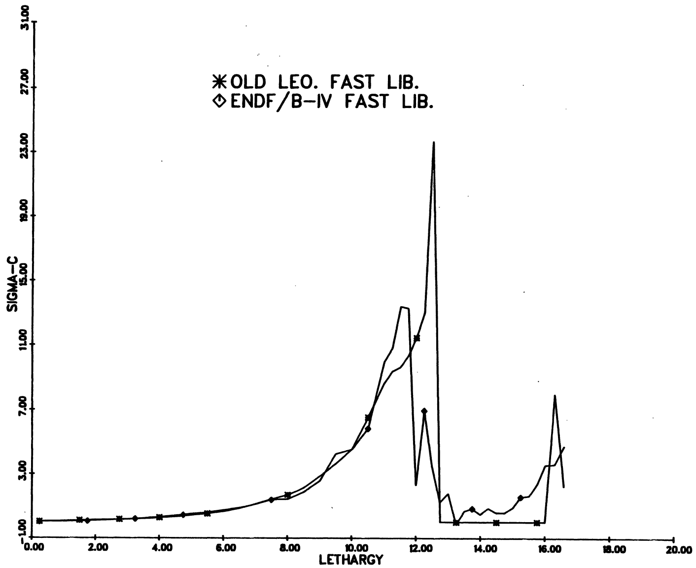
Figure 1. LEOPARD Library Comparison: ^{235}\text{U} Capture Cross-Section vs. Lethargy
