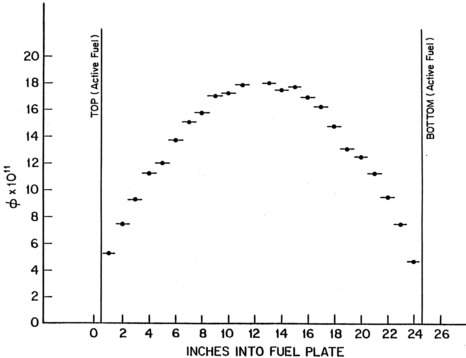
Figure 3. . Wire Activation Results for \phi_F -Location L-37-
