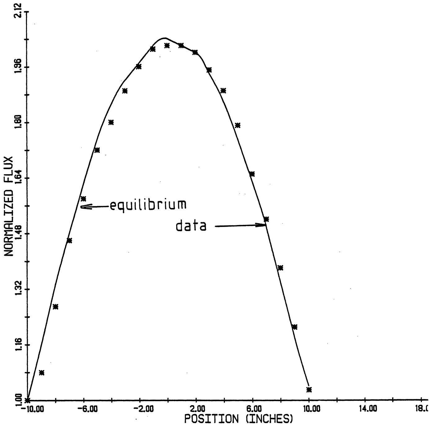
Figure 16. Equilibrium data compared to code response for data taken axially at 1"/minute through the center 21" of L-37.
