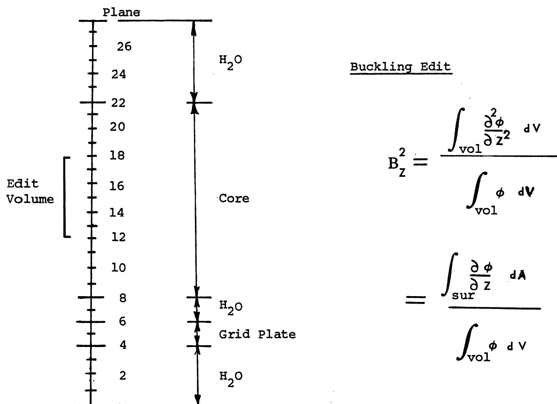
Figure 8. Axial Geometry for 3-Dimensional VENTURE Calculation
