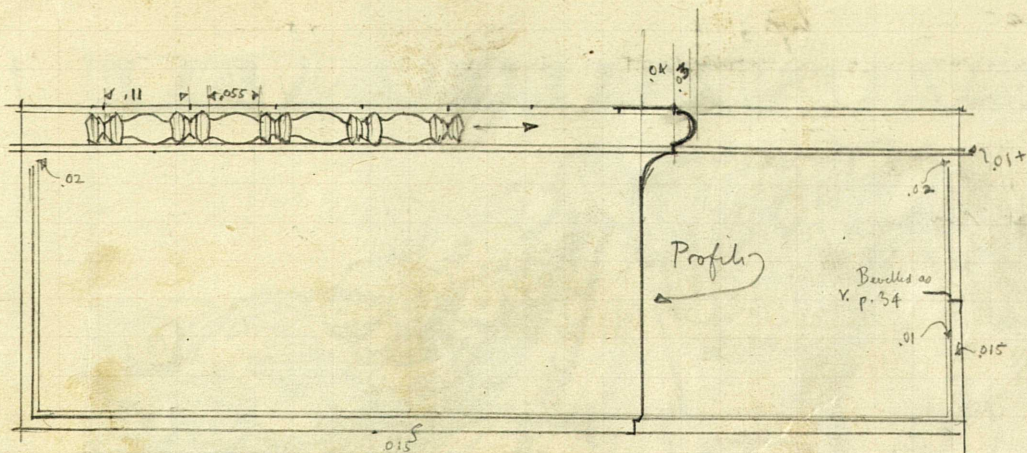
Top Block of Cella wall with Tetragal
