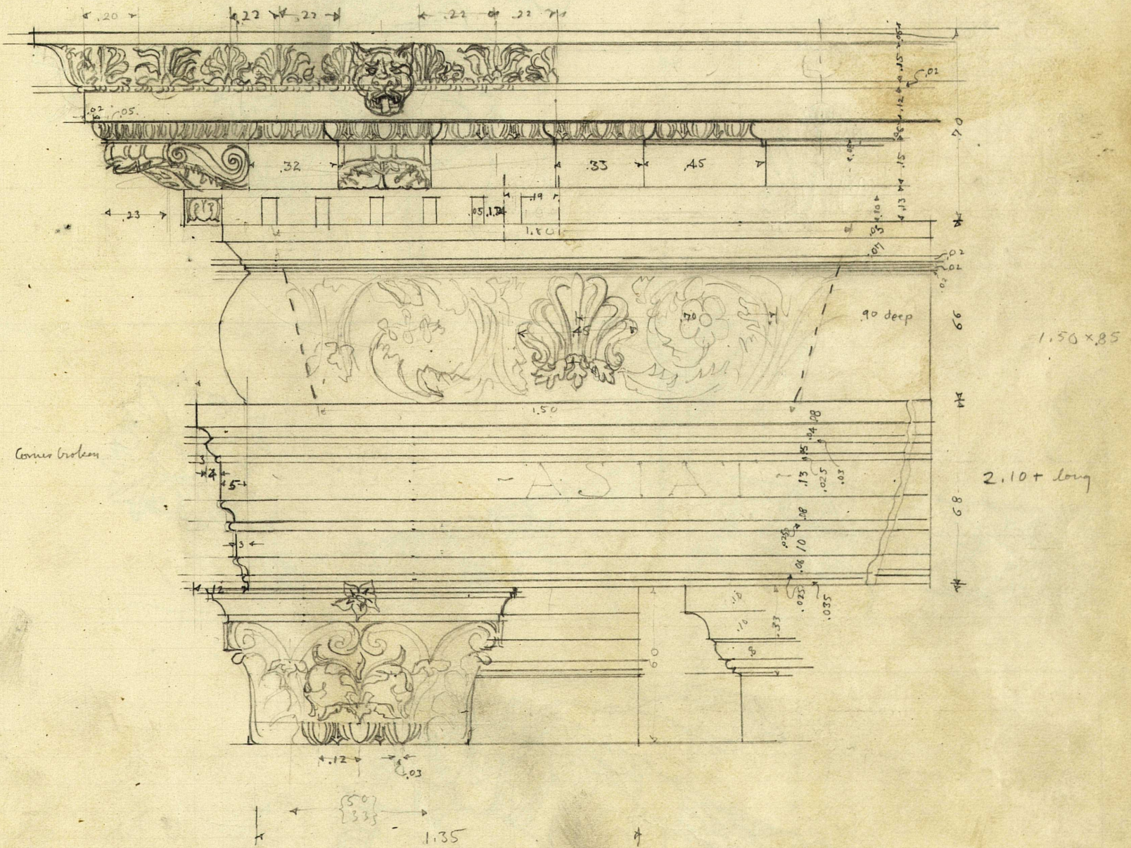
Main Entablature and Cap of Pier
