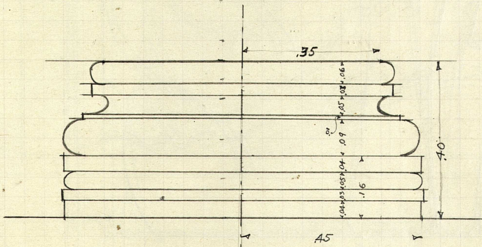
- Base of Cipolino(?) Marble -
