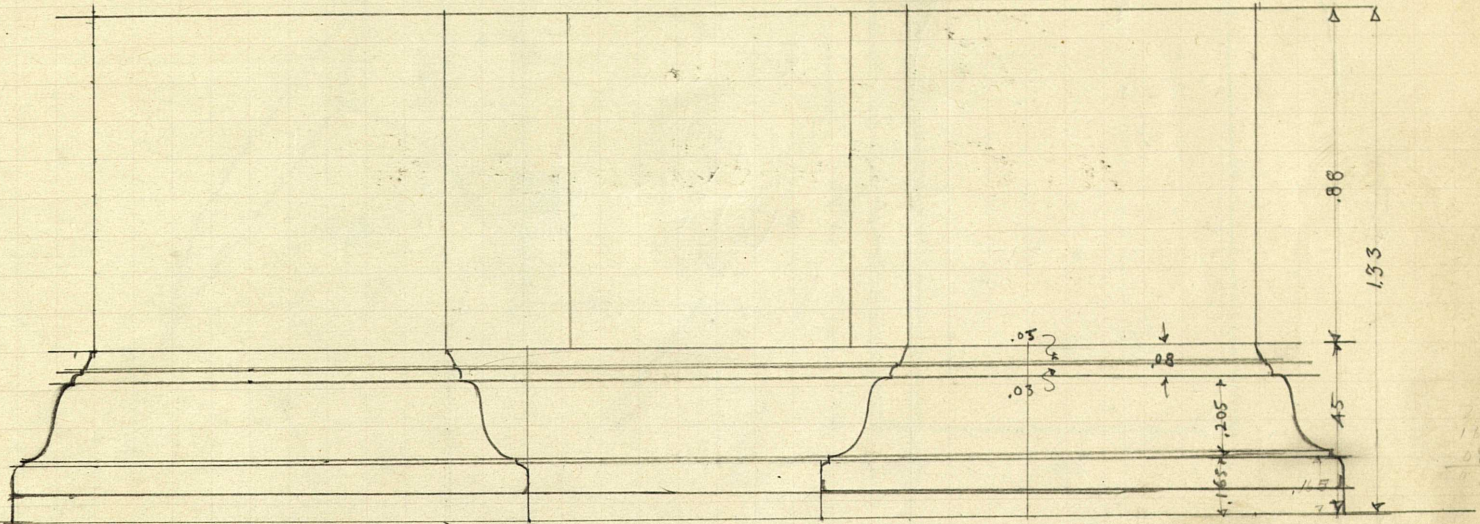
Elevation of Long Side of Base
