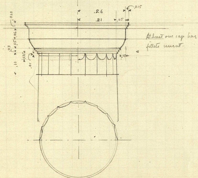
Details of the Doric Order
