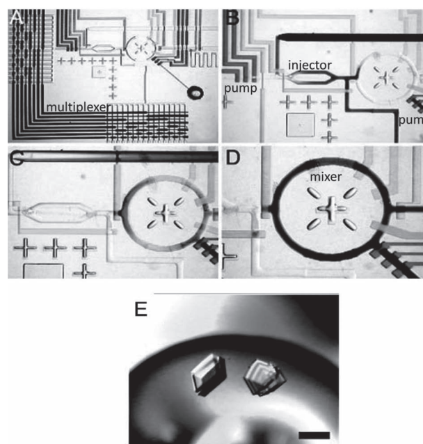
Figure 5. Applications of microfluidic multiplexers. A–D) Optical micrographs of “Formulation chip”. E) Large, single, 3D crystals grown directly from optimal screen. A–E, reproduced with permission. [37] Copyright 2004, National Academy of Sciences, USA.
