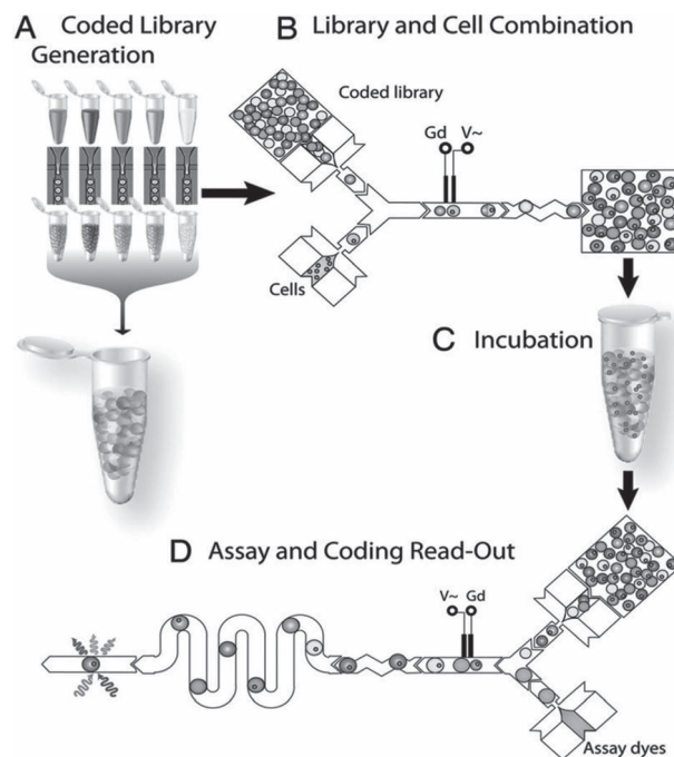
Figure 7. Droplet microfluidic application flowchart. A) Cell stimulants are encapsulated into droplets and stored off chip. B) Stimulants are mixed together or with single-cell encapsulated droplets via fusion operations. C) After fusion, the droplets can then be recollected and incubated off chip if necessary. D) Droplets are once again loaded into a droplet device with fusion operations with separate reagents for protein assay. Fluorescence signals can then be acquired downstream after chaotic advection mixing to determine effects of stimulants on single cells. Reproduced. [64]
