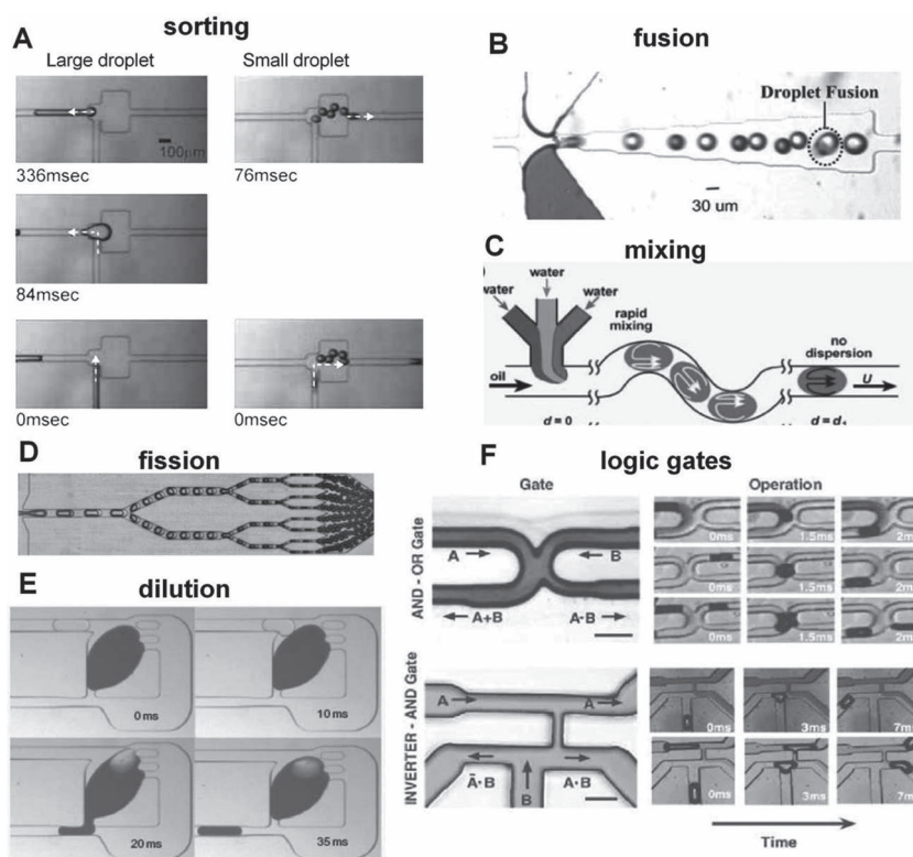
Figure 6. Droplet microfluidic operations. A) Sorting by size. Reproduced with permission. [49] Copyright 2008, Springer. B) Spontaneous fusion. Reproduced with permission. [55] Copyright 2006, Royal Society of Chemistry. C) Mixing by chaotic advection. Reproduced. [56] D) Droplet fission. Reproduced with permission. [58] Copyright 2011, Royal Society of Chemistry. E) Dilution. Reproduced with permission. [61] Copyright 2011, Nature Publishing Group. F) Microfluidic analogues of electric logic gates. Reproduced with permission. [62] Copyright 2007, American Association for the Advancement of Science.
