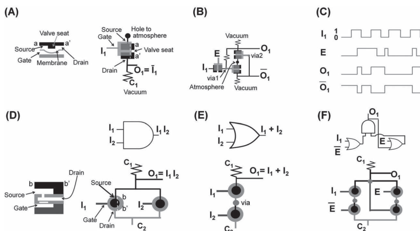
Figure 3. Microfluidic logic gates. A) Pneumatic NOT gate. Cross-section of a valve shows the valve-on state; source and drain terminals are in the top channel; and a gate terminal locates at the bottom channel under the membrane. In the top view of the valve, black area is in top channel and gray area is in bottom channel. B) Pneumatic gated D latch consisting of NOT gates. C) State of each line in gated D latch. Vacuum and atmospheric pressure are defined as state 1 and 0, respectively. D) Hydraulic AND gate. Cross-section shows a normally open valve, which has a pressure gain with a rigid disk (white bar above gate in left panel); valve is off when gate pressure is sufficiently high to deflect the membrane containing the disk upward and to close a hole. In the top view of the valves, black, light gray, and dark gray areas are in the top, middle, and bottom channels, respectively. E) Hydraulic OR gate. F) Hydraulic static latch consisting of AND and OR gates. State of each line coincides that in (C). Note that high and low pressures are defined as state 1 and 0, respectively, and it is the opposite of pneumatic logic.
