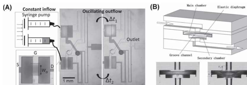
Figure 4. Constant-input-driven microfluidic oscillator. A) Constant-flow-driven oscillator. In the two normally closed valves, one valve's drain is connected to the other valve's gate, thereby making alternating pressure accumulation and release of each valve. Reproduced with permission. [30] Copyright 2012, American Chemical Society. B) Constant-pressure-driven oscillators. Vibration of free-standing, flexible disk results in outflow oscillation. Reproduced with permission. [31] Copyright 2012, Royal Society of Chemistry.
